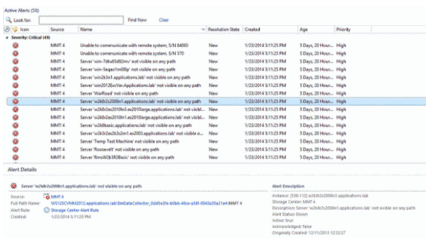
Figure 14. SCOM Active Alerts Pane
