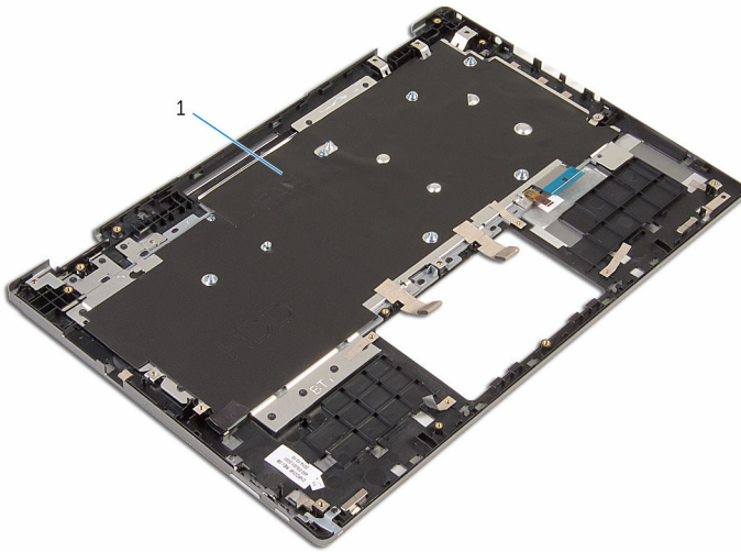
1 palmrest and keyboard assembly
