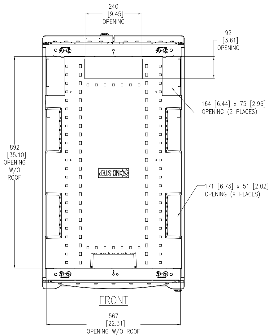
TOP VIEW CABLE OPENINGS (COVERS REMOVED)
