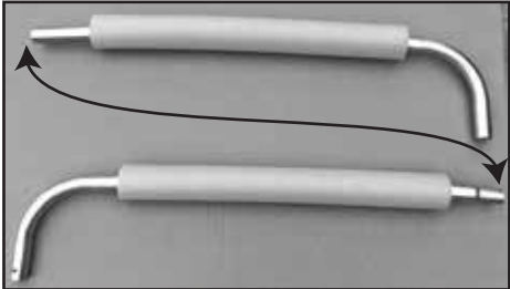
Slide foam (V) over the left and right curved arch tubes (T, U). Connect a left arch tube (T) and a right arch tube (U). To connect parts, simply slide the section of tubing that is smaller on one end into the adjacent tube.
