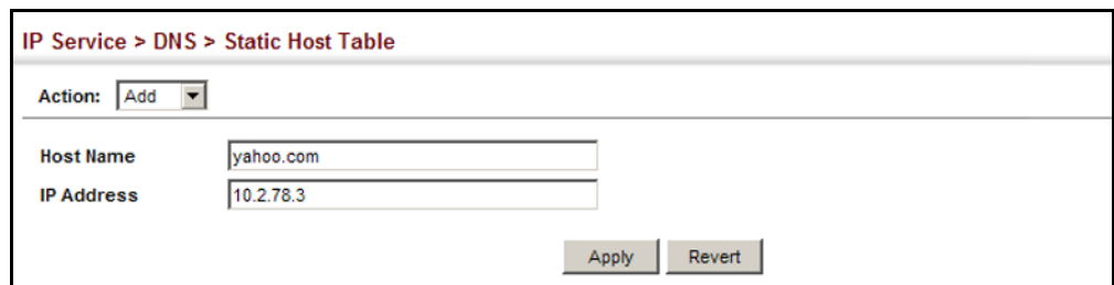
Figure 422: Configuring Static Entries in the DNS Table
