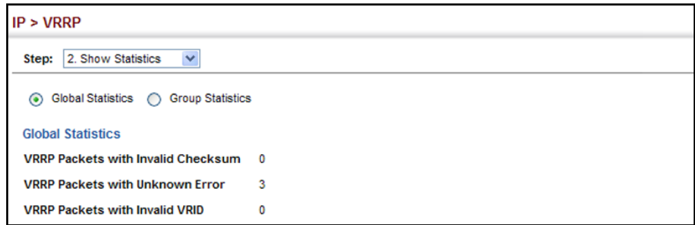
Figure 465: Showing Counters for Errors Found in VRRP Packets
