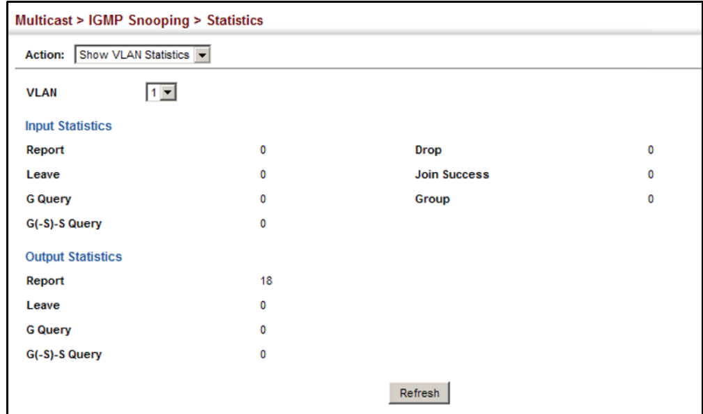
Figure 352: Displaying IGMP Snooping Statistics – VLAN
