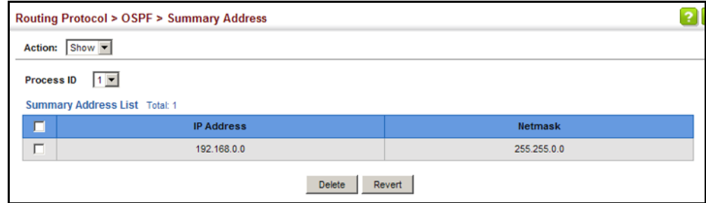
Figure 507: Showing Summary Addresses for External Routes
