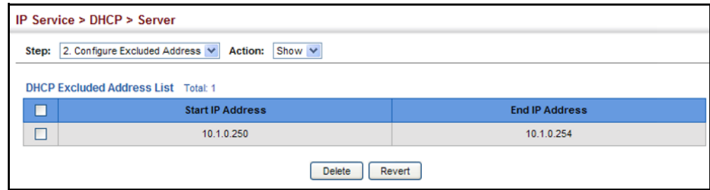
Figure 431: Showing Excluded Addresses on the DHCP Server
