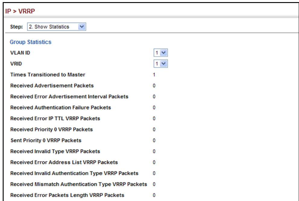
Figure 466: Showing Counters for Errors Found in a VRRP Group
