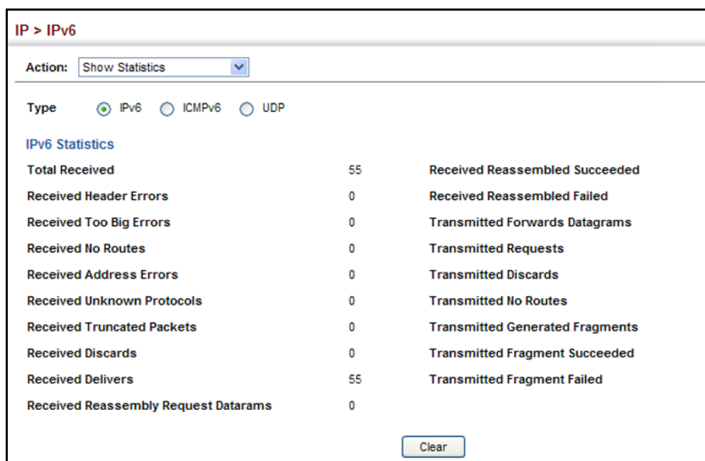
Figure 413: Showing IPv6 Statistics (IPv6)
