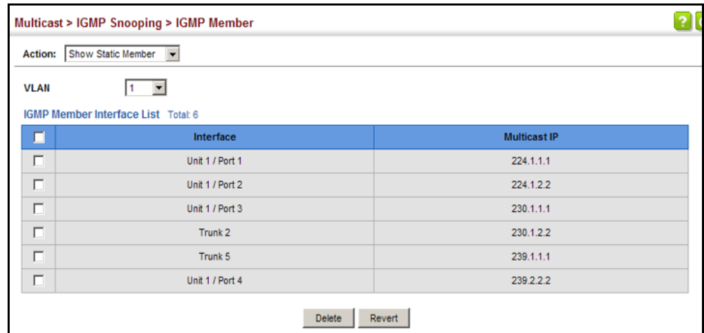
Figure 345: Showing Static Interfaces Assigned to a Multicast Service
