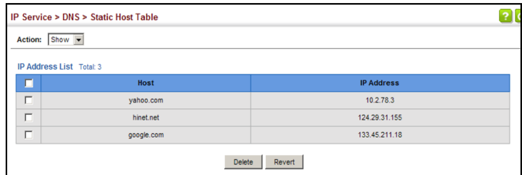
Figure 423: Showing Static Entries in the DNS Table
