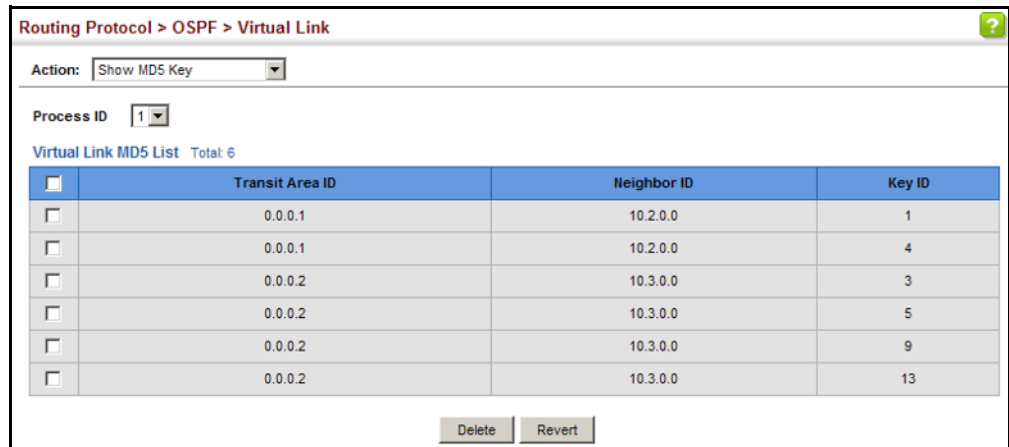
Figure 516: Showing MD5 Authentication Keys
