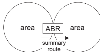
Figure 500: Route Summarization for ABRs
