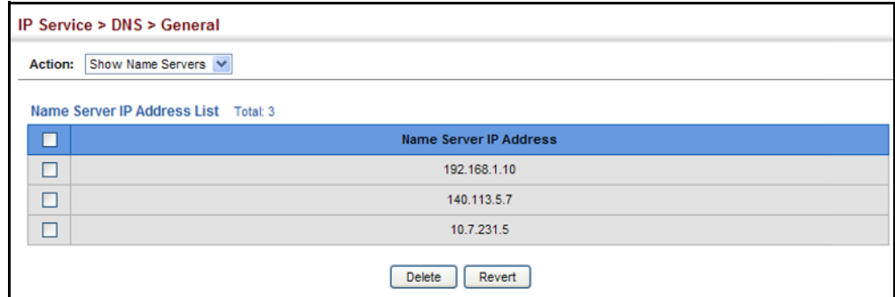
Figure 421: Showing the List of Name Servers for DNS
