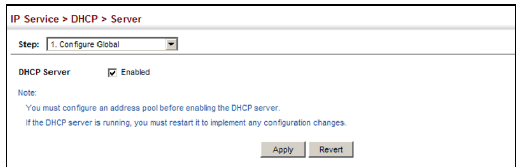
Figure 429: Enabling the DHCP Server
