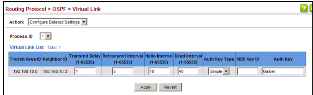
Figure 515: Configuring Detailed Settings for a Virtual Link
