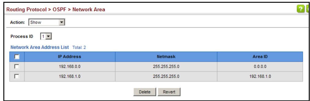
Figure 488: Showing OSPF Network Areas
