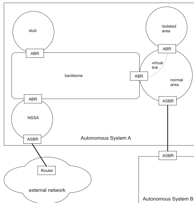
Figure 485: Configuring OSPF
