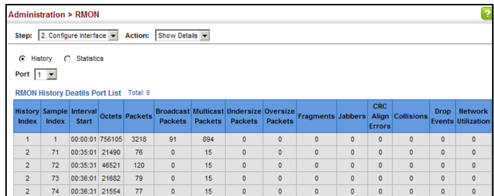
Figure 285: Showing Collected RMON History Samples
