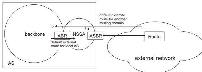
Figure 495: OSPF NSSA
