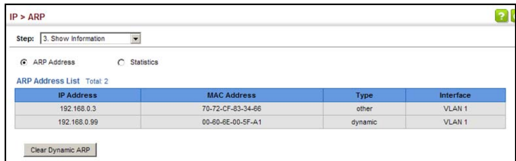
Figure 451: Displaying ARP Entries
