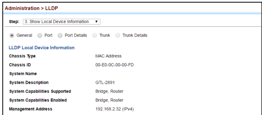
Figure 247: Displaying Local Device Information for LLDP (General)
