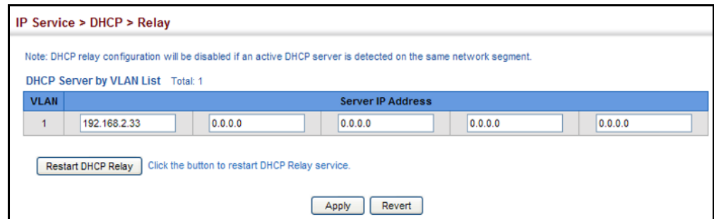
Figure 427: Configuring DHCP Relay Service
