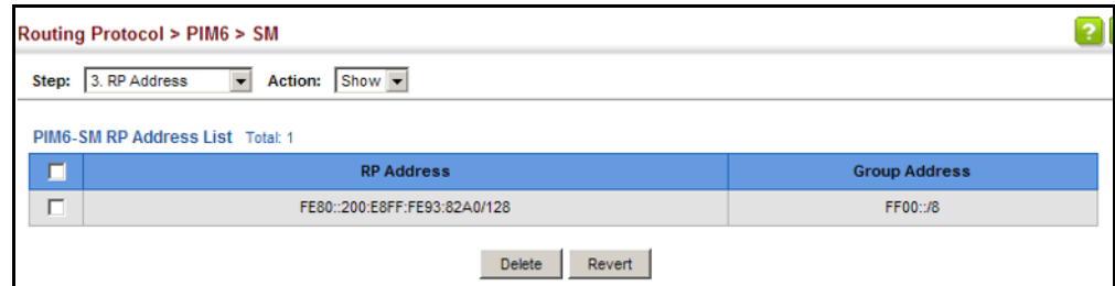
Figure 544: Showing PIM6 Static Rendezvous Points
