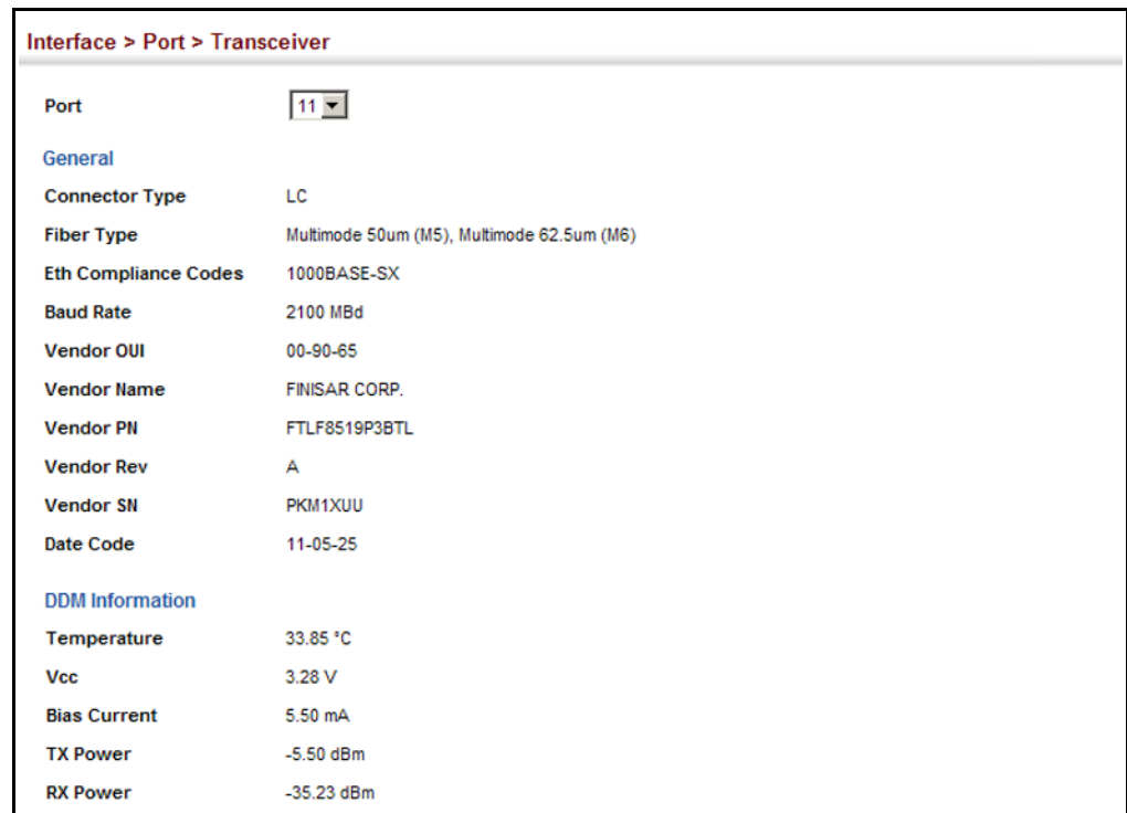
Figure 45: Displaying Transceiver Data
