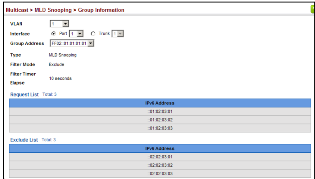
Figure 367: Showing IPv6 Multicast Services and Corresponding Sources
