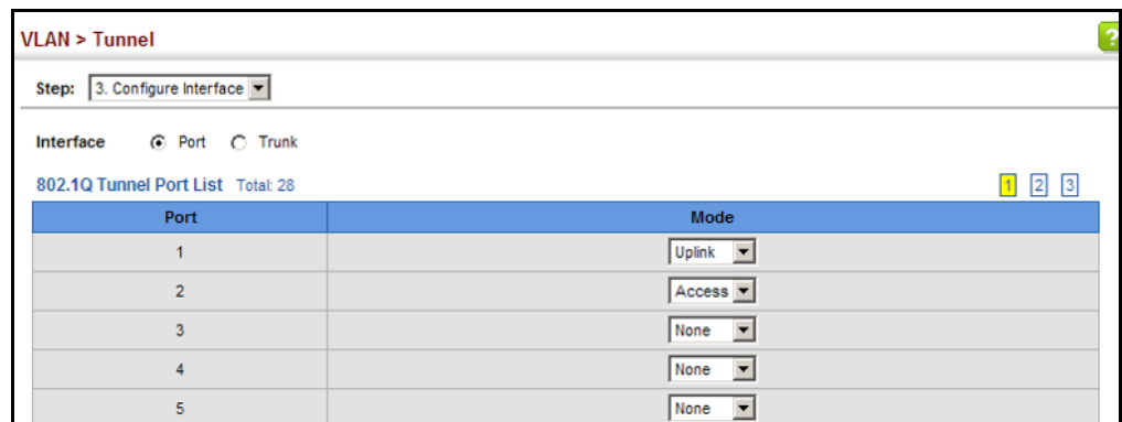
Figure 86: Adding an Interface to a QinQ Tunnel
