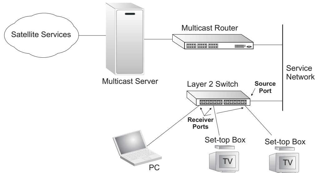
Figure 368: MVR Concept
