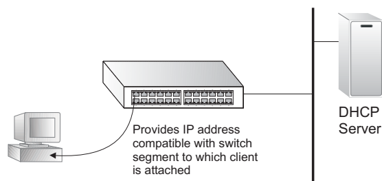
Figure 417: Layer 3 DHCP Relay Service
