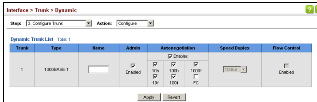
Figure 58: Configuring Connection Settings for a Dynamic Trunk
