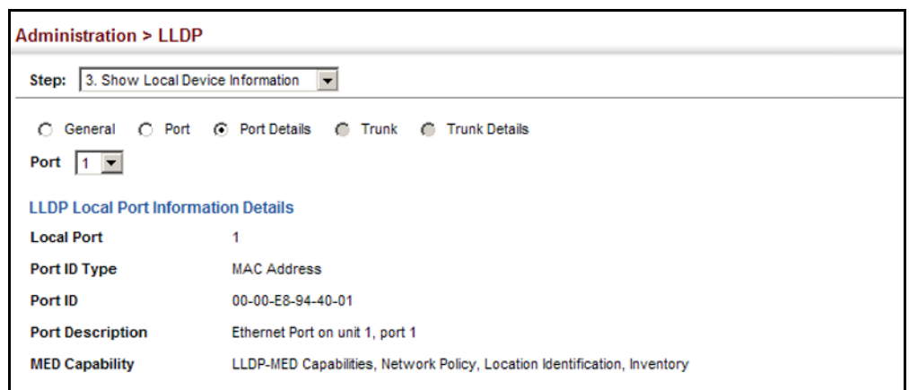
Figure 249: Displaying Local Device Information for LLDP (Port Details)
