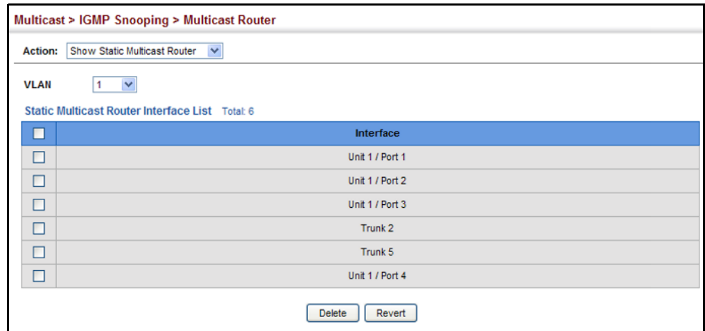
Figure 341: Showing Static Interfaces Attached a Multicast Router
