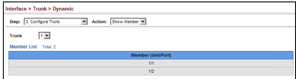
Figure 57: Showing Members of a Dynamic Trunk
