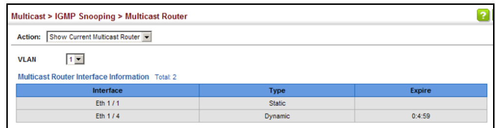
Figure 342: Showing Current Interfaces Attached a Multicast Router
