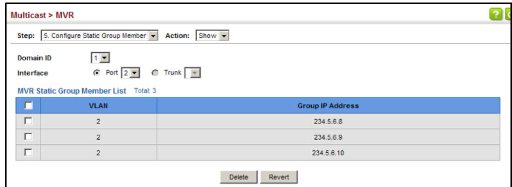
Figure 377: Showing the Static MVR Groups Assigned to a Port
