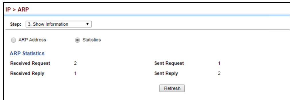
Figure 430: Displaying ARP Statistics
