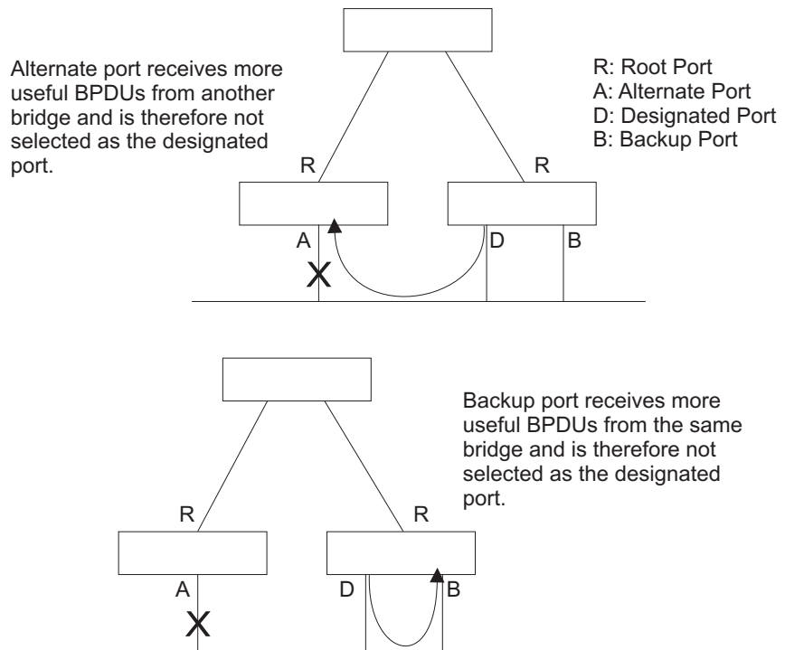
Figure 120: STA Port Roles
