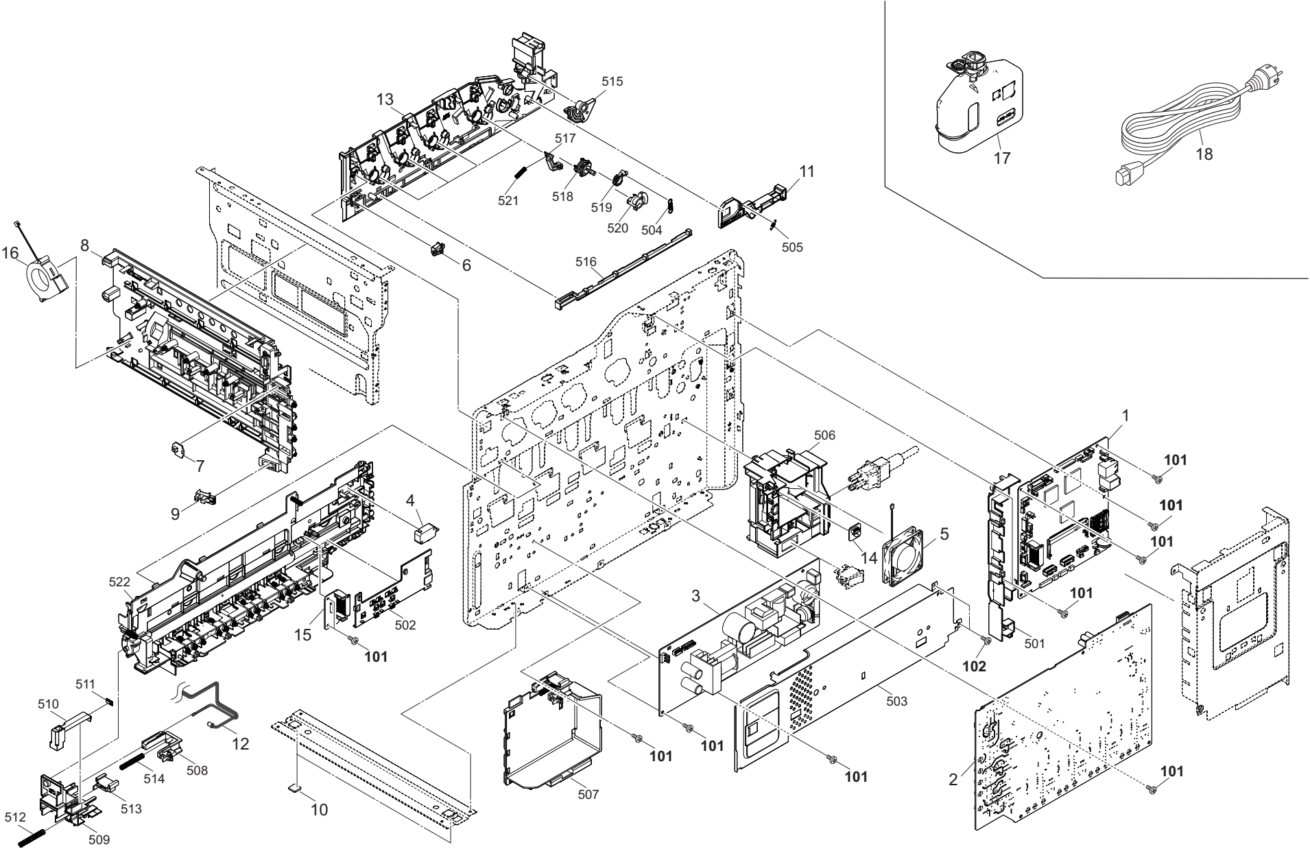
FIG. 14 Electrical Components 2
