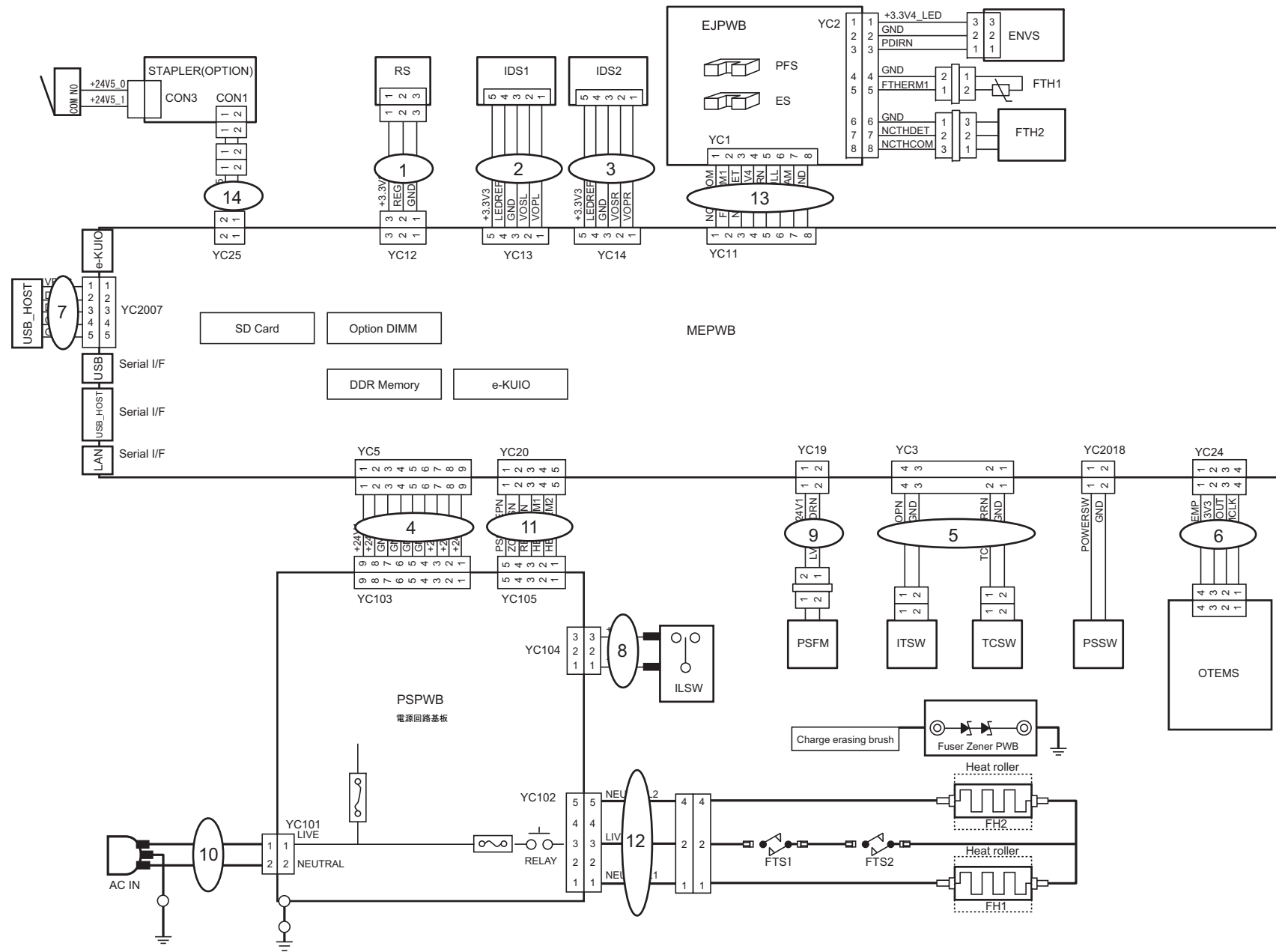
FIG. 19 Wire Section 1 2VM
