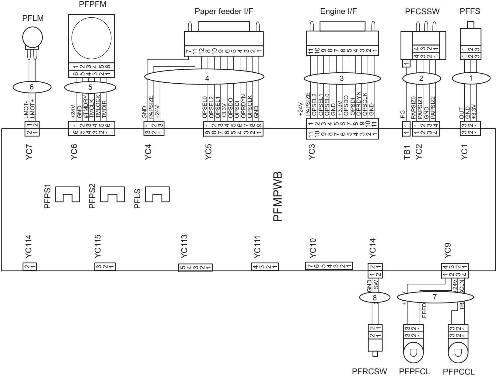
FIG. 3 Wire Section
