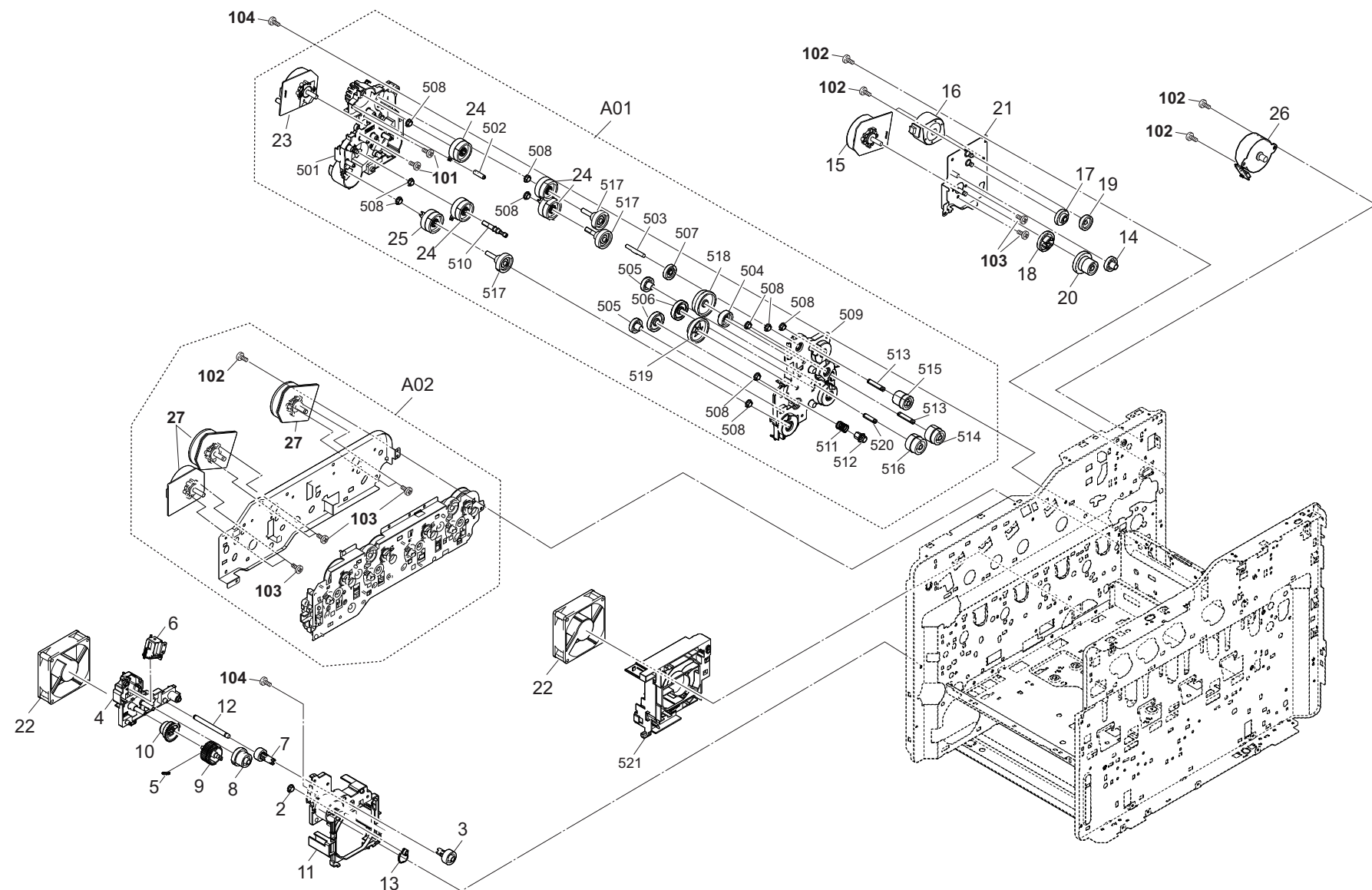
FIG. 12 Drive Section
