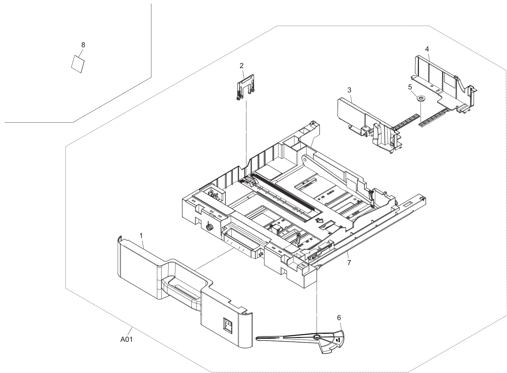
FIG. 4 Paper Cassette
