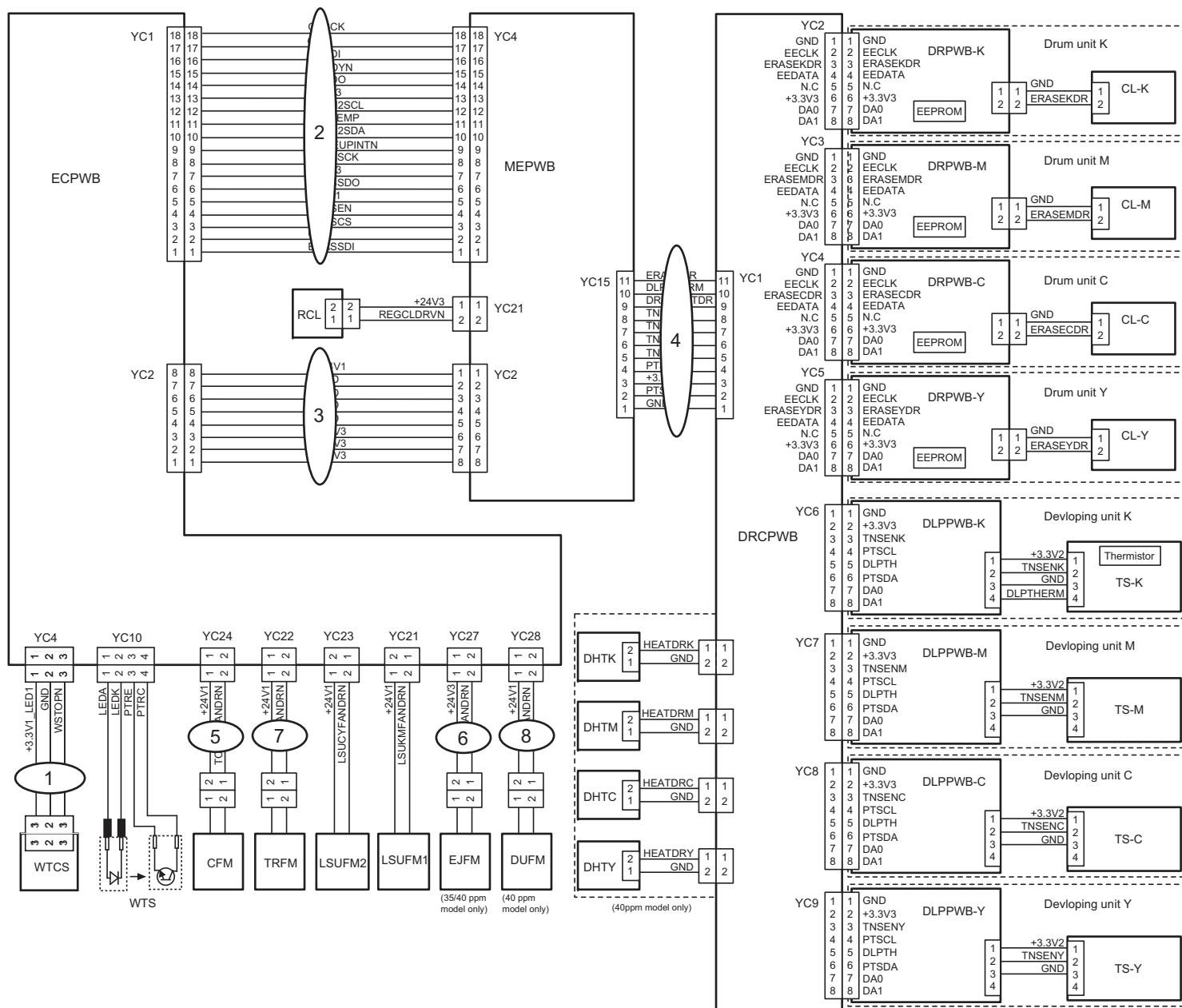
FIG. 18 Wire Section 3
