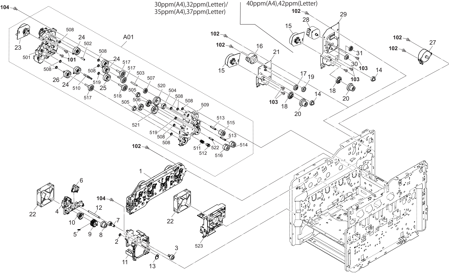
FIG. 12 Drive Section
