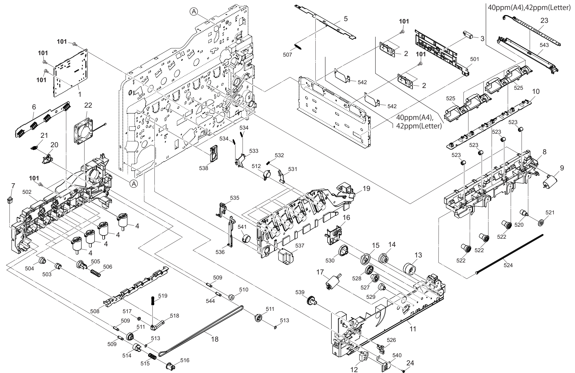
FIG. 13 Electrical Components 1
