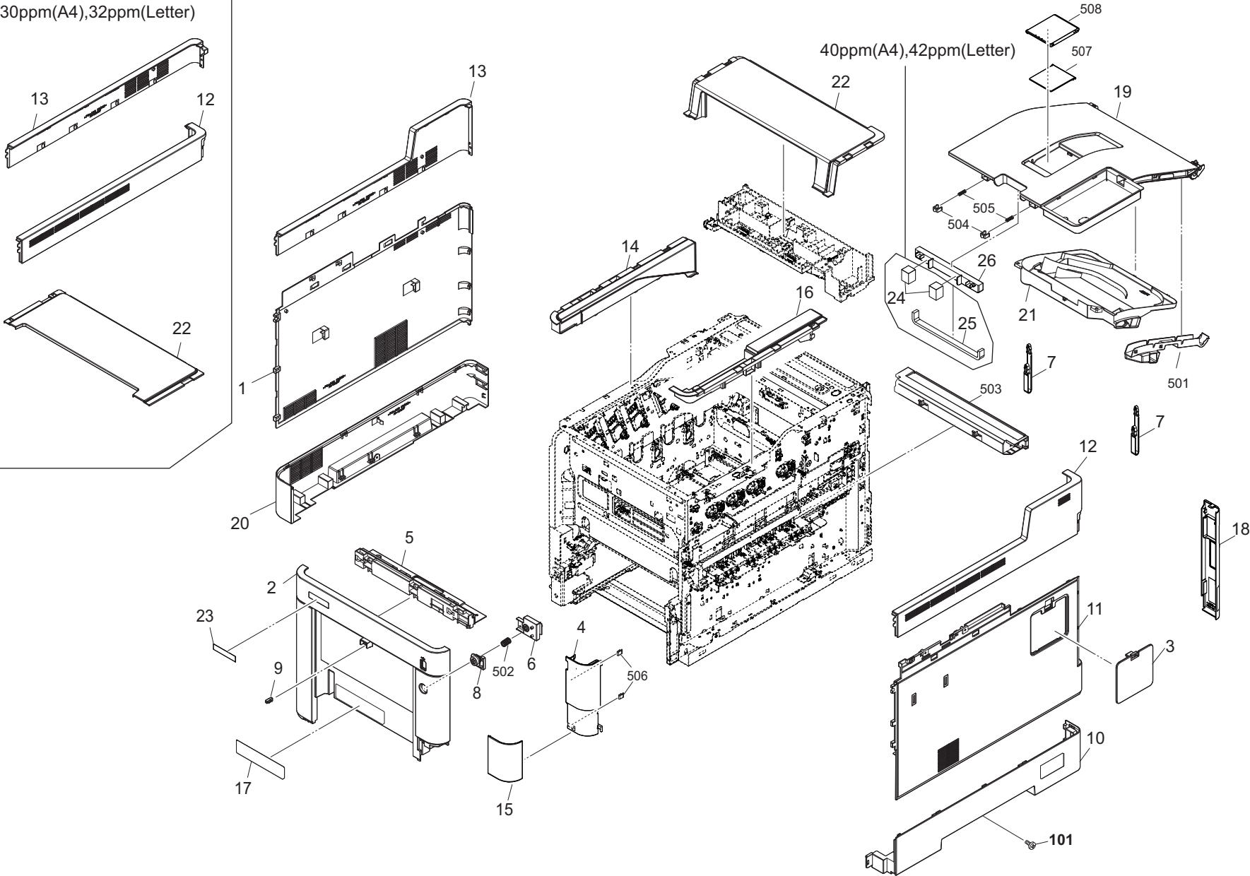
FIG. 1 Covers
