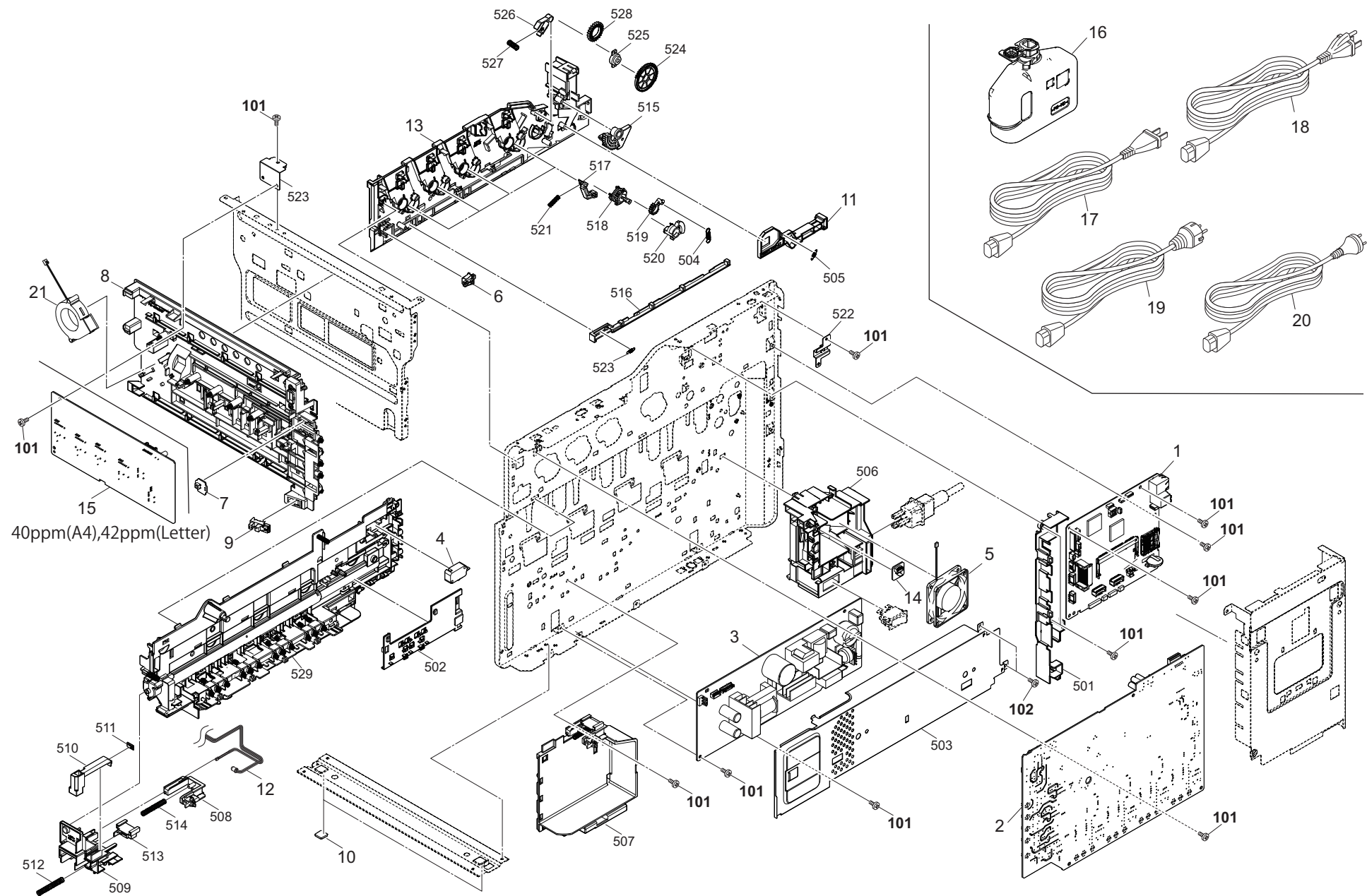
FIG. 14 Electrical Components 2
