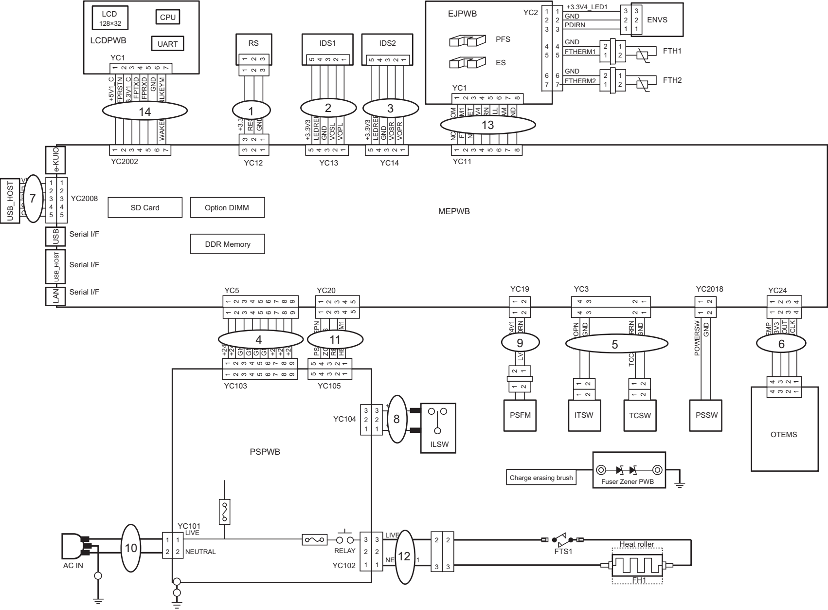
FIG. 16 Wire Section 1 (30ppm(A4),32ppm(Letter))
