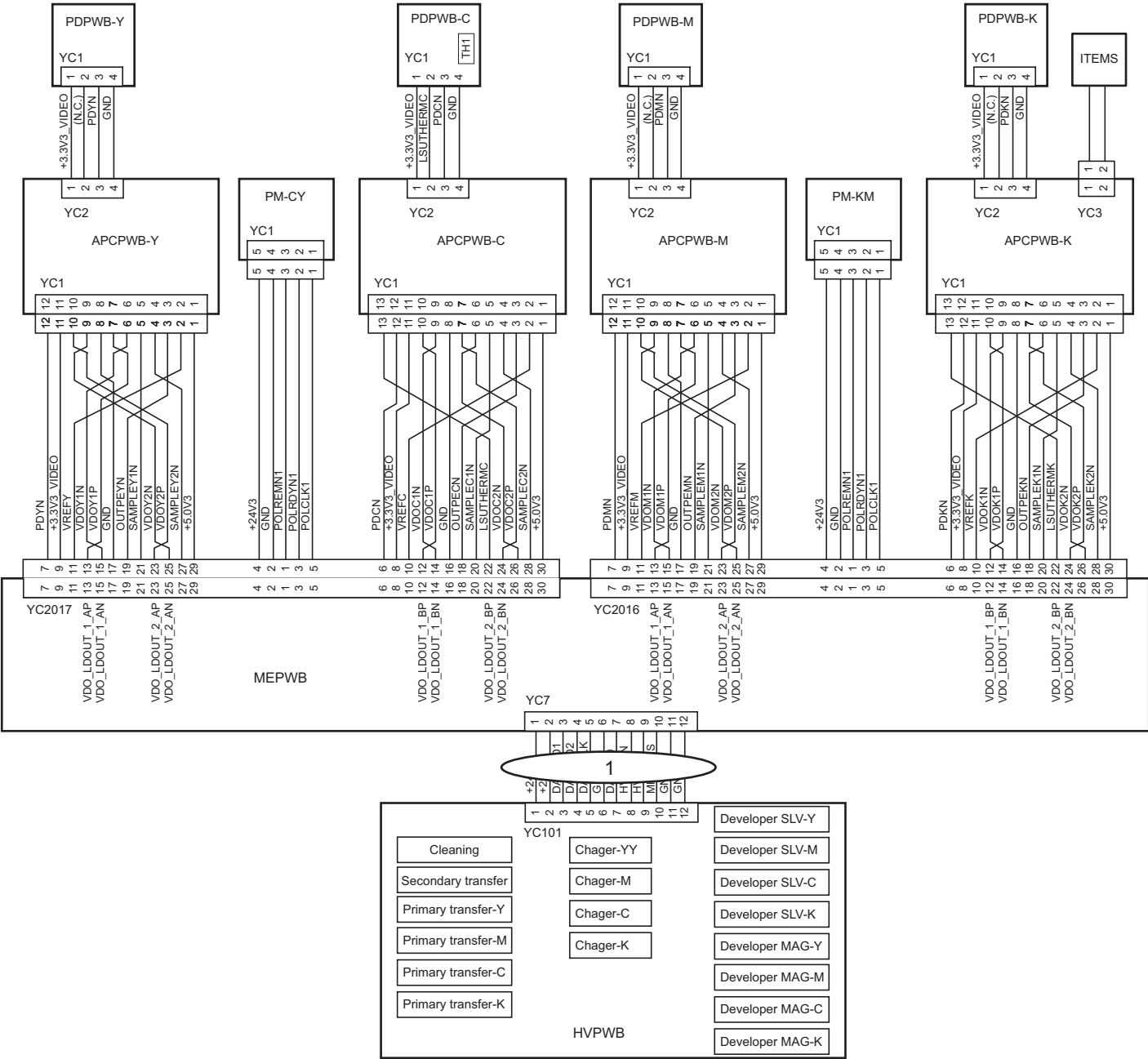
FIG. 17 Wire Section 2 (30ppm(A4),32ppm(Letter)/35ppm(A4),37ppm(Letter))
