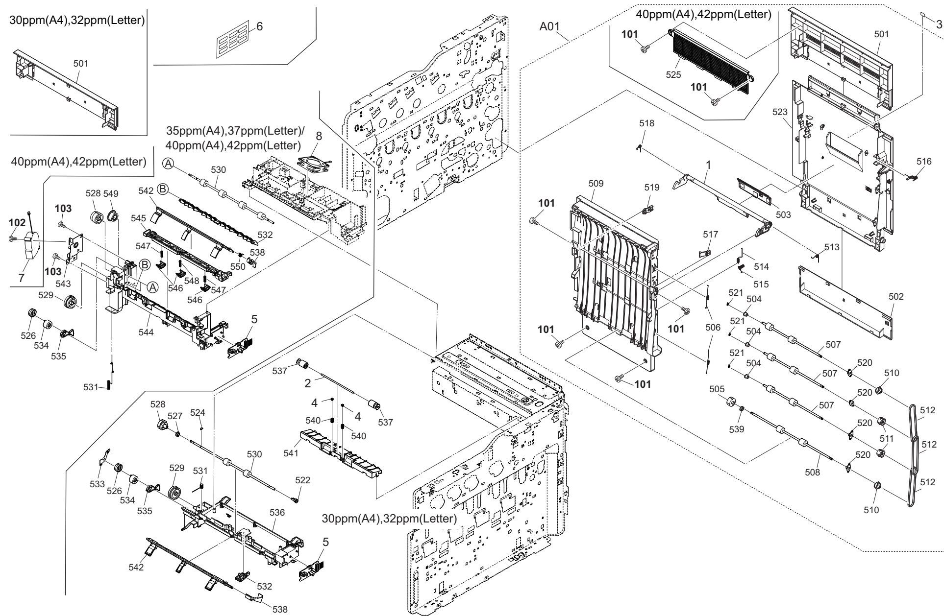
FIG. 5 Conveying Section 1
