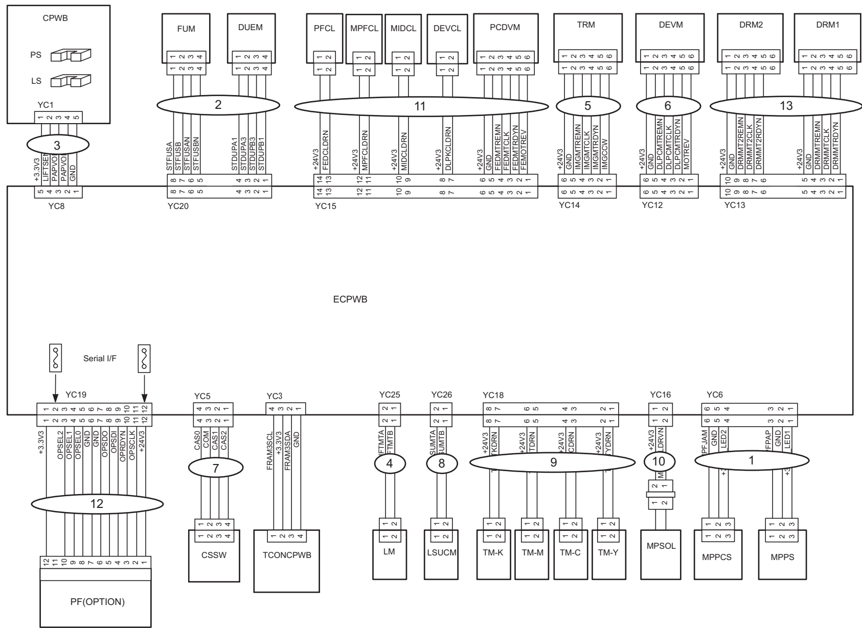
FIG. 19 Wire Section 4 (30ppm(A4),32ppm(Letter))
