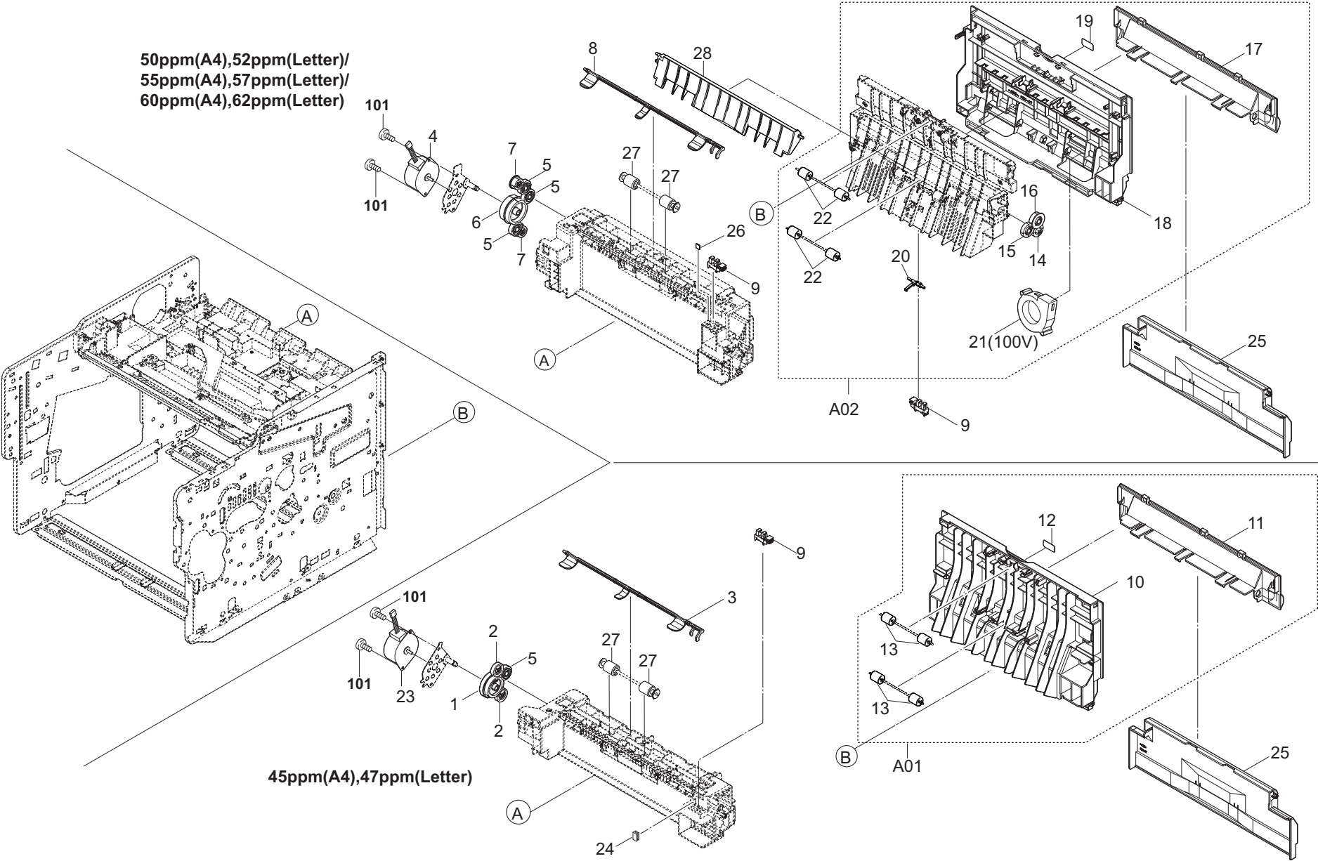
FIG. 8 Exit Section
