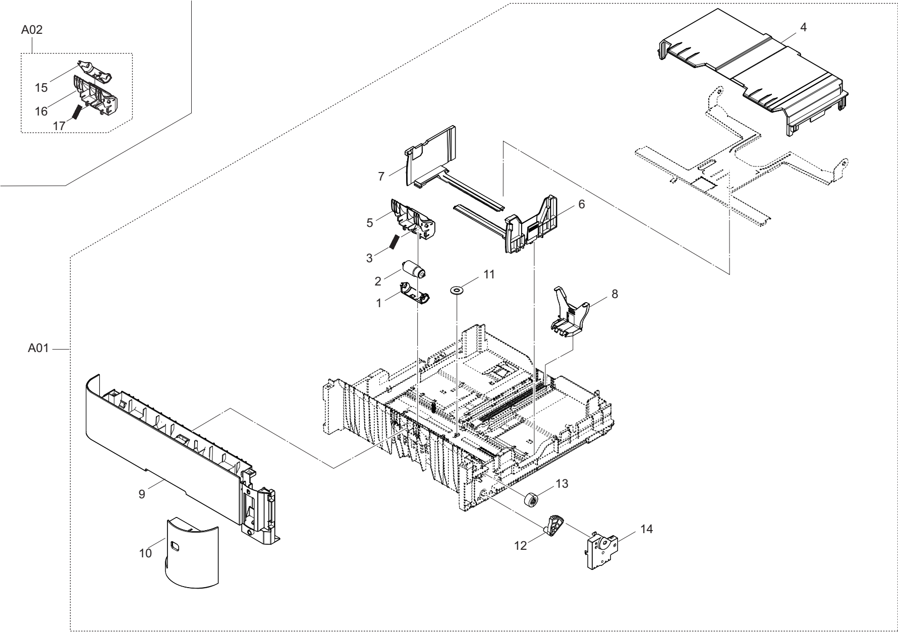
FIG. 3 Paper Cassette
