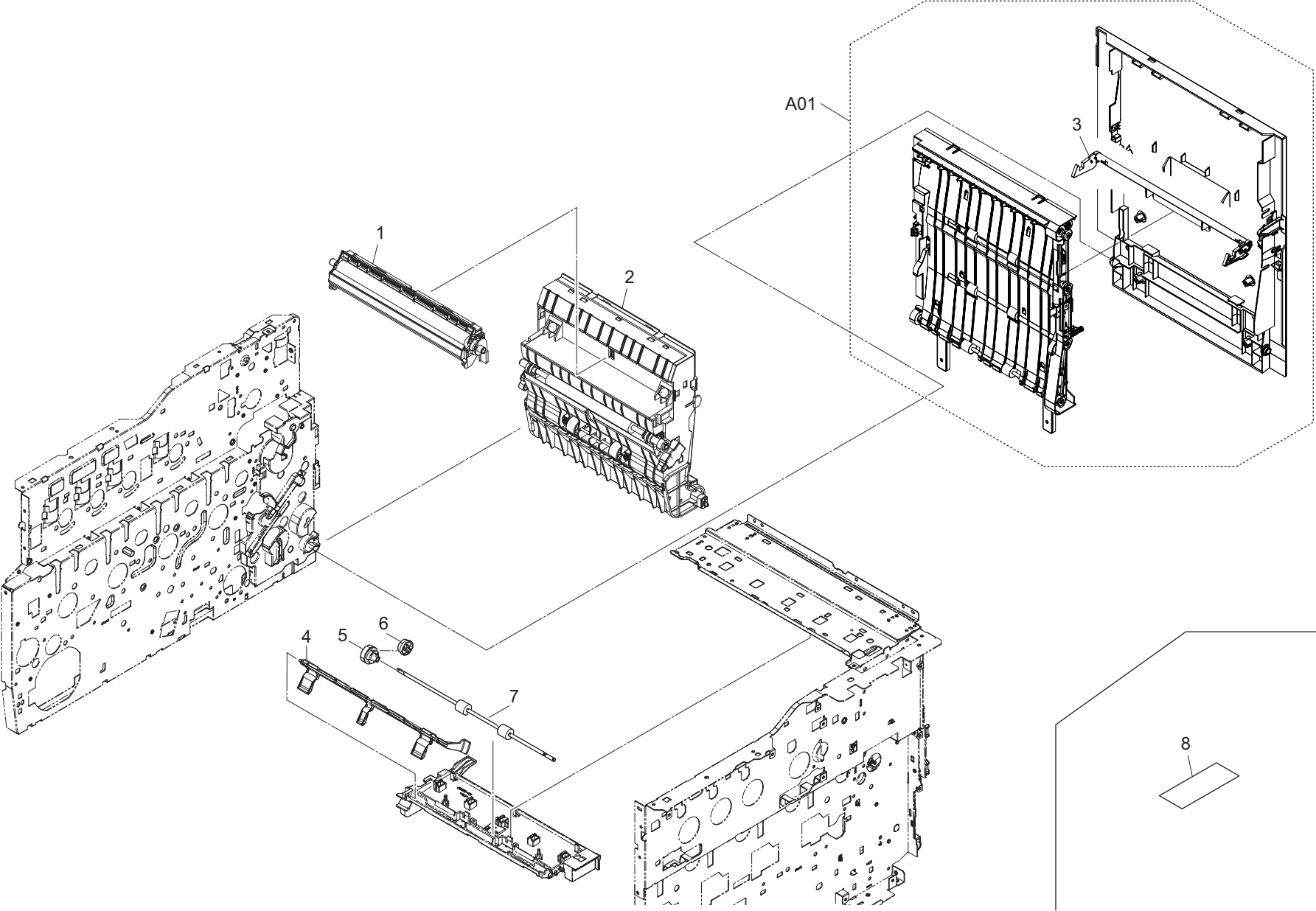
FIG. 5 Paper Conveying Section
