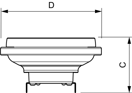
MAS LEDspot LV D 20-100W 840 AR111 24D
