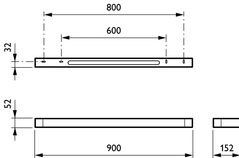
SmartBalance Wall-mounted WL484
