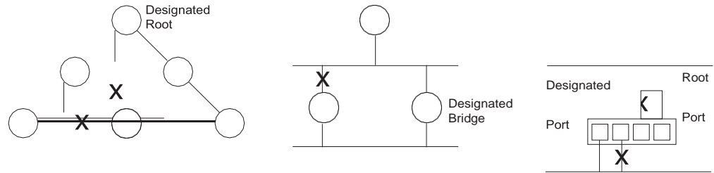
Figure 100: STP Root Ports and Designated Ports
