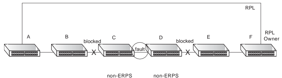
Figure 272: Non-ERPS Device Protection
