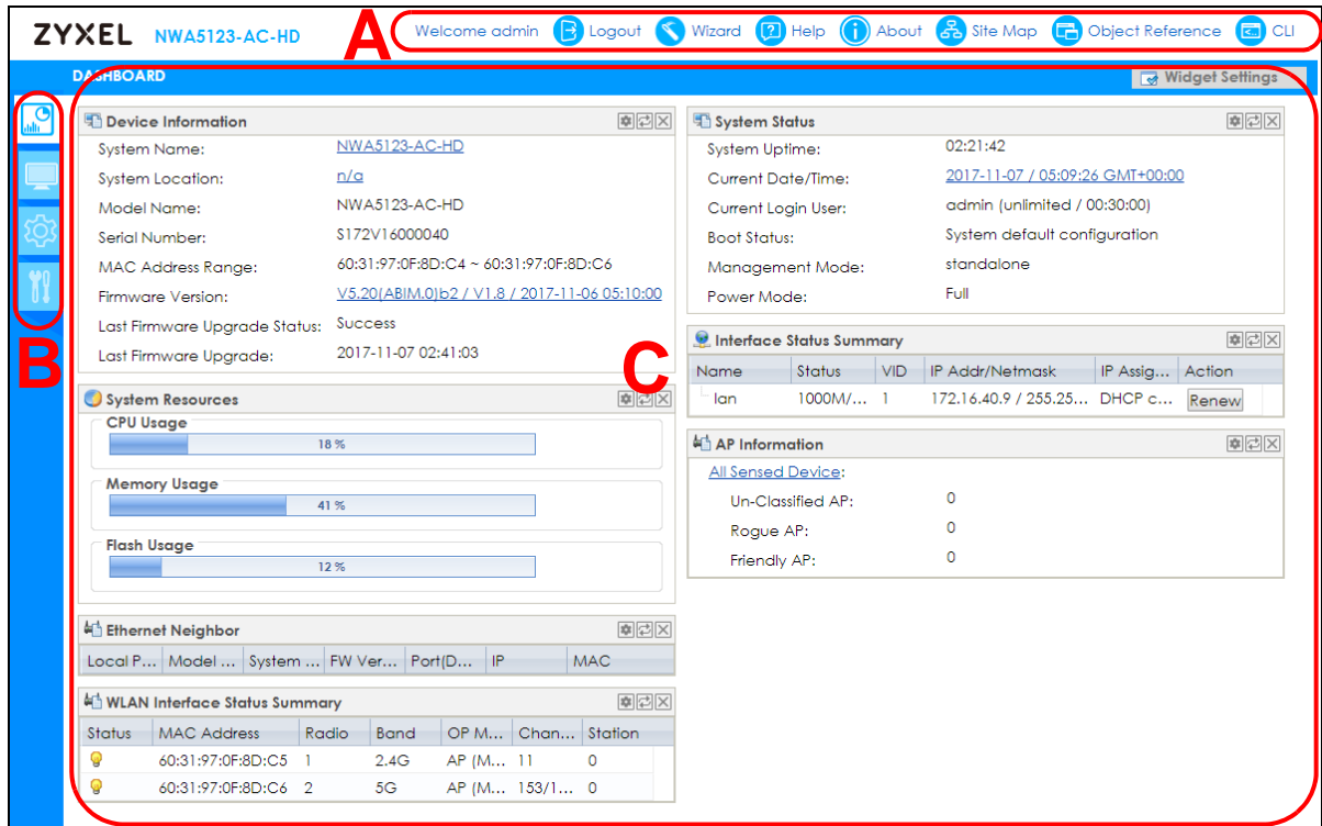
Figure 10 The Web Configurator's Main Screen
