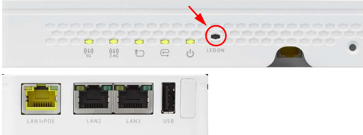
Figure 8 WAC5302D-S LEDs
