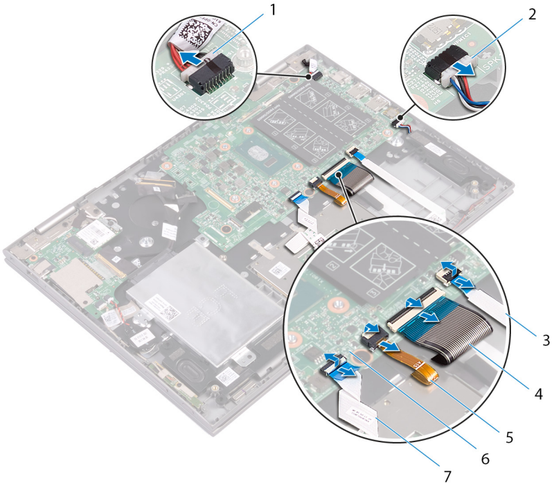
Figure 26. System board
