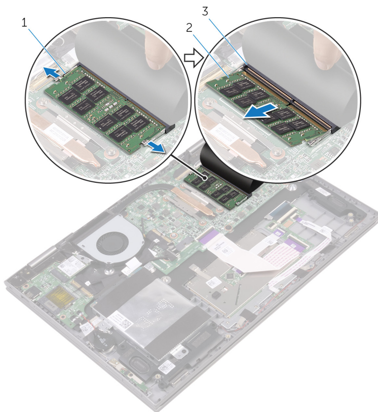
Figure 5. Memory module
