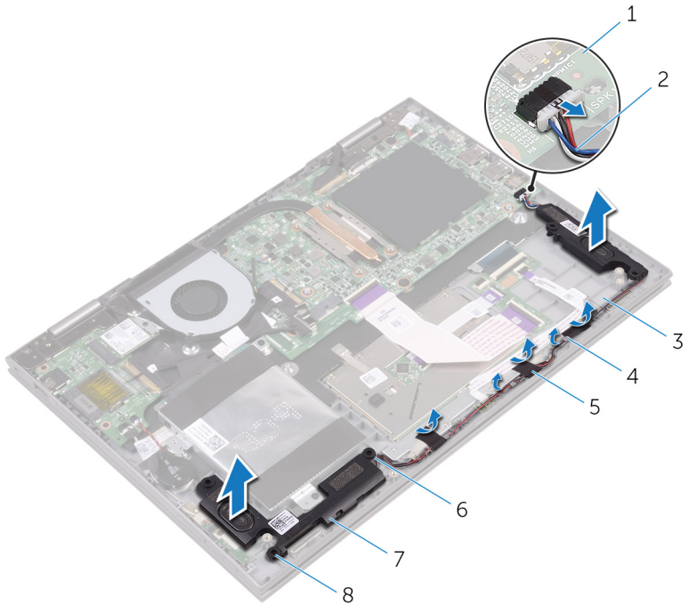
Figure 13. Speakers
