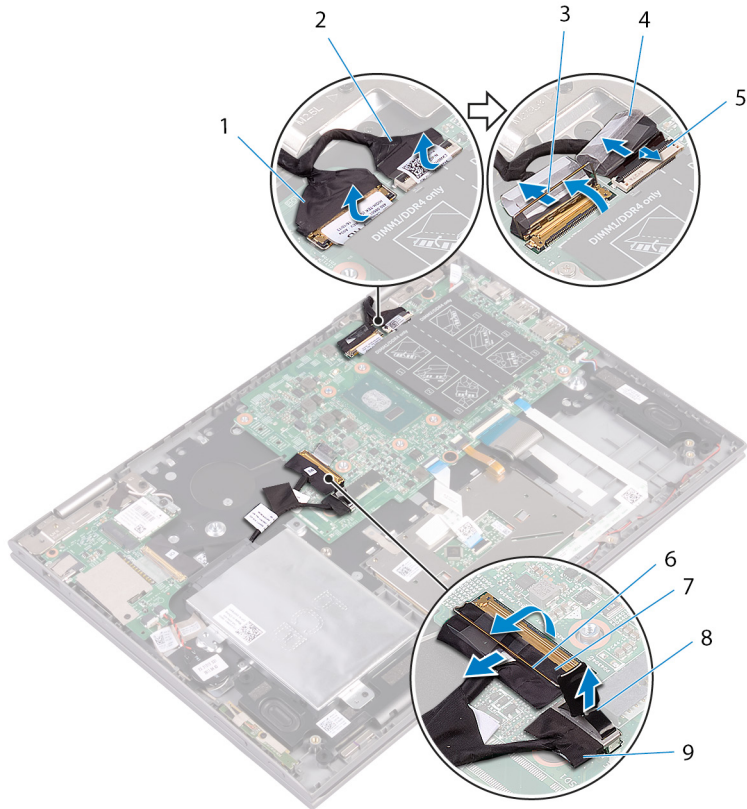
Figure 25. System board
