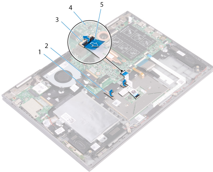
Figure 18. Touchpad
