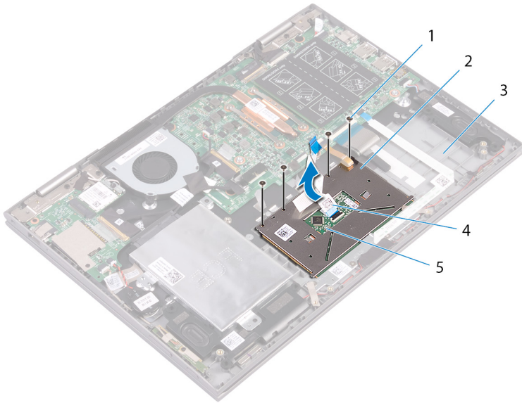
Figure 19. Touchpad
