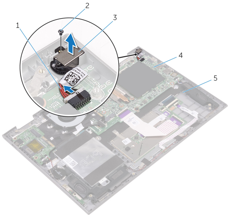
Figure 24. Power-adapter port
