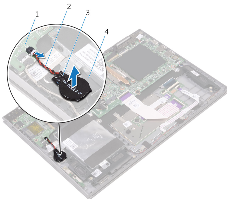
Figure 10. Coin-cell battery
