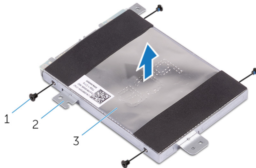
Figure 9. Hard drive
