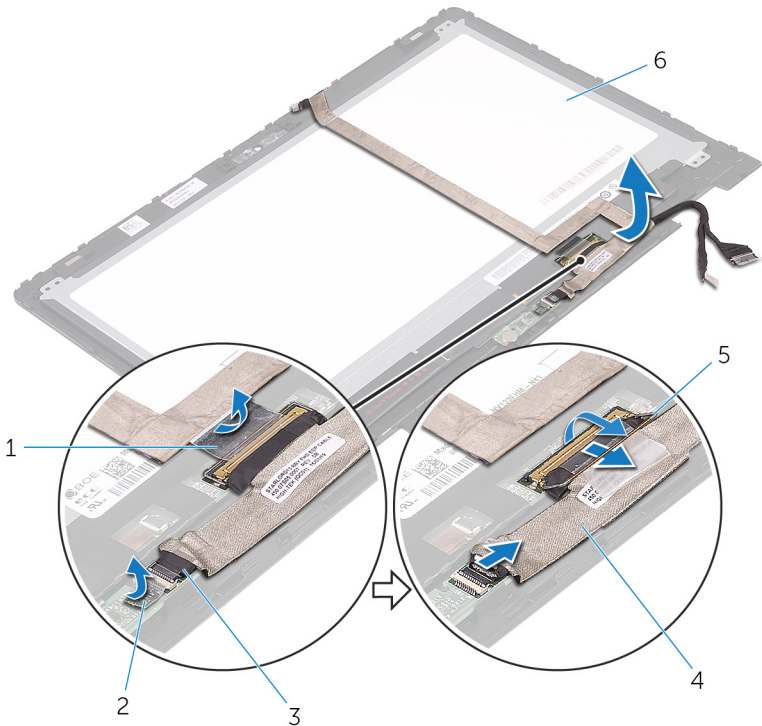
Figure 33. Display cable
