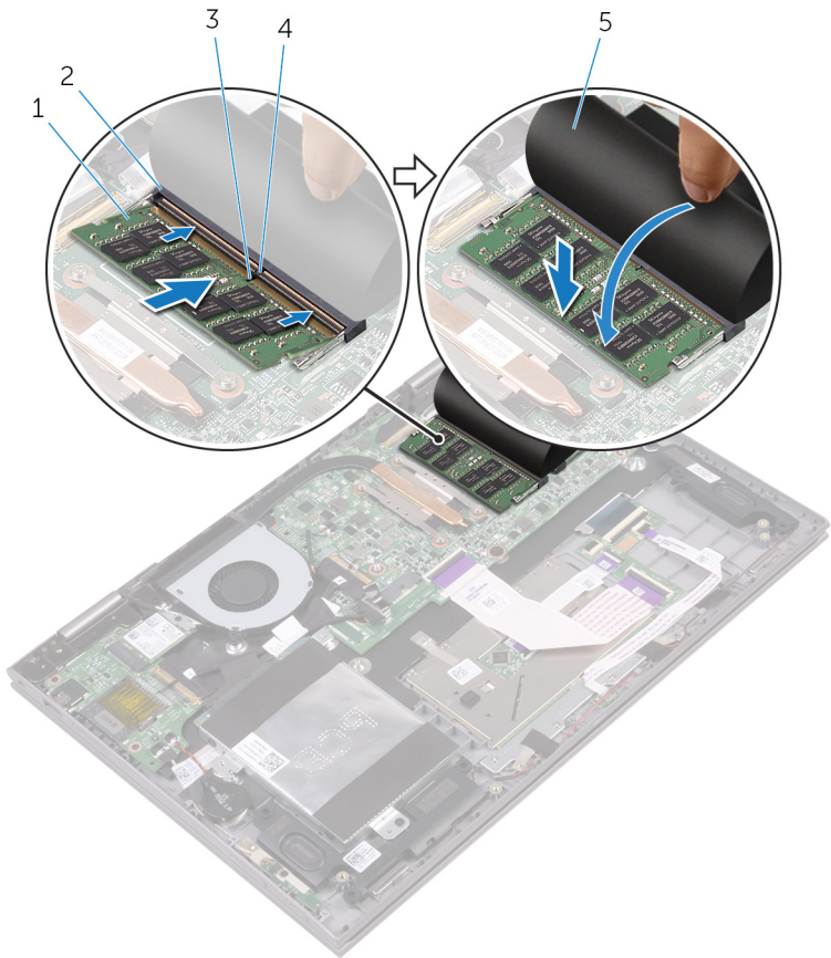
Figure 6. Memory module
