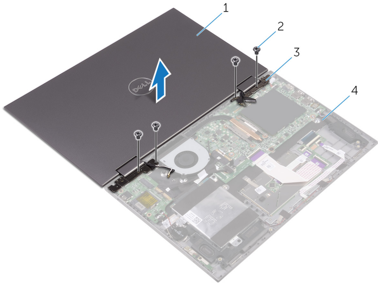
Figure 22. Display assembly
