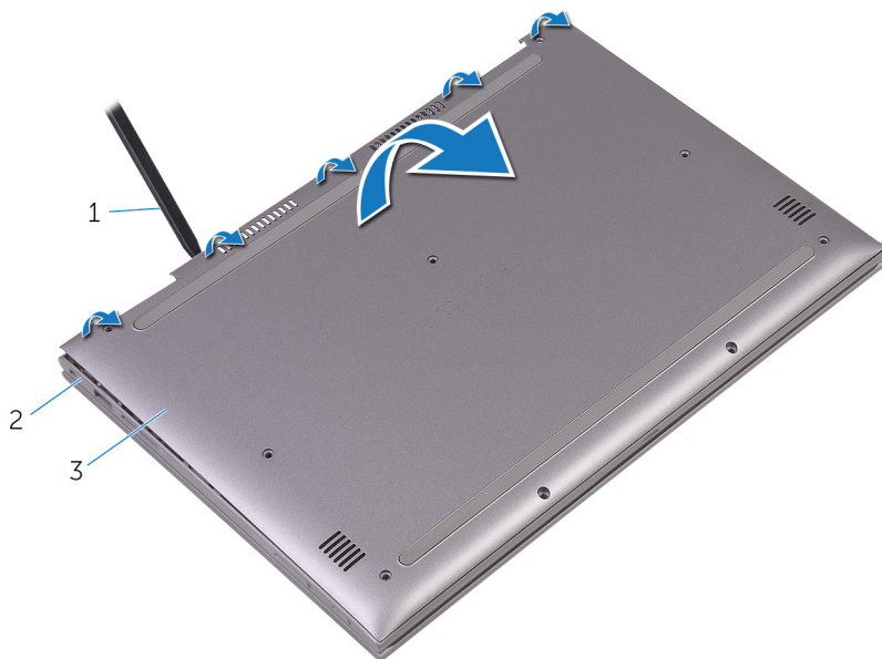
Figure 2. Base cover
