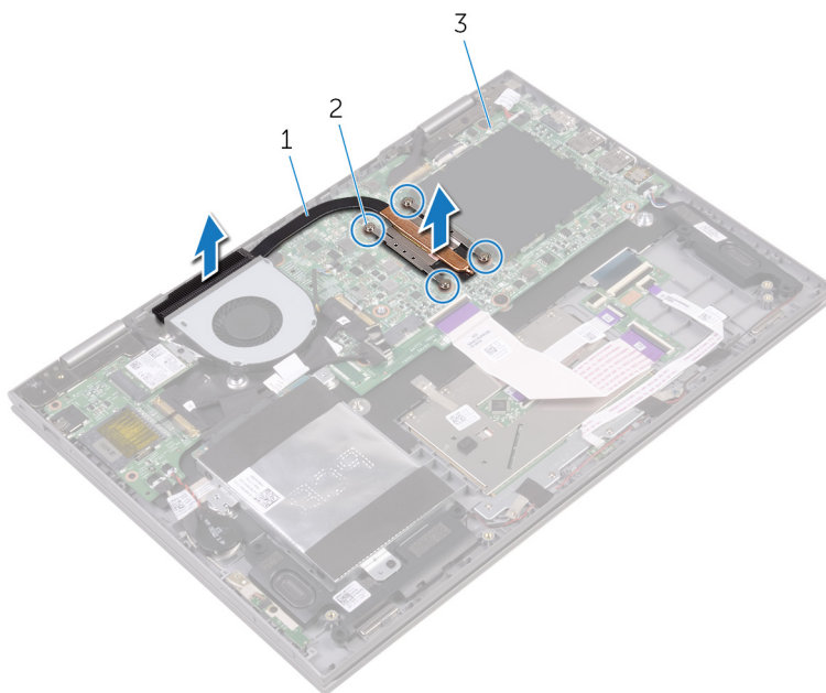
Figure 15. Heat sink
