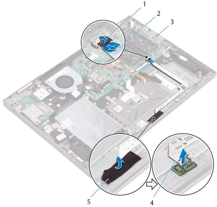
Figure 17. Status-light board
