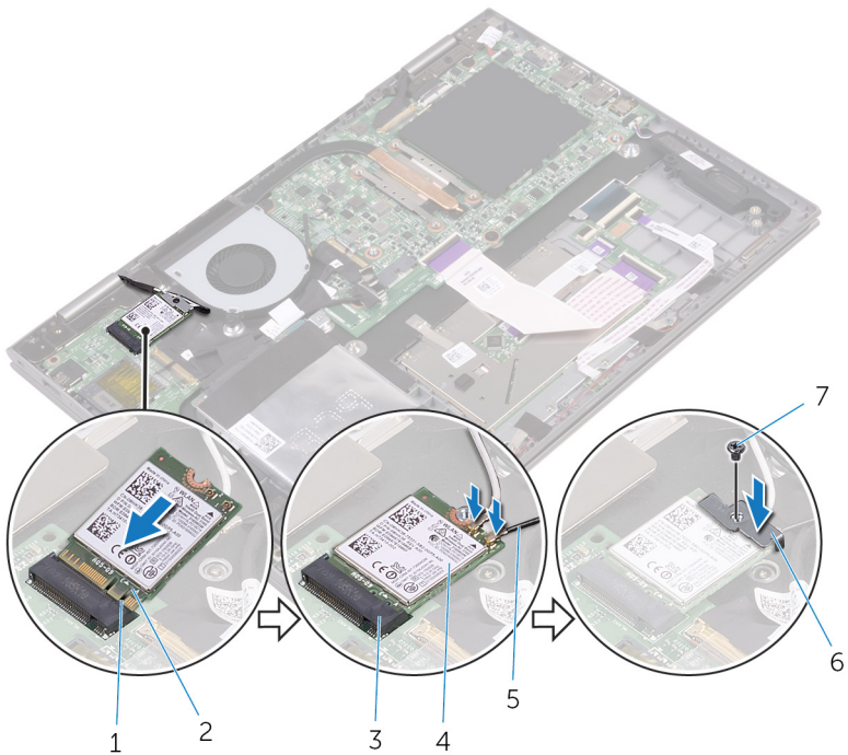
Figure 12. Wireless card
