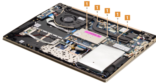
Figure 7. Removal steps of fan and heat sink assembly
