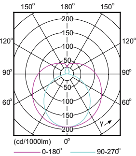
CorePro LEDtube HF 600mm 9W G13 840, 865 800lm T8 G
