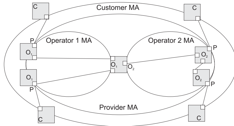
Figure 306: Multiple CFM Maintenance Domains
