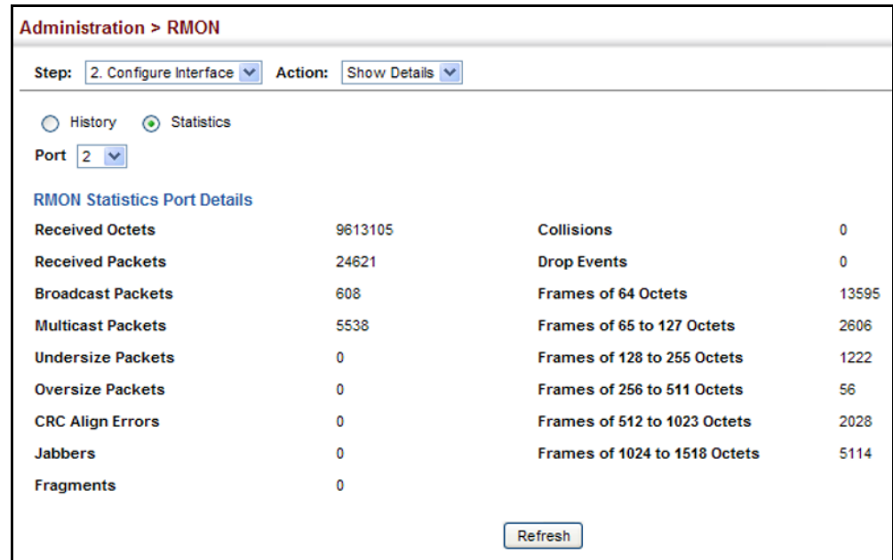
Figure 289: Showing Collected RMON Statistical Samples
