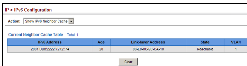
Figure 404: Showing IPv6 Neighbors
