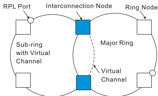
Figure 298: Sub-ring with Virtual Channel
