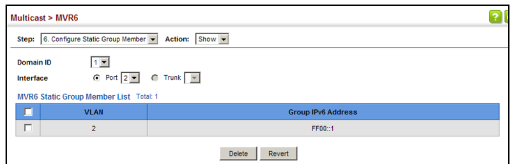
Figure 391: Showing the Static MVR6 Groups Assigned to a Port
