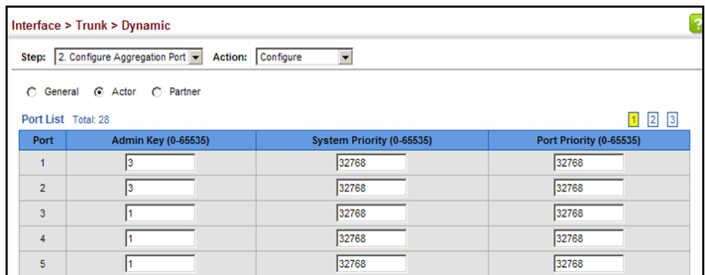
Figure 56: Configuring LACP Parameters on a Port
