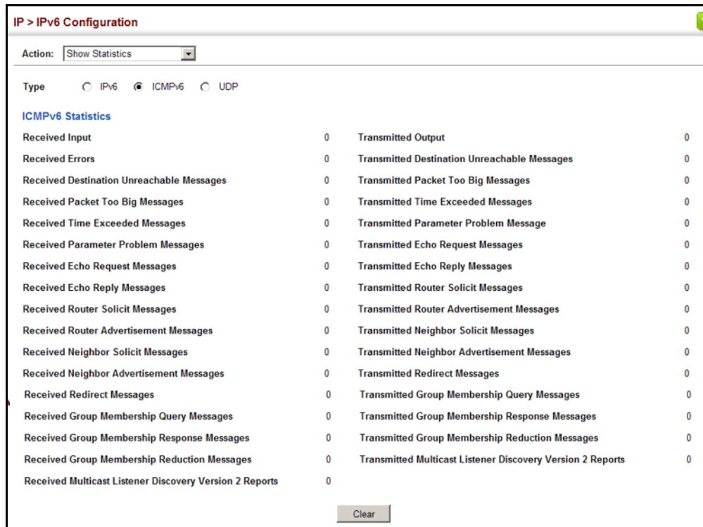
Figure 406: Showing IPv6 Statistics (ICMPv6)
