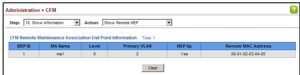
Figure 325: Showing Information on Remote MEPs
