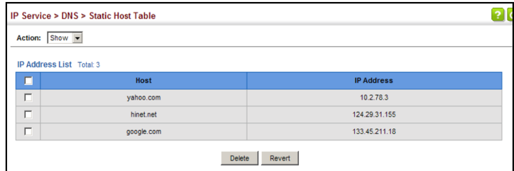
Figure 415: Showing Static Entries in the DNS Table
