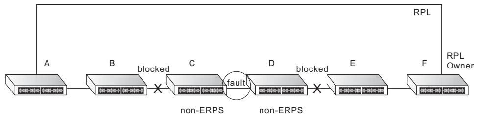
Figure 300: Non-ERPS Device Protection
