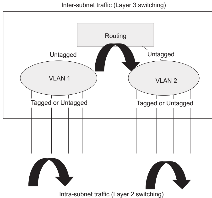
Figure 423: Virtual Interfaces and Layer 3 Routing
