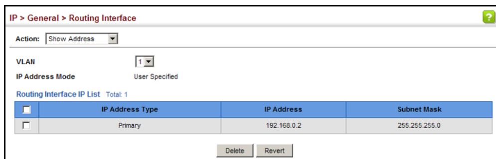
Figure 398: Showing the Configured IPv4 Address for an Interface
