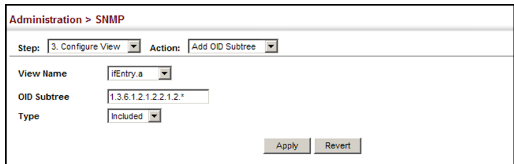
Figure 262: Adding an OID Subtree to an SNMP View
