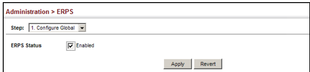
Figure 297: Setting ERPS Global Status
