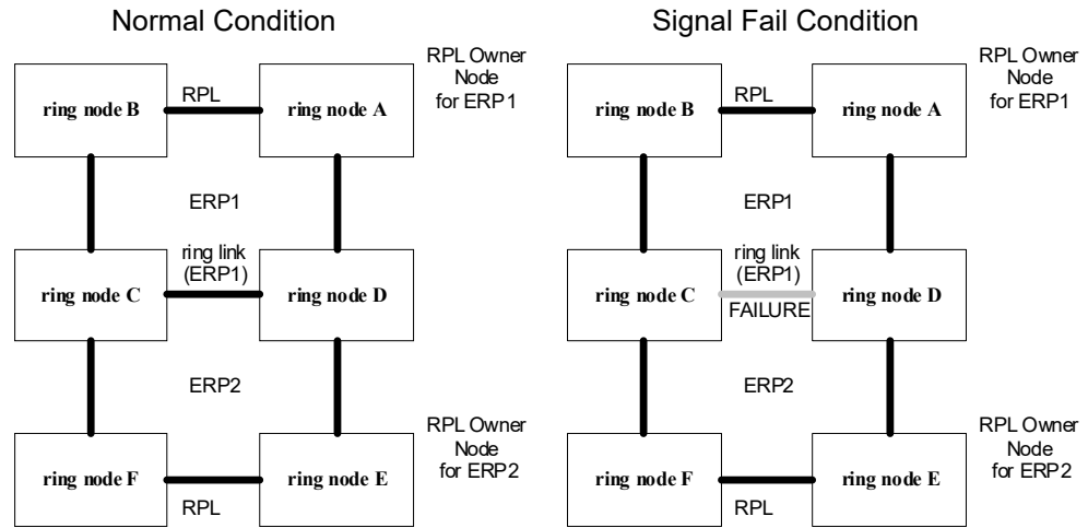
Figure 296: Ring Interconnection Architecture (Multi-ring/Ladder Network)
