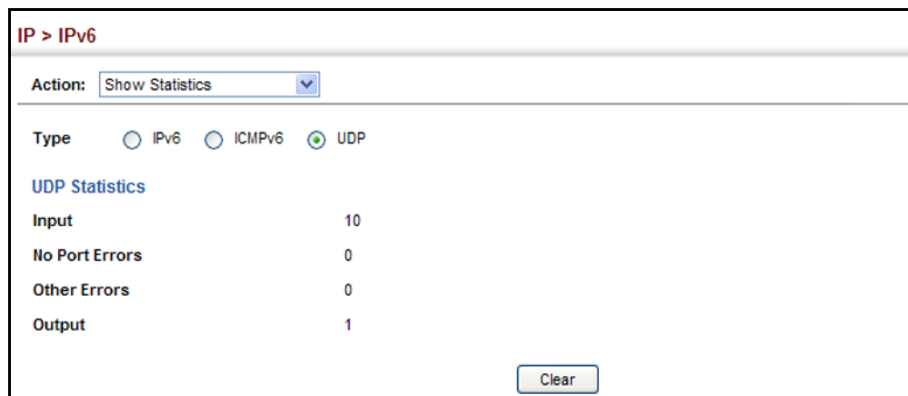
Figure 407: Showing IPv6 Statistics (UDP)
