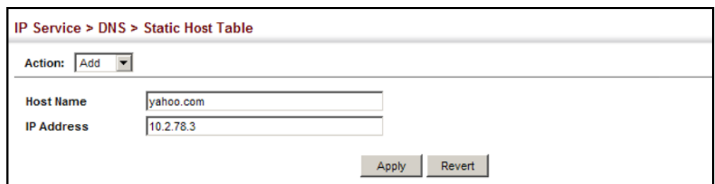
Figure 414: Configuring Static Entries in the DNS Table
