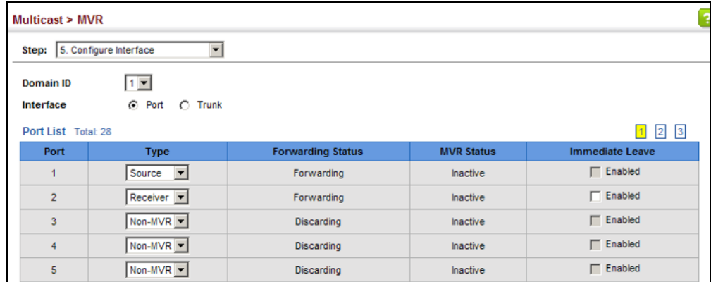
Figure 376: Configuring Interface Settings for MVR
