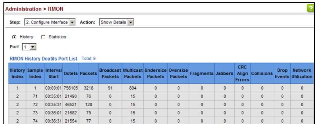
Figure 286: Showing Collected RMON History Samples
