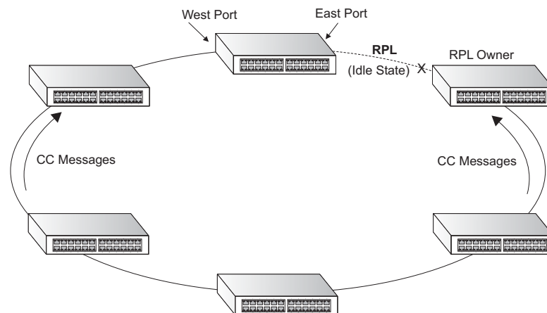
Figure 295: ERPS Ring Components
