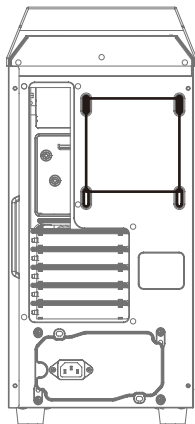
Rear: Supports the installation of 120mm fan or 120mm Radiator
