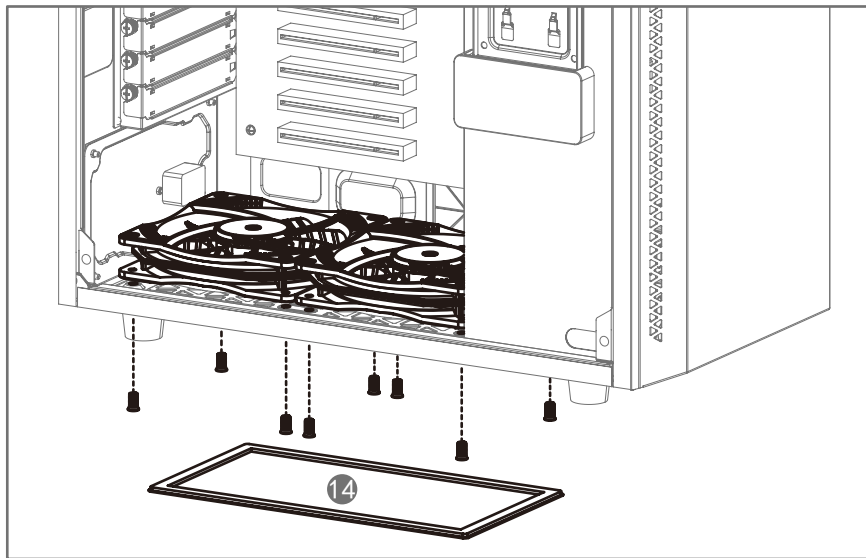
Installation of fans at bottom
