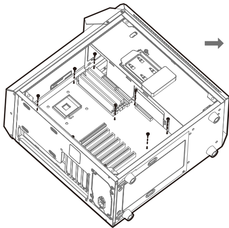
Installation of ATX MB
