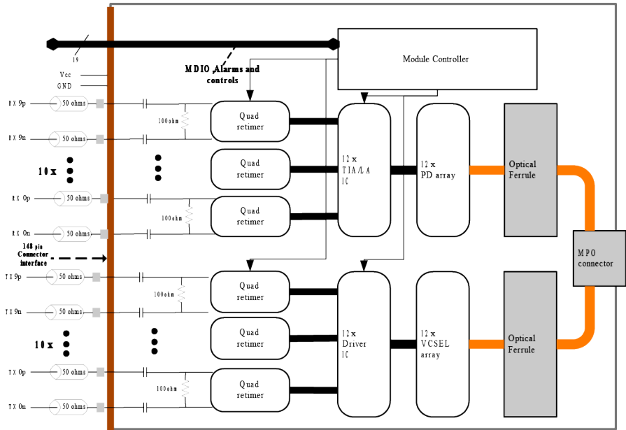
CFP Module Functional Block Diagram
