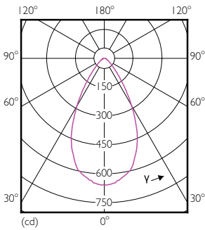
MAS VLE LEDspotLV 50W GU5-3 827 60D MR16
