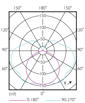
CorePro LEDlinear MV 60W R7S 830 Linear
