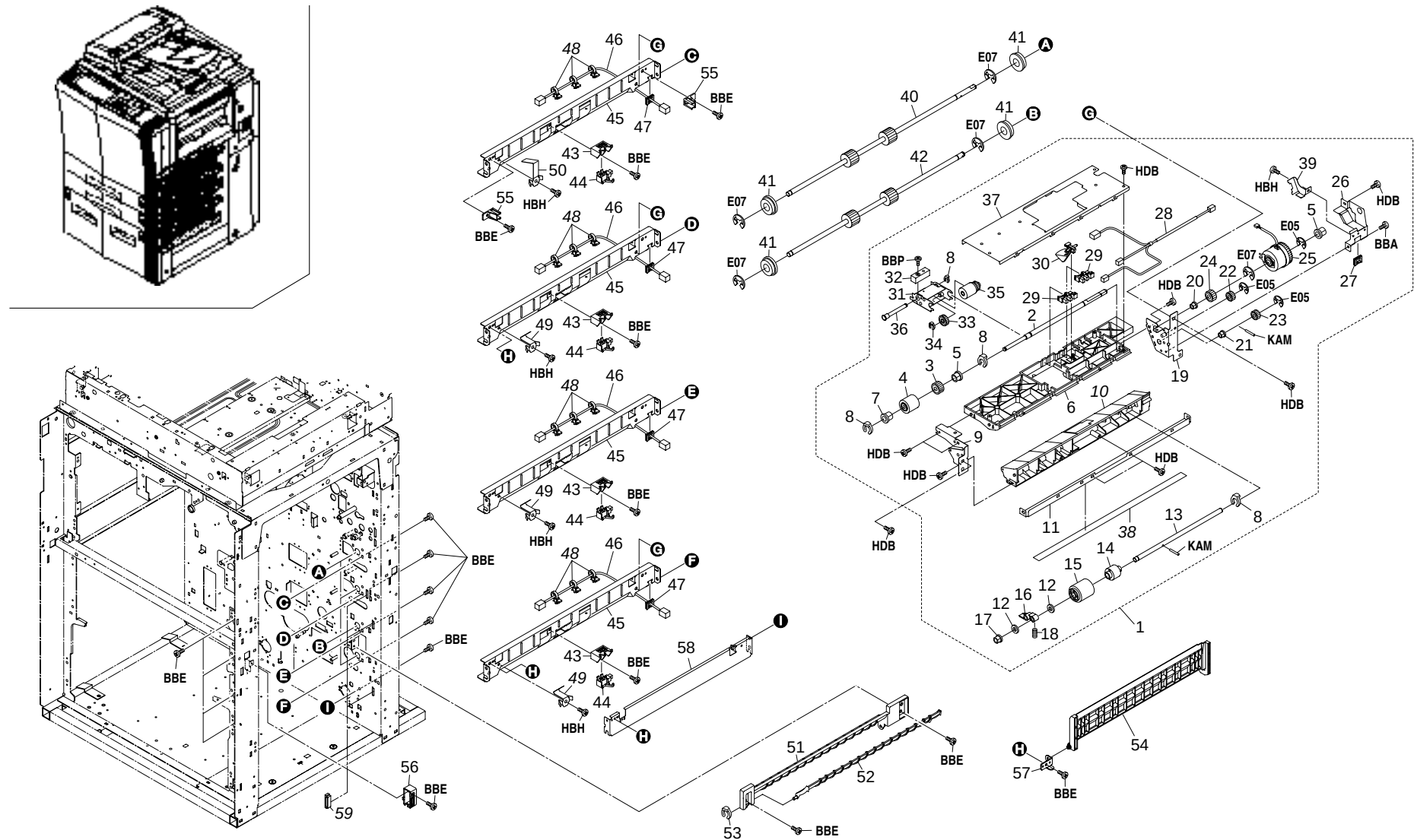
FIG. 7 PRIMARY PAPER FEED SECTION
