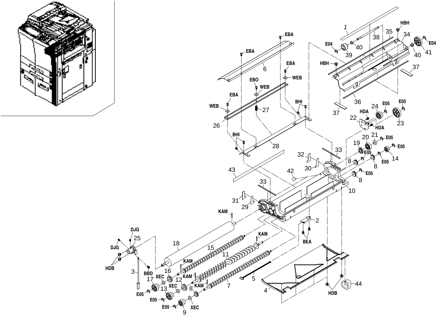
FIG. 13 DEVELOPING SECTION
