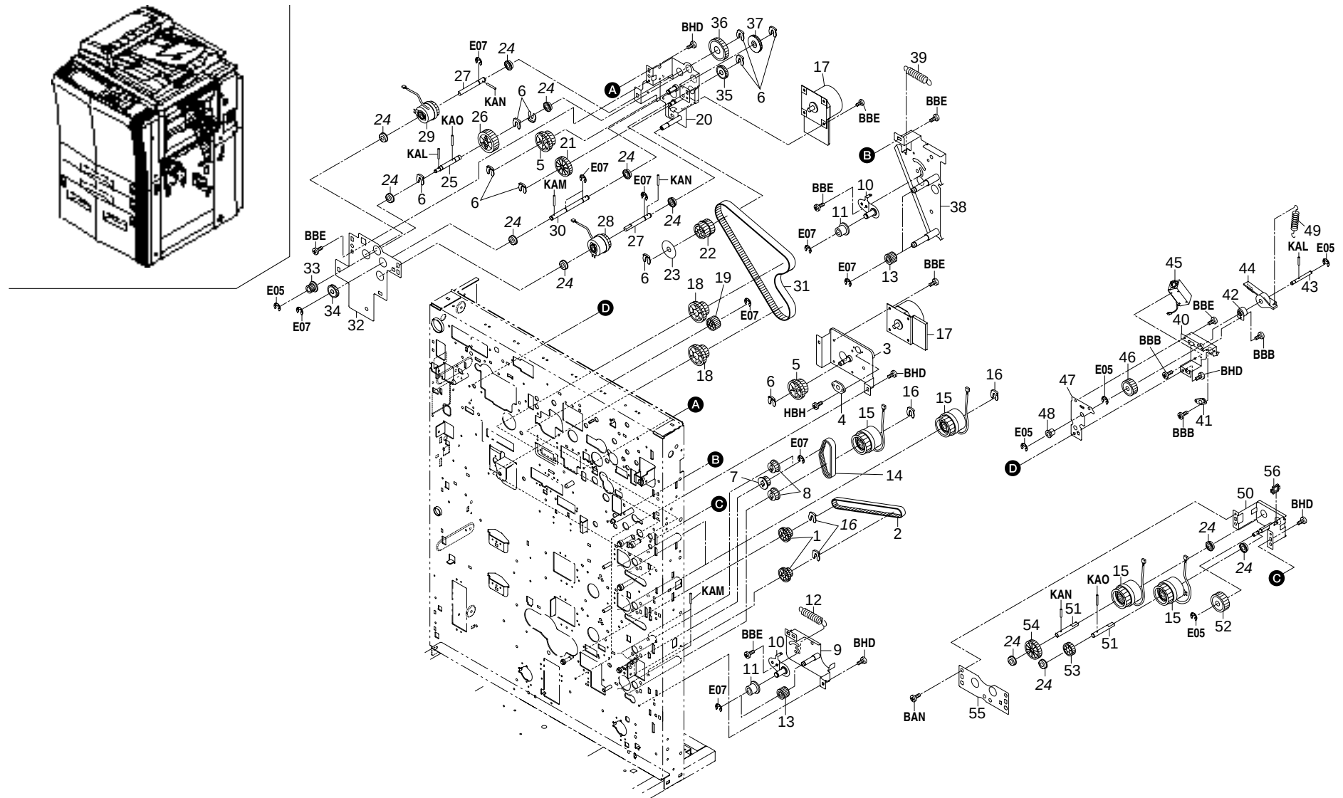
FIG. 21 DRIVING SECTION I
