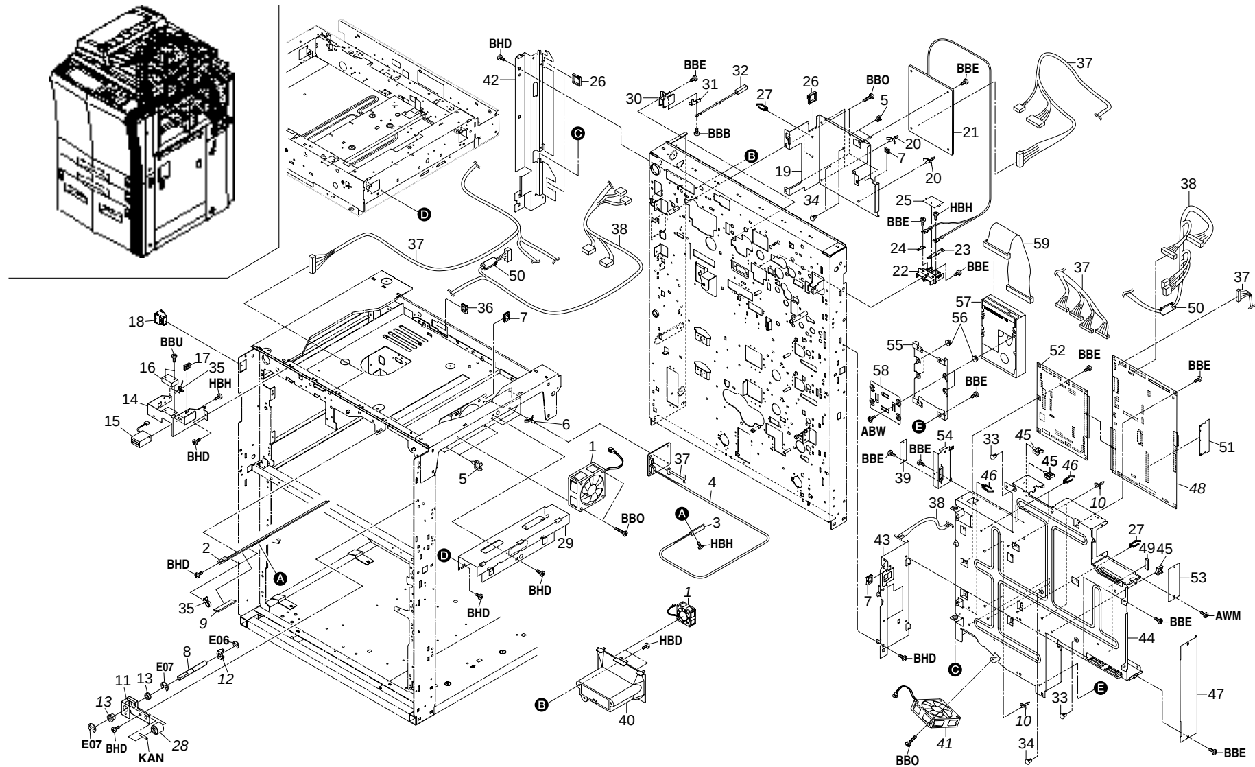
FIG. 40 ELECTRICAL SECTION II
