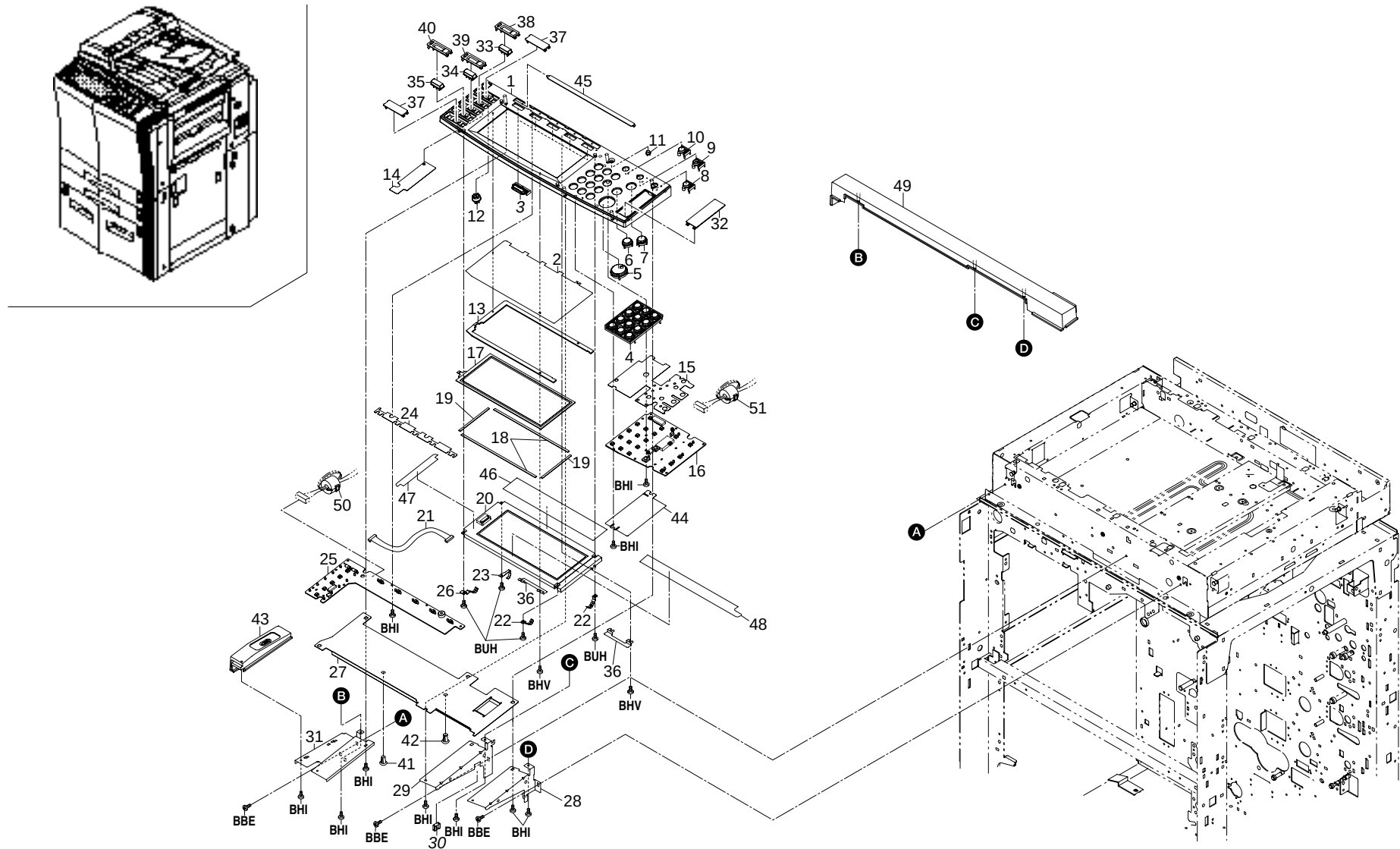
FIG. 41 OPERATION SECTION
