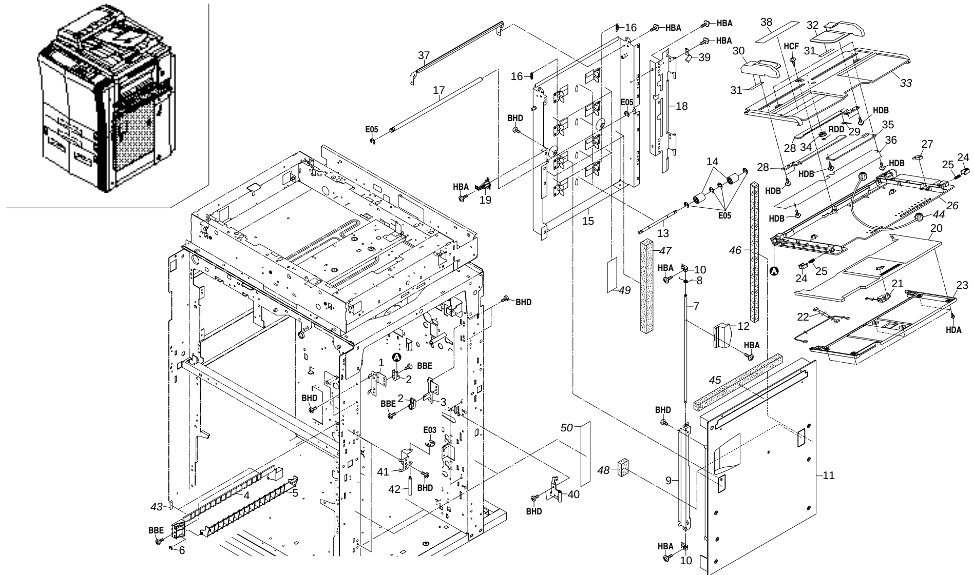
FIG. 28 BYPASS & VERTICAL CONVEYING SECTION
