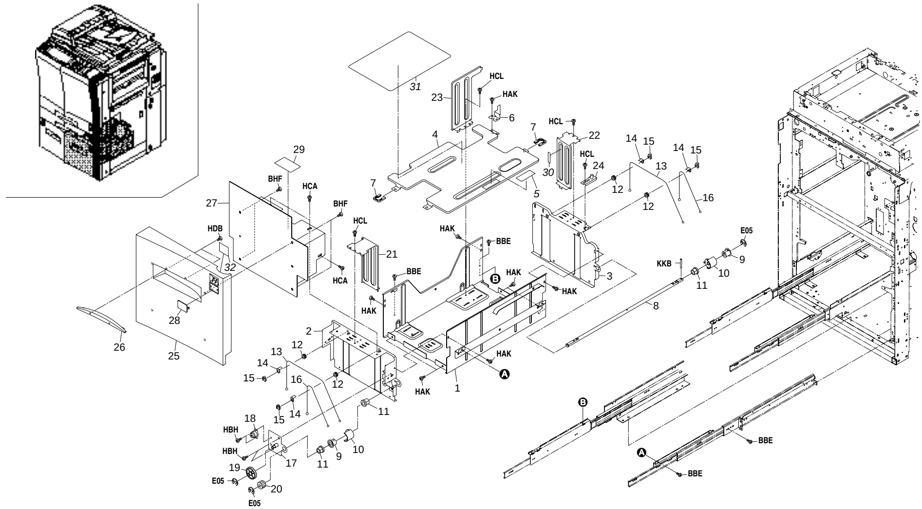
FIG. 4 DECK A SECTION
