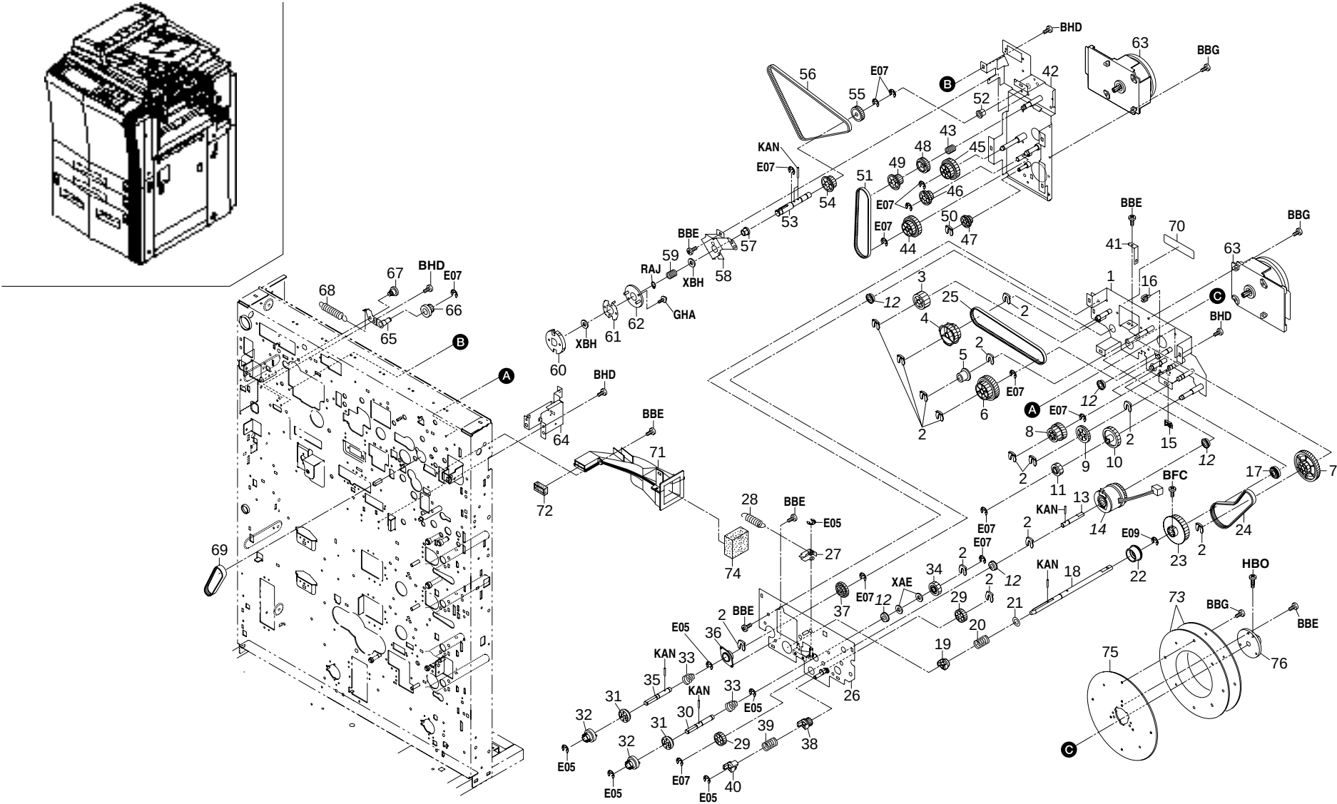
FIG. 22 DRIVING SECTION II
