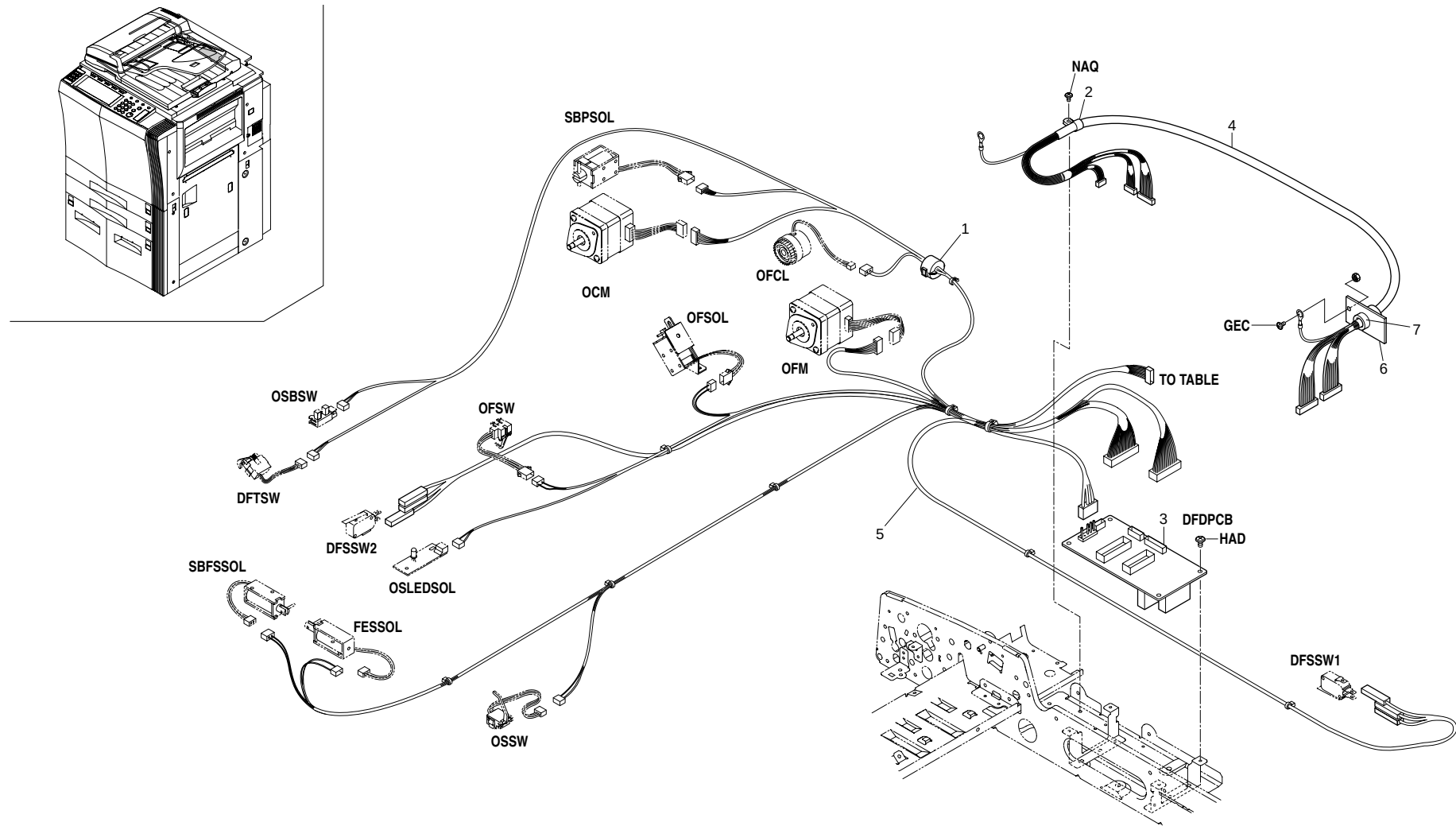
FIG. 38 ELECTRICAL SECTION (DF)
