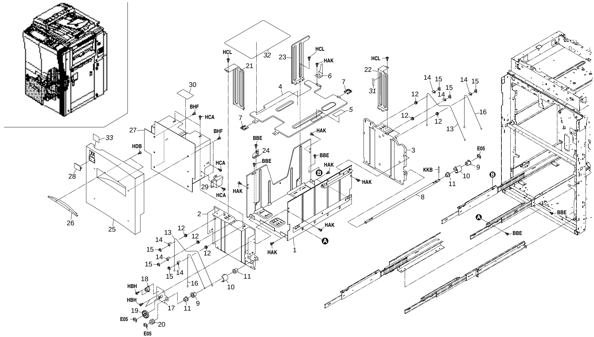
FIG. 5 DECK B SECTION
