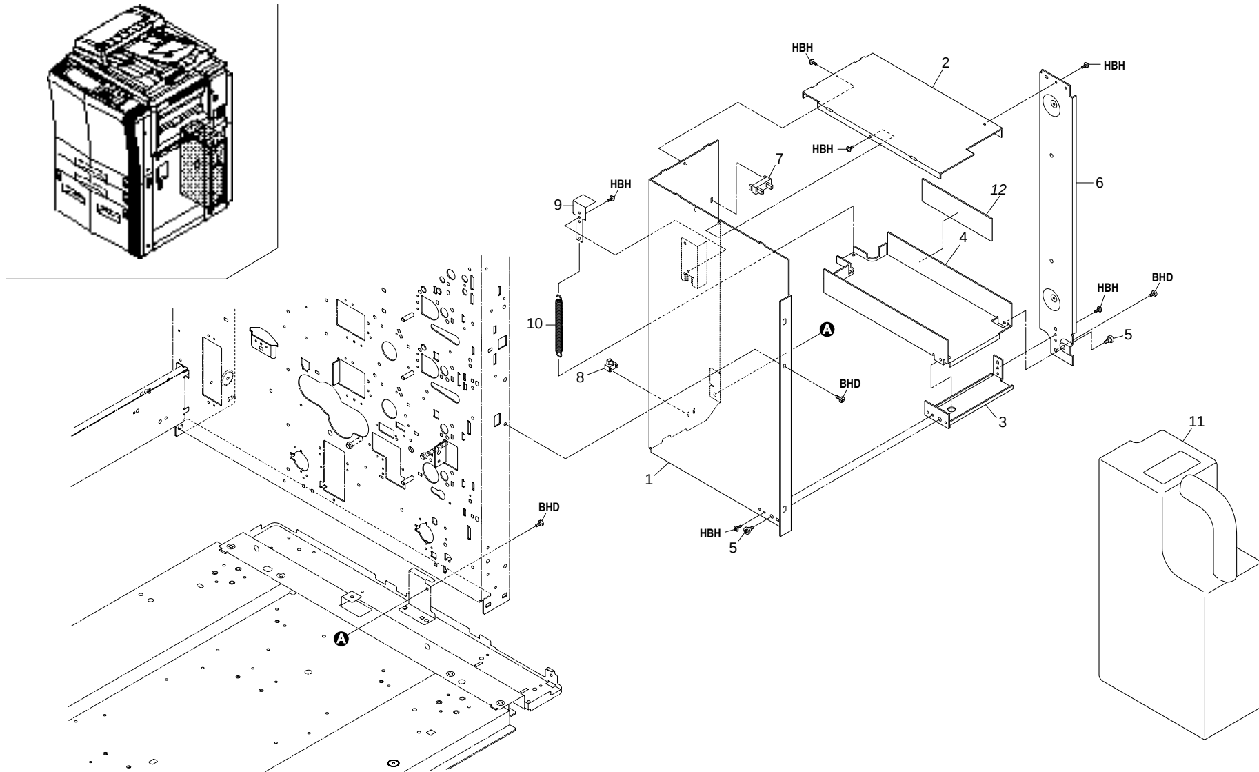
FIG. 15 CLEANING SECTION II
