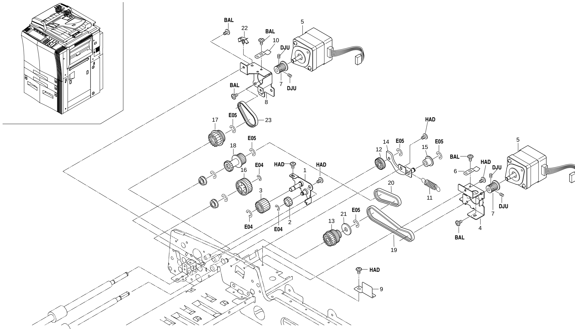
FIG. 37 DRIVING SECTION (DF)
