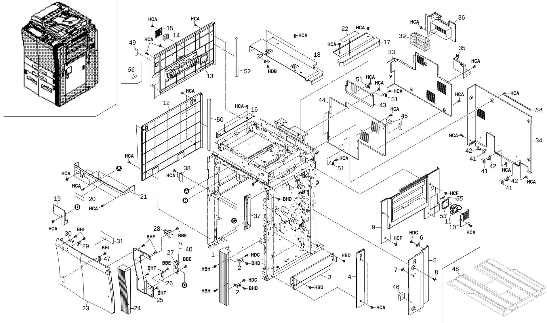
FIG. 1 COVER SECTION
