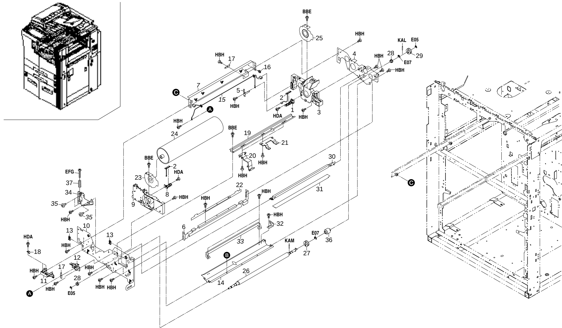
FIG. 8 IMAGING SECTION I
