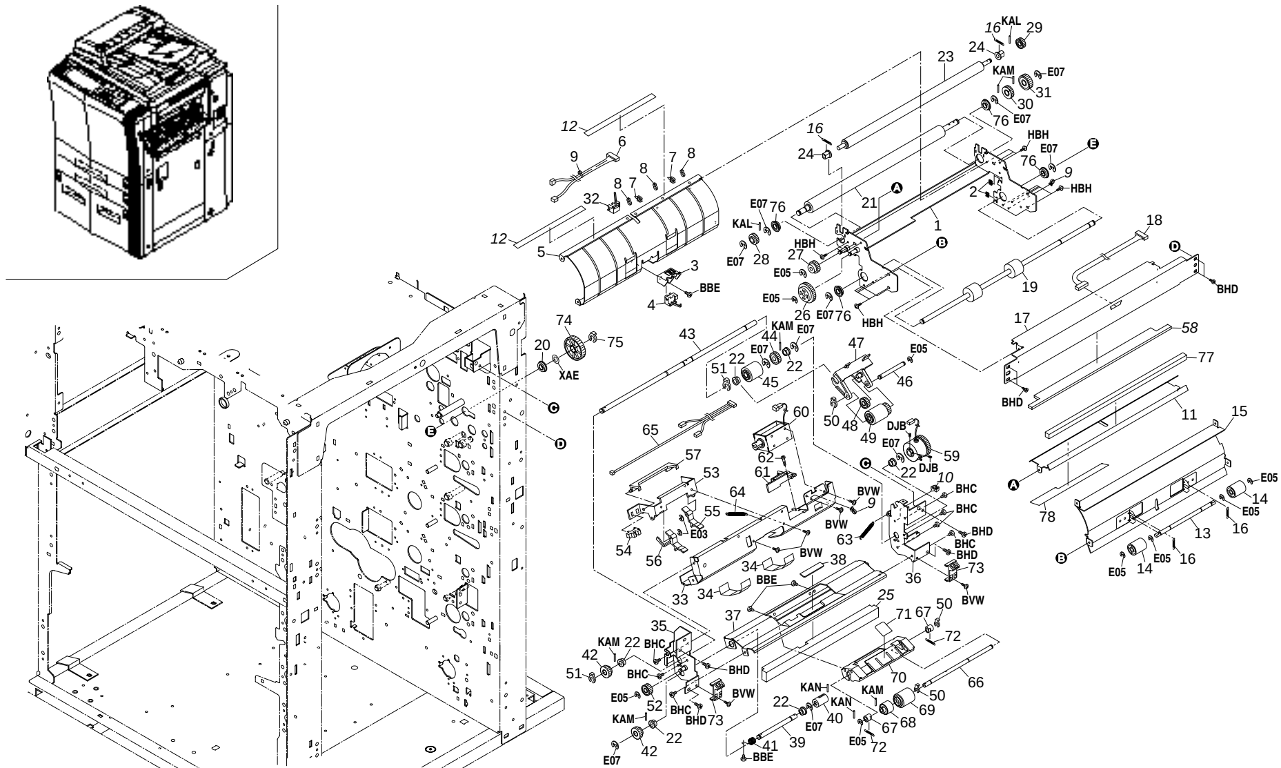
FIG. 27 BYPASS FEED SECTION
