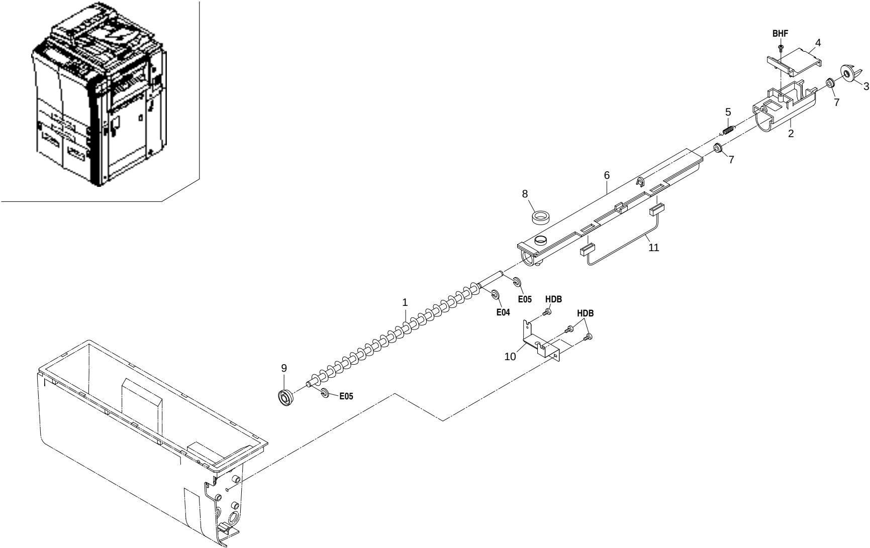
FIG. 30 HOPPER SECTION II
