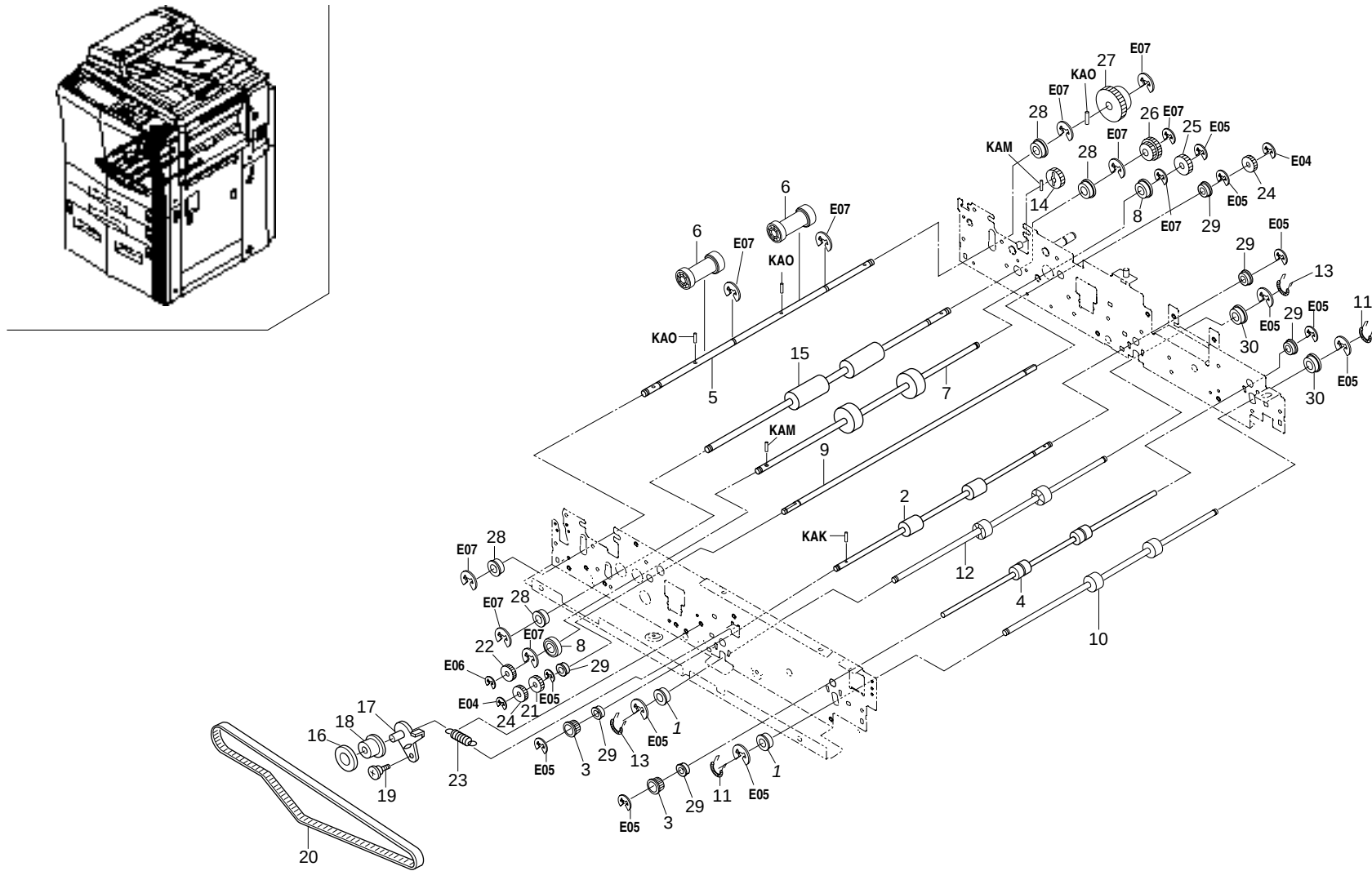
FIG. 25 DUPLEX SECTION III
