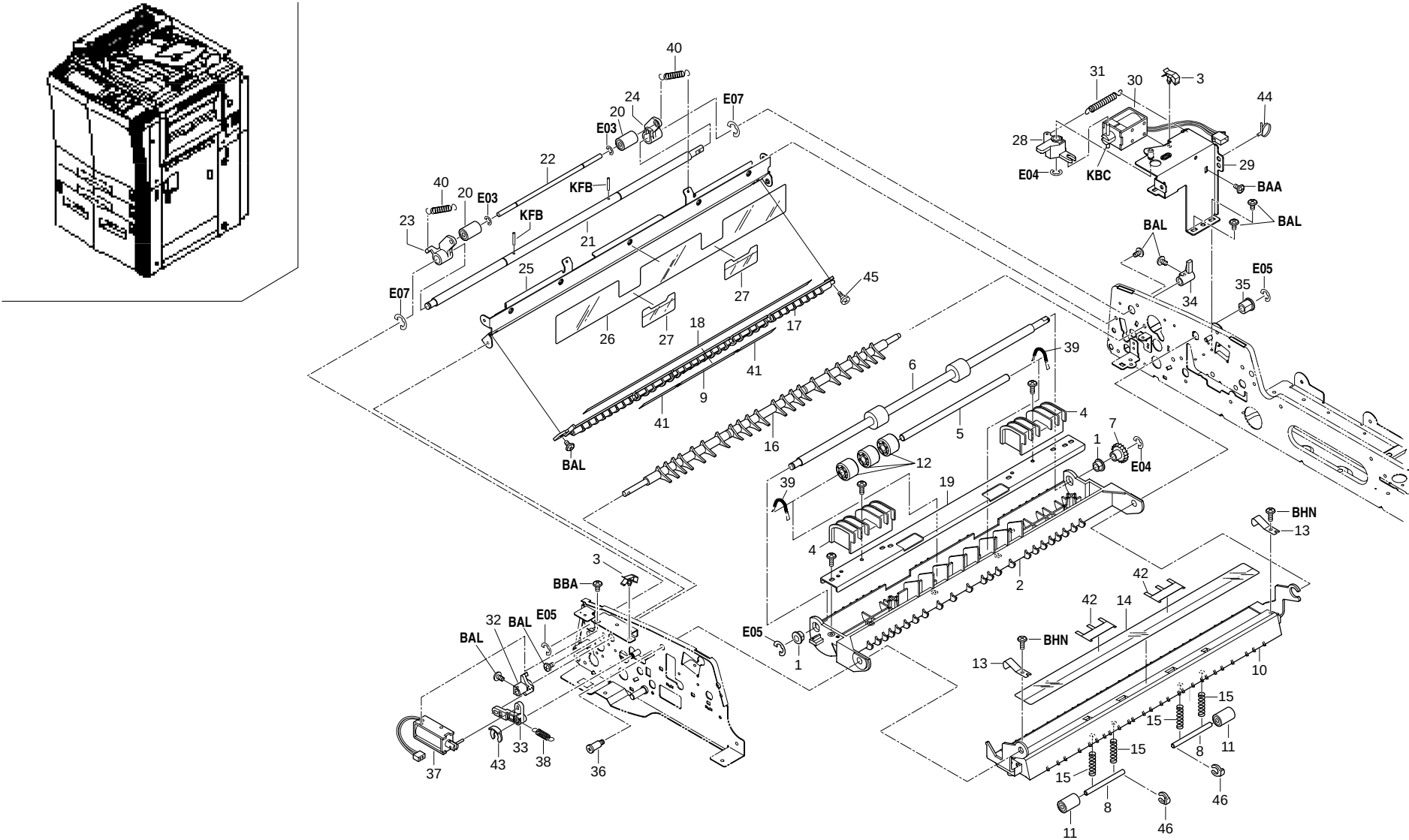
FIG. 35 REVERSING SECTION (DF)
