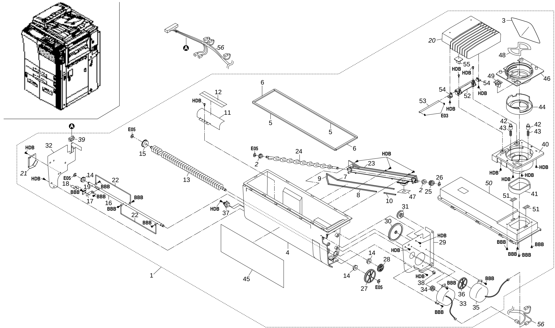
FIG. 29 HOPPER SECTION I
