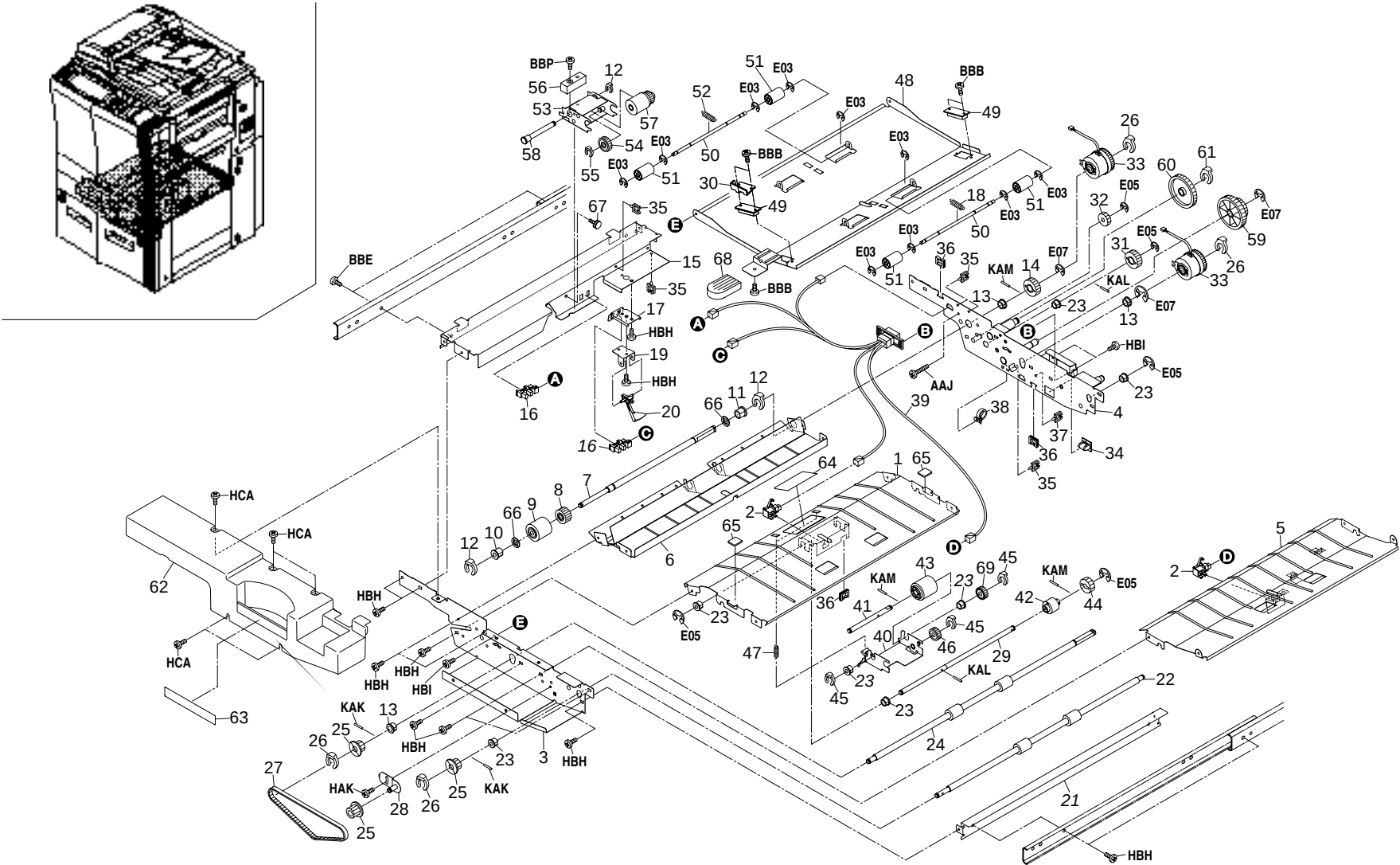
FIG. 6 DECK CONVEYING SECTION
