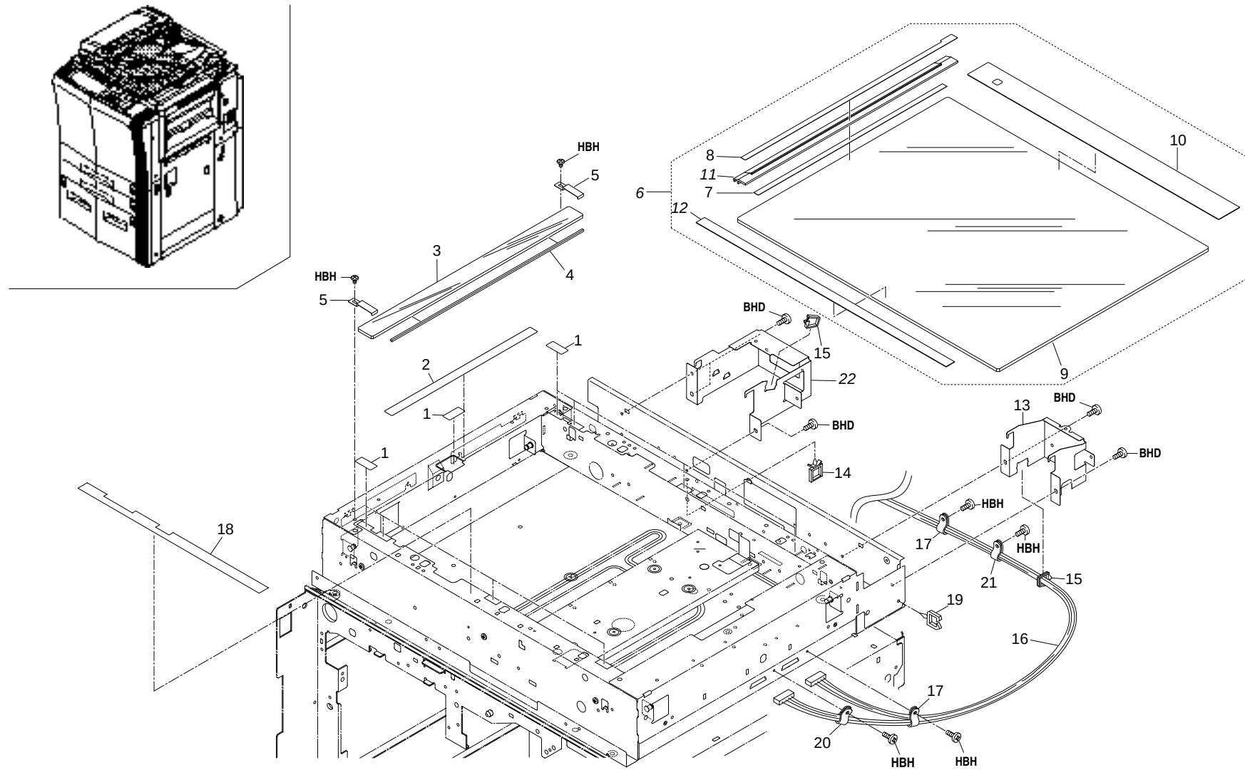
FIG. 11 OPTICAL SECTION II
