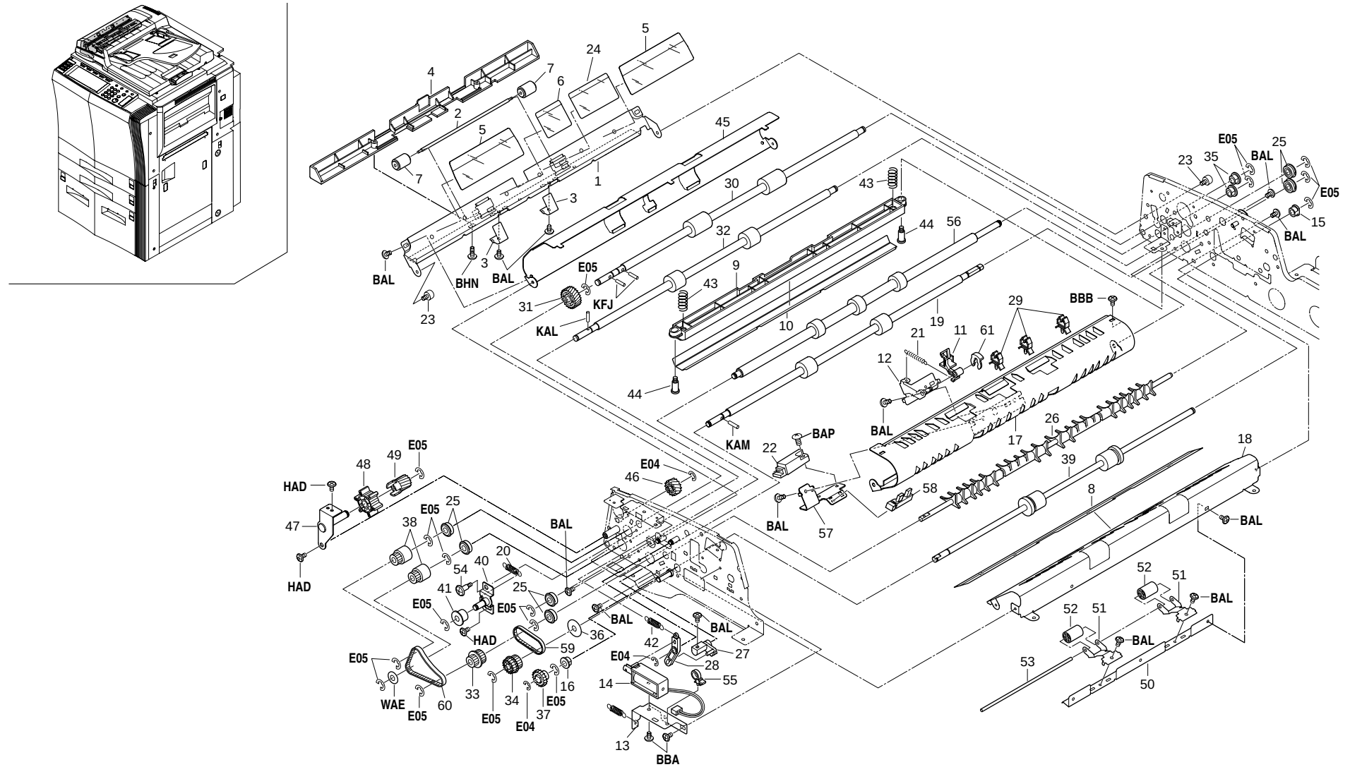
FIG. 36 PAPER EJECT SECTION (DF)
