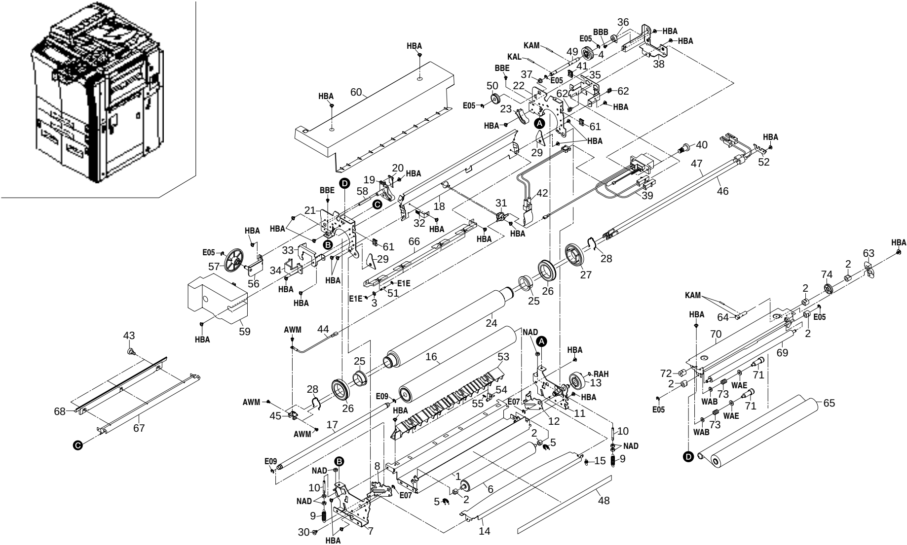
FIG. 19 FIXING SECTION
