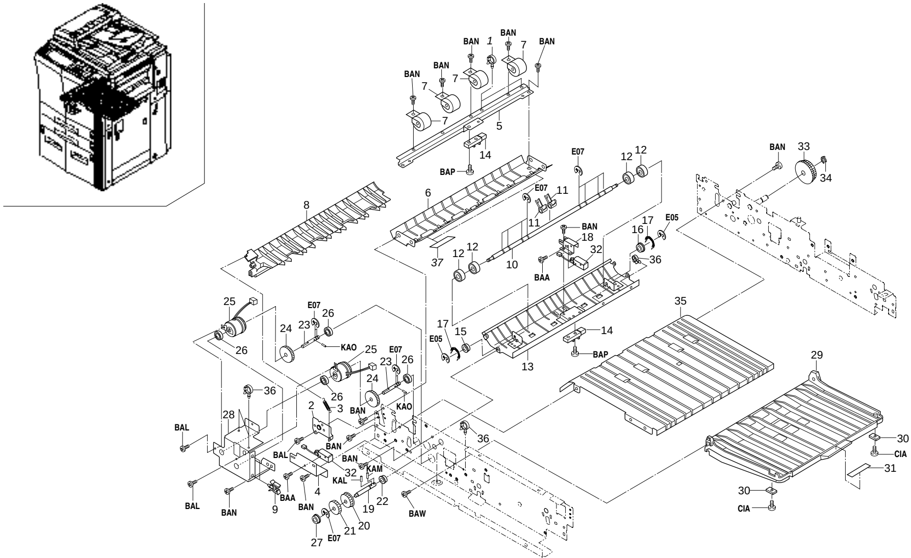
FIG. 24 DUPLEX SECTION II
