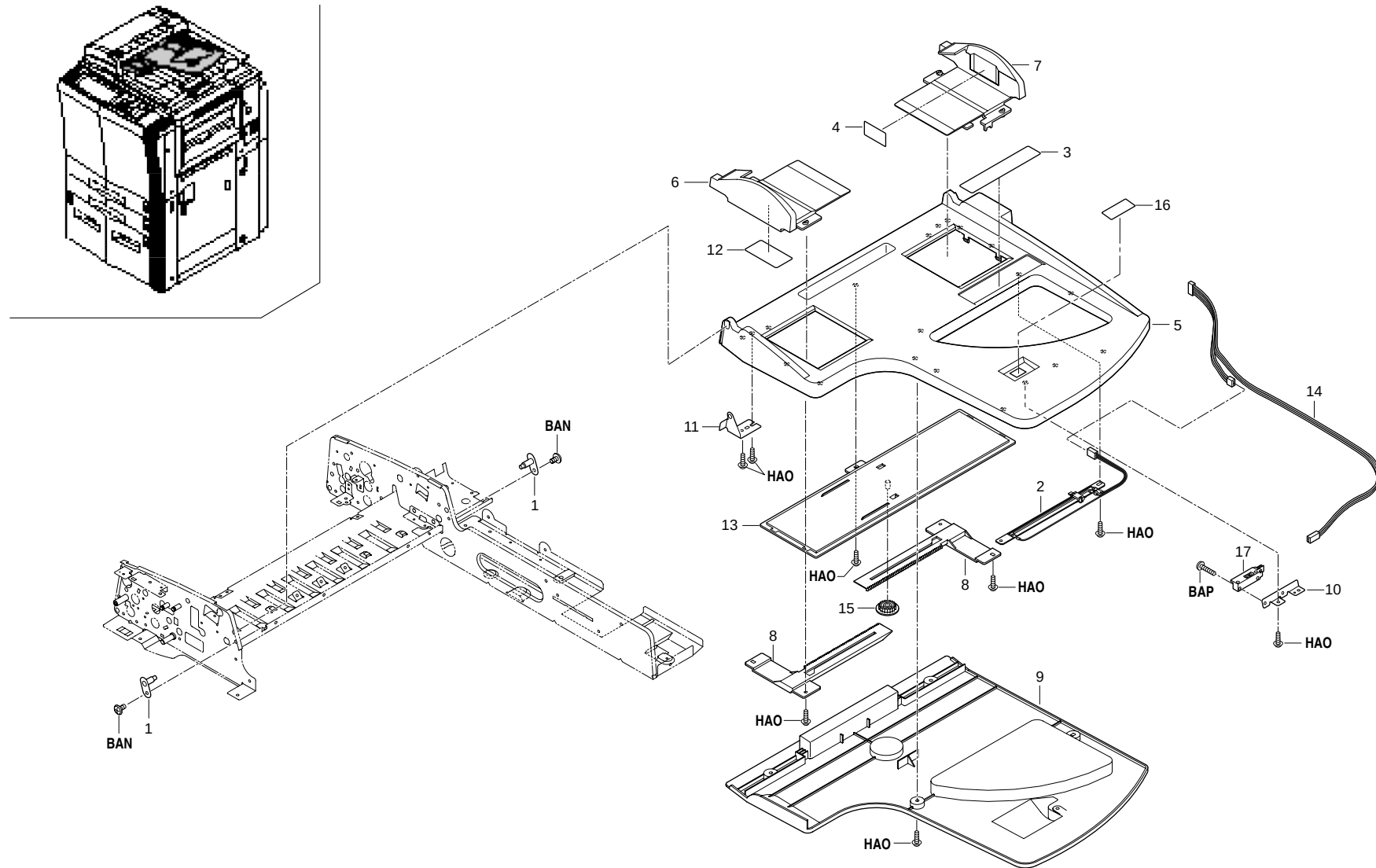
FIG. 33 PAPER FEED-IN SECTION (DF)
