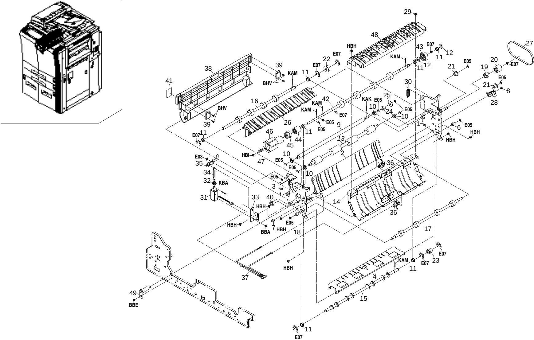
FIG. 18 CONVEYING SECTION III
