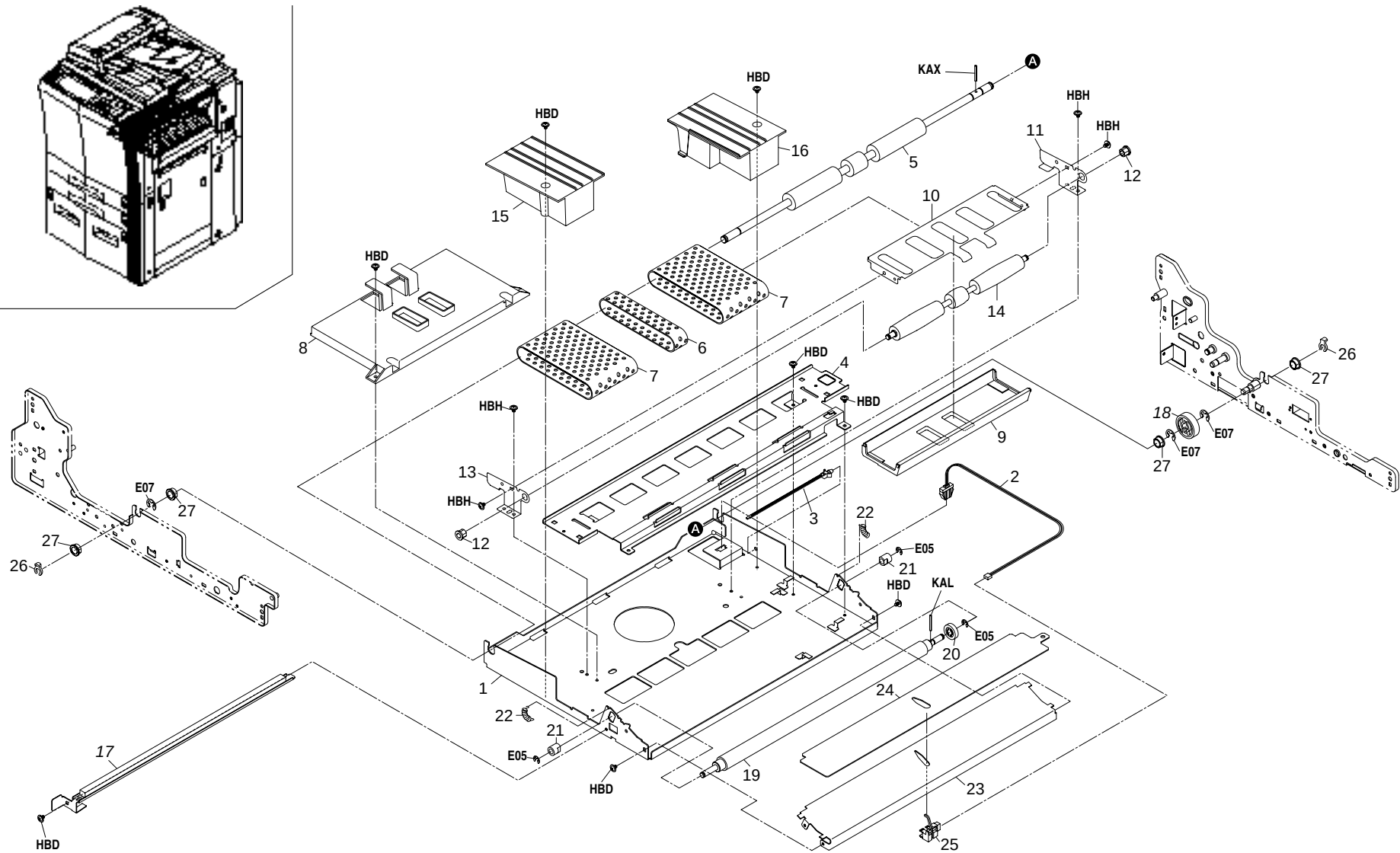
FIG. 17 CONVEYING SECTION II
