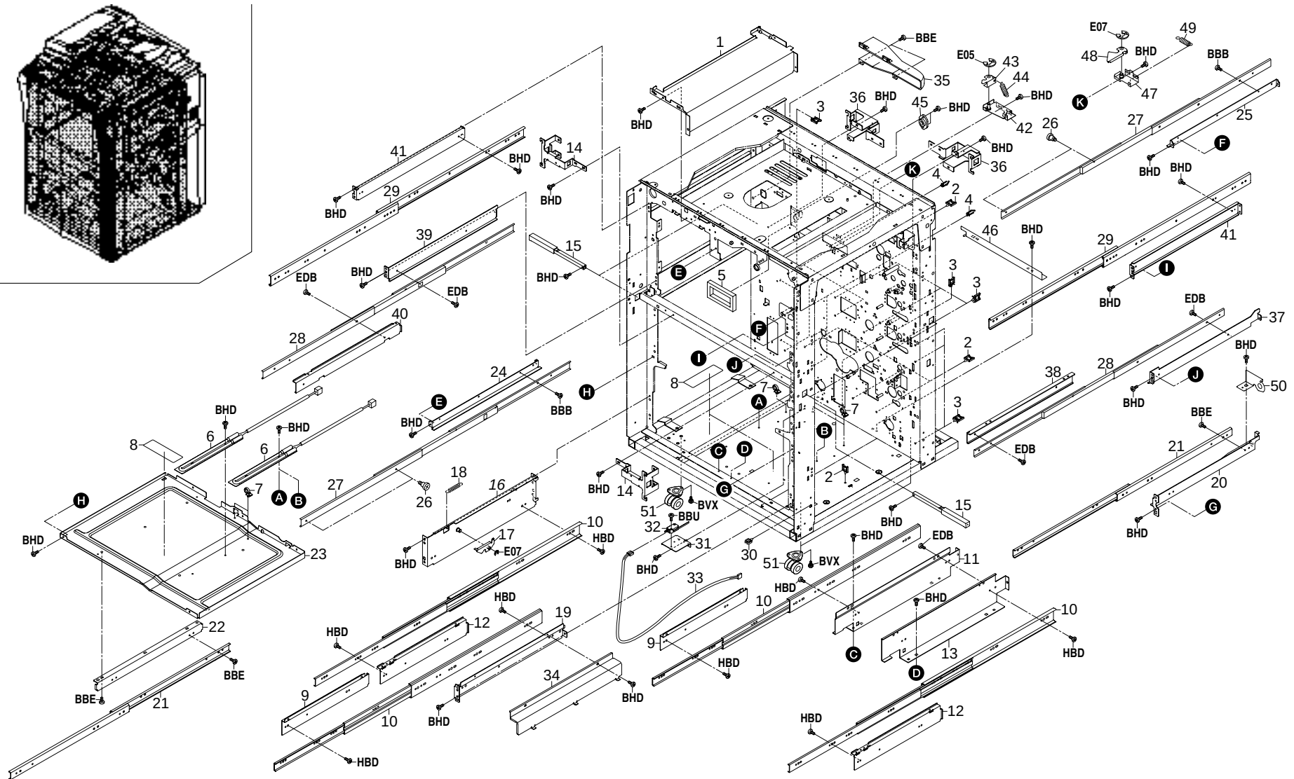
FIG. 2 FRAME SECTION
