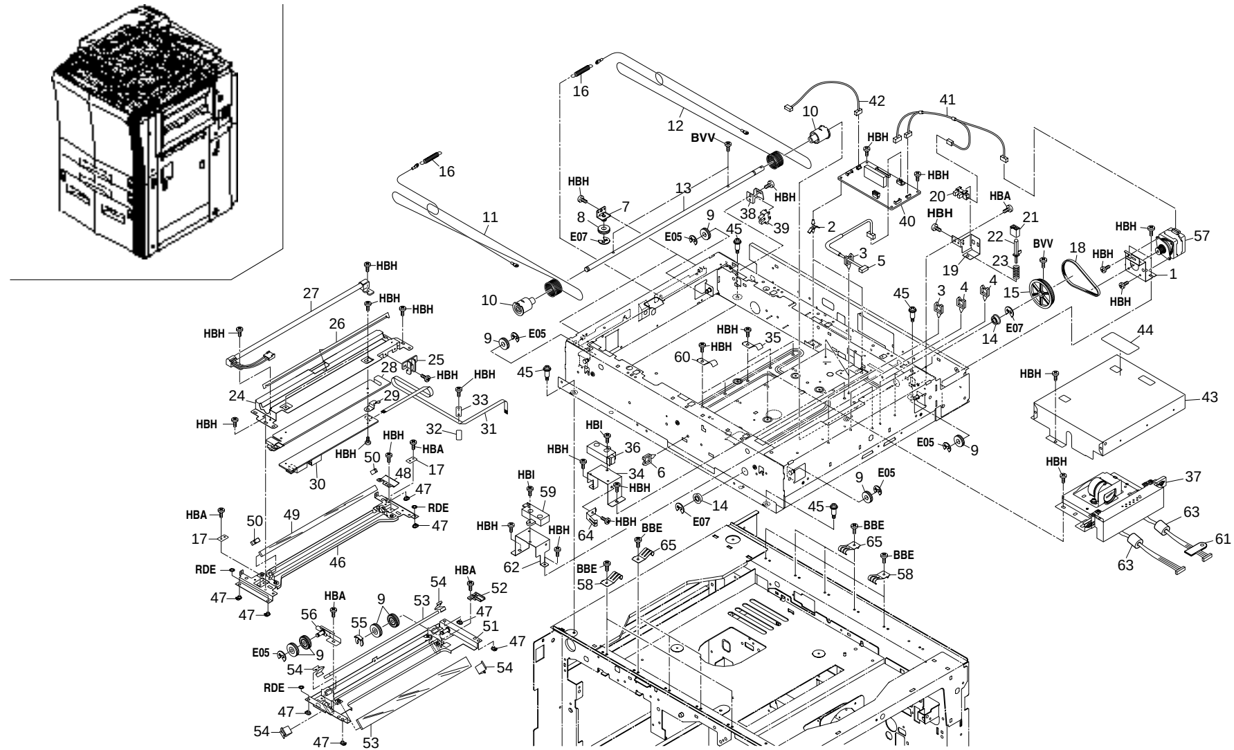
FIG. 10 OPTICAL SECTION I
