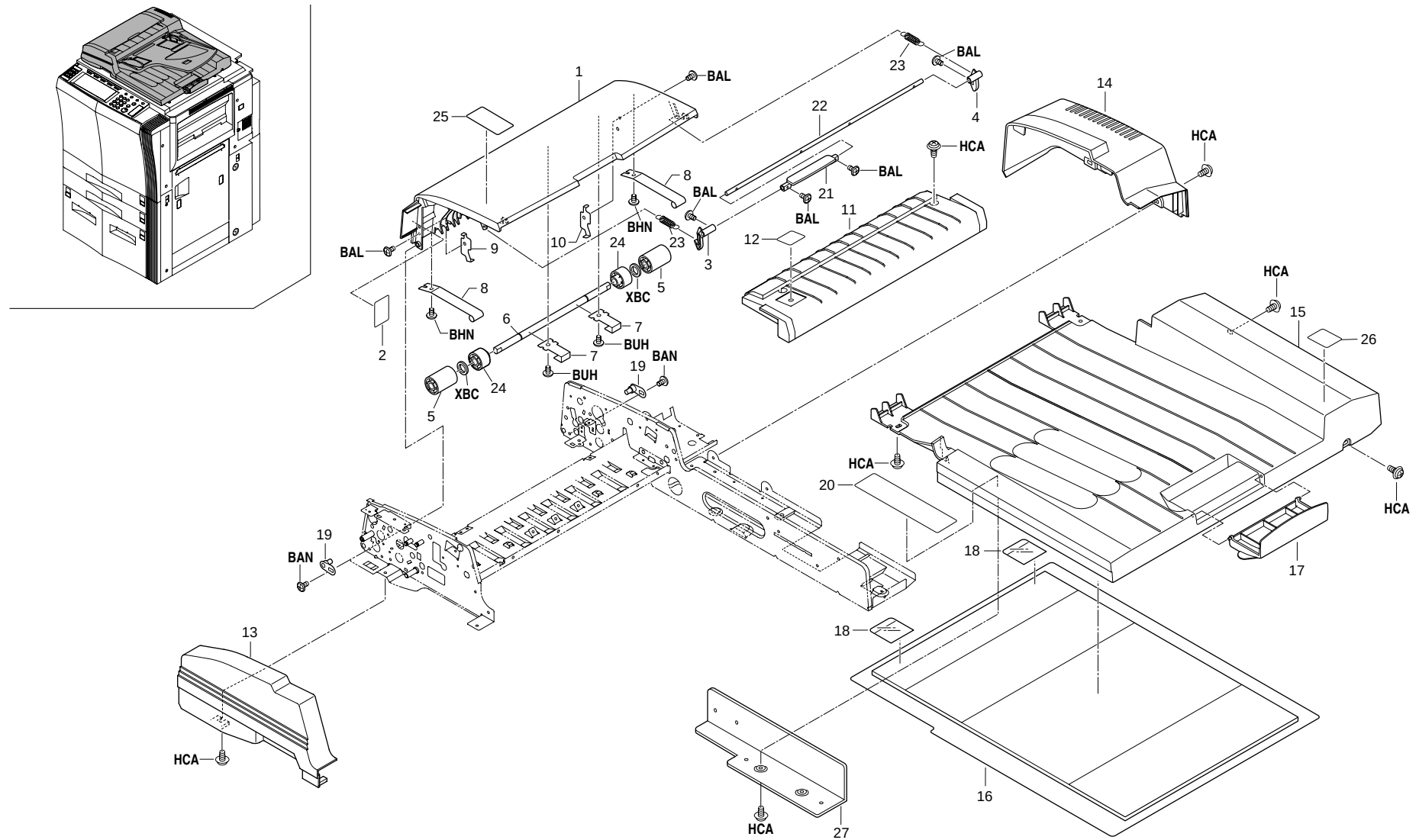
FIG. 31 COVER SECTION (DF)
