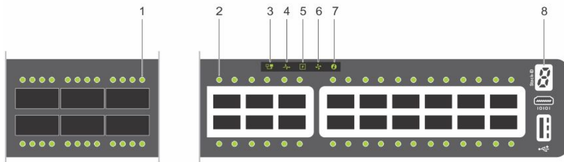
Figure 13. S4148U-ON switch I/O-side LEDs
