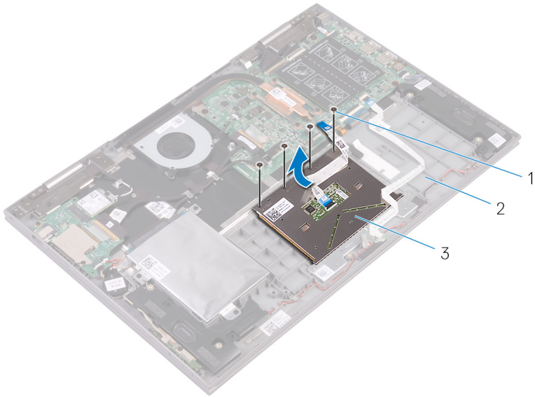
Figure 16. Removing the touchpad
