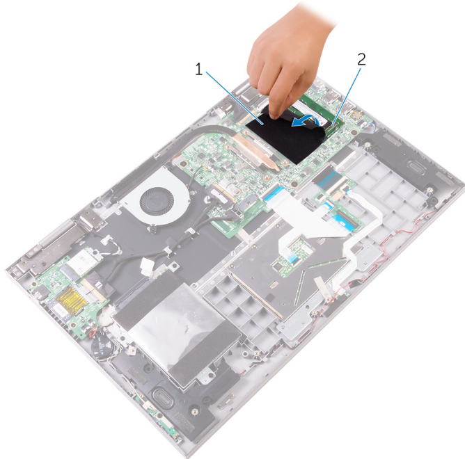
Figure 4. Removing the memory modules
