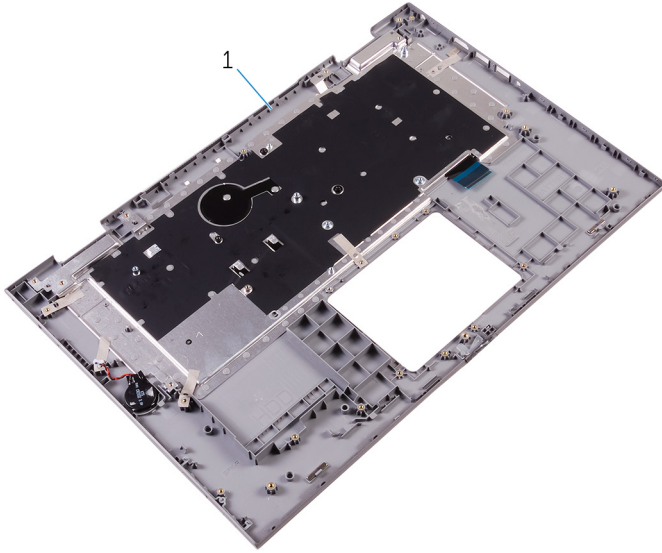
Figure 30. Removing the palm rest and keyboard assembly
