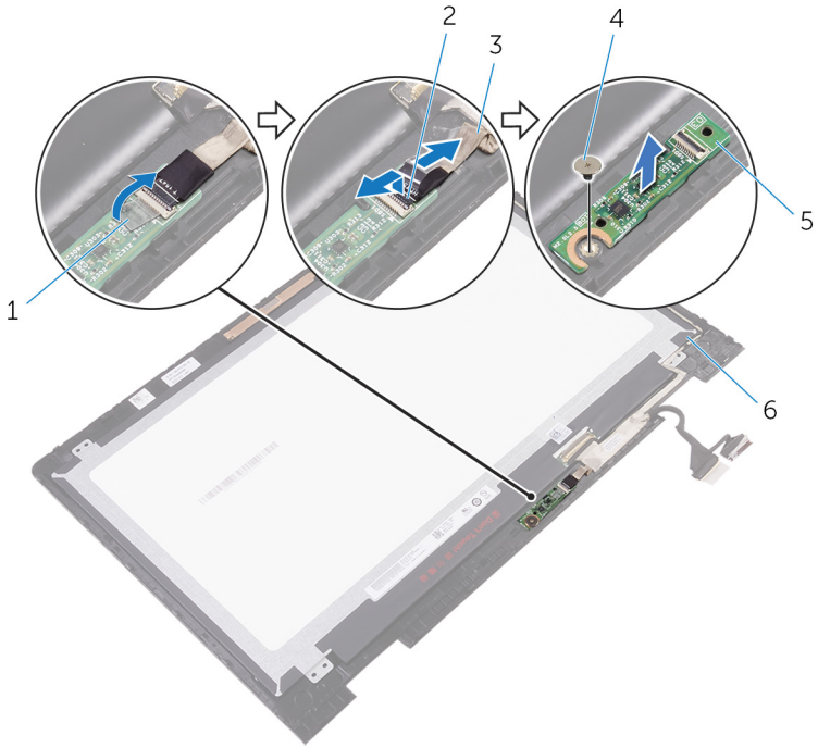
Figure 37. Removing the sensor board
