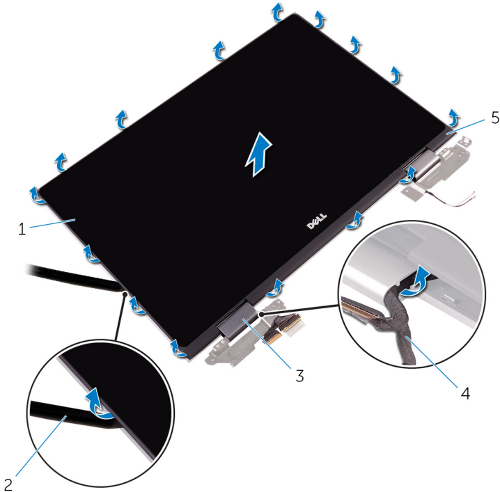
Figure 31. Removing the display back cover and antenna assembly
