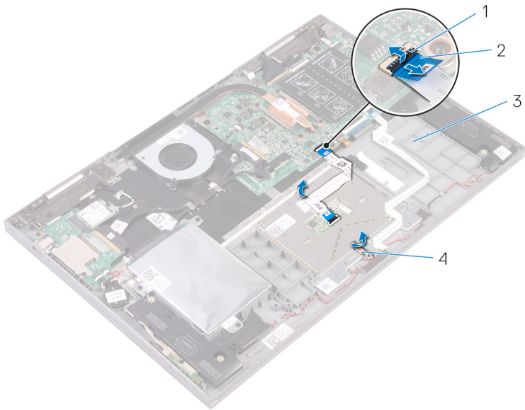
Figure 15. Disconnecting the touchpad cable
