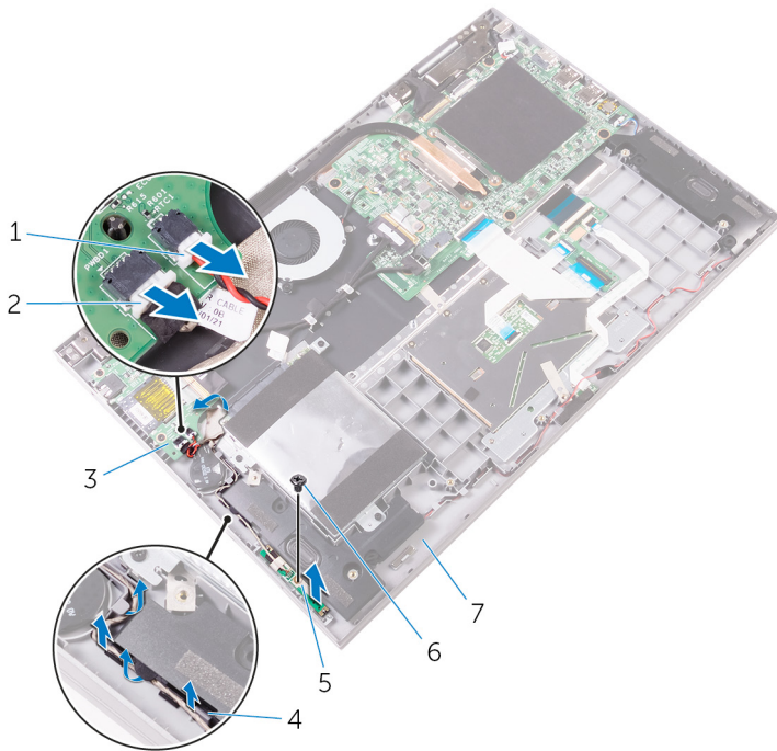
Figure 22. Removing the power and volume-buttons board
