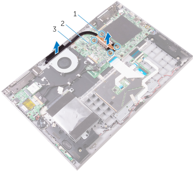
Figure 20. Removing the heat sink
