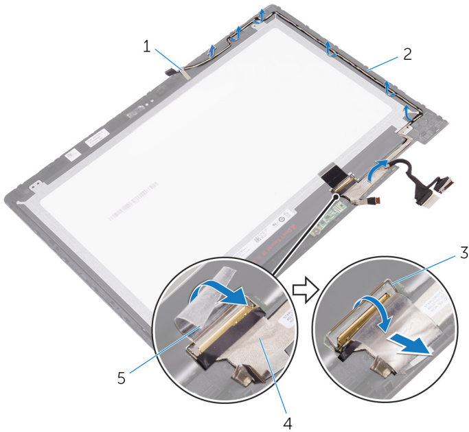
Figure 34. Removing the display cable
