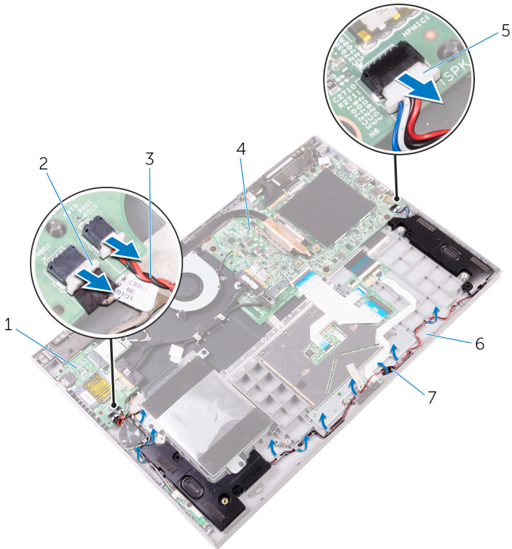
Figure 17. Removing the speakers
