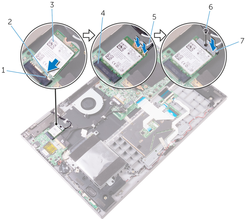
Figure 13. Replacing the wireless card
