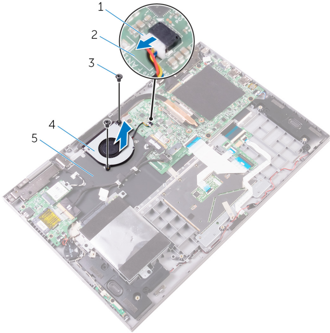
Figure 19. Removing the fan
