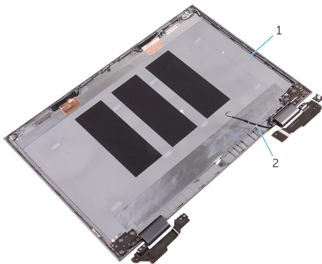
Figure 35. Display back-cover and antenna assembly
