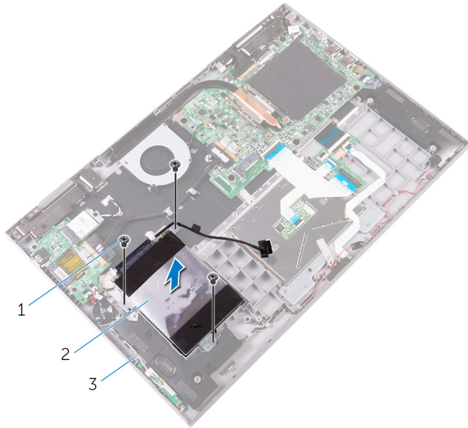
Figure 8. Removing the hard-drive assembly
