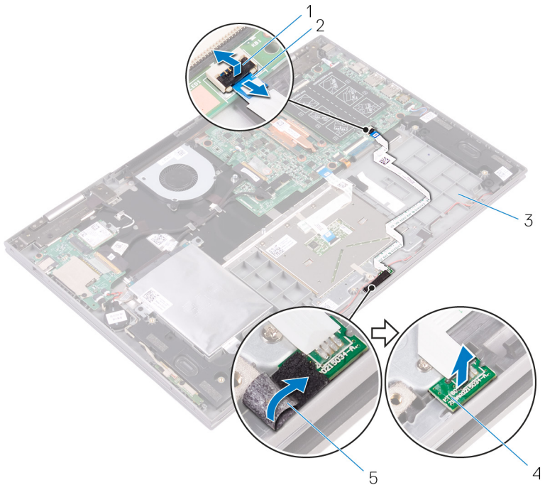
Figure 14. Removing the status-light board
