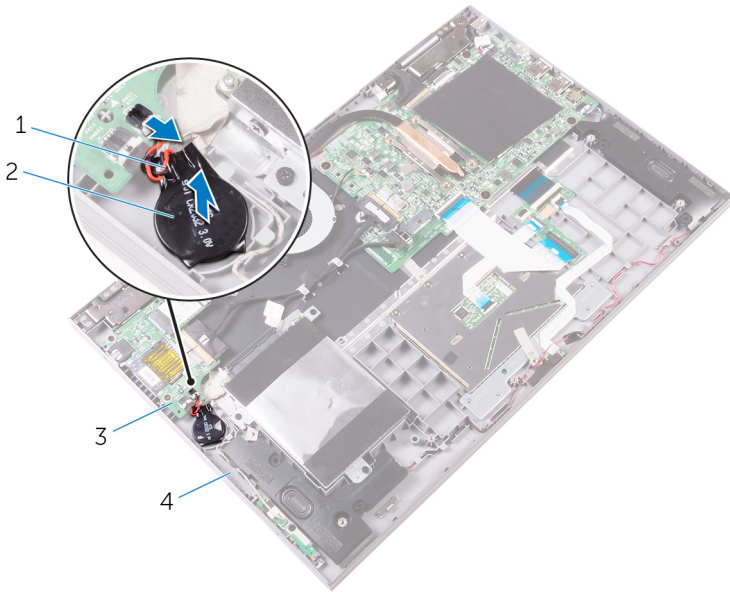
Figure 11. Removing the coin-cell battery
