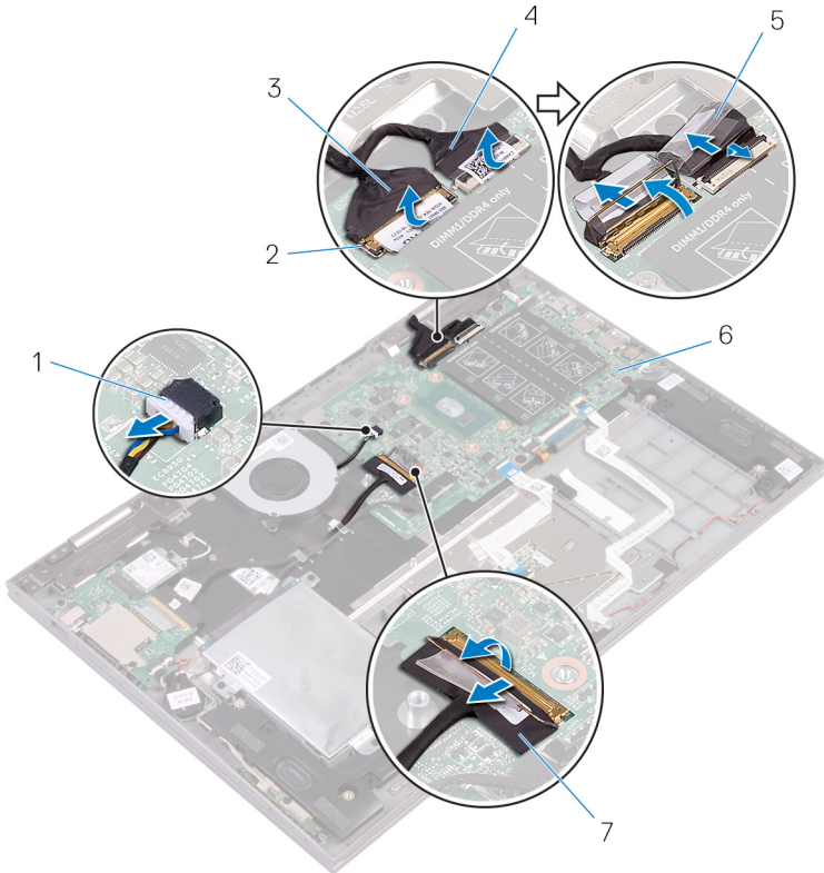
Figure 25. Removing the system board cables
