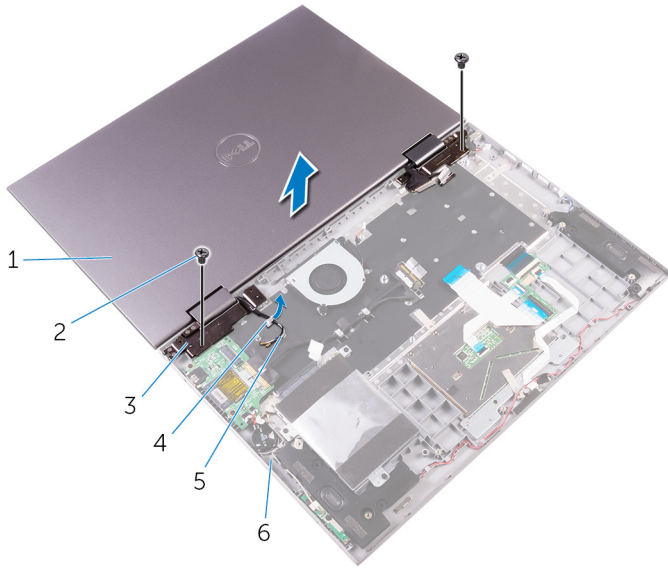
Figure 29. Removing the display assembly
