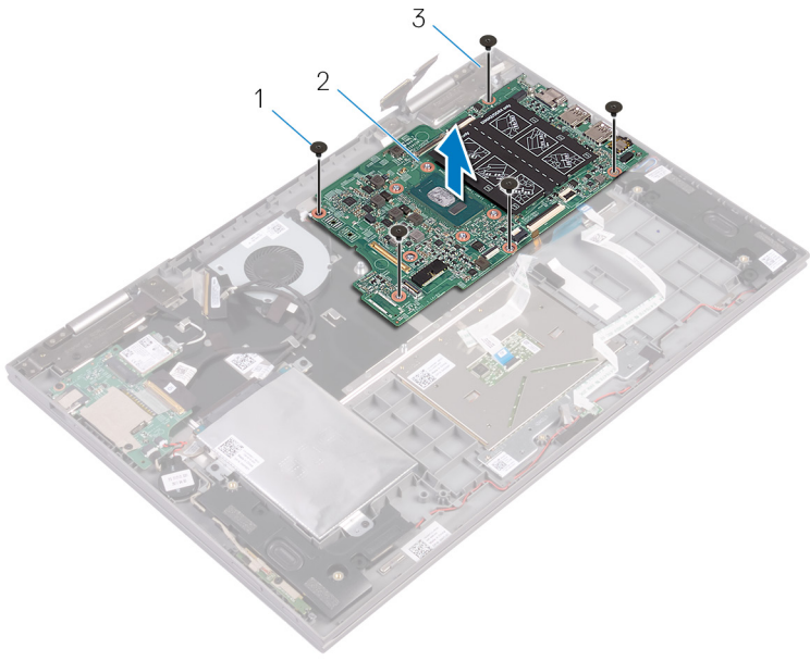
Figure 27. Removing the system board
