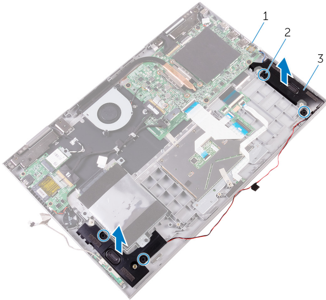
Figure 18. Removing the speakers
