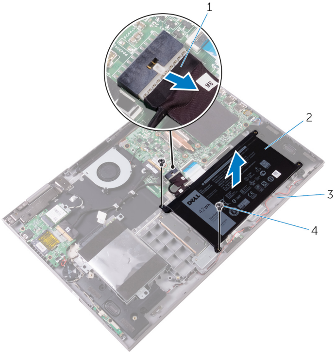
Figure 3. Removing the battery
