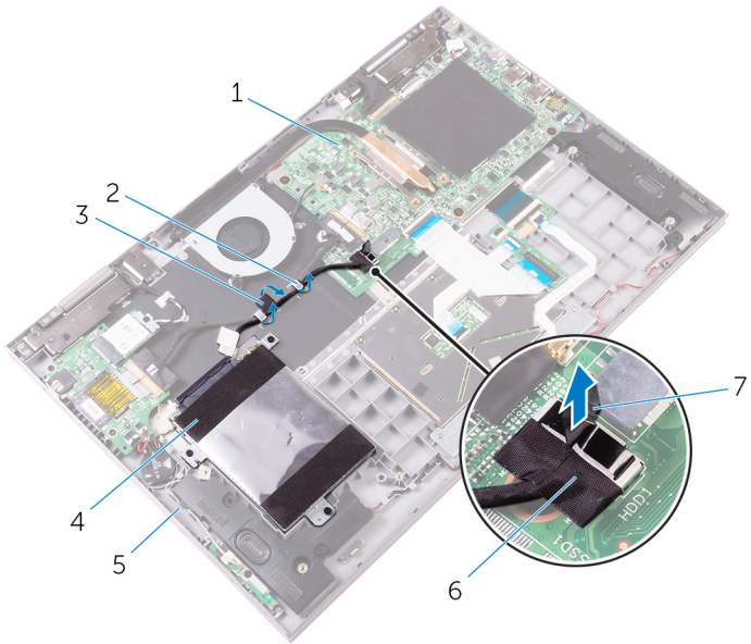
Figure 7. Removing the hard-drive assembly
