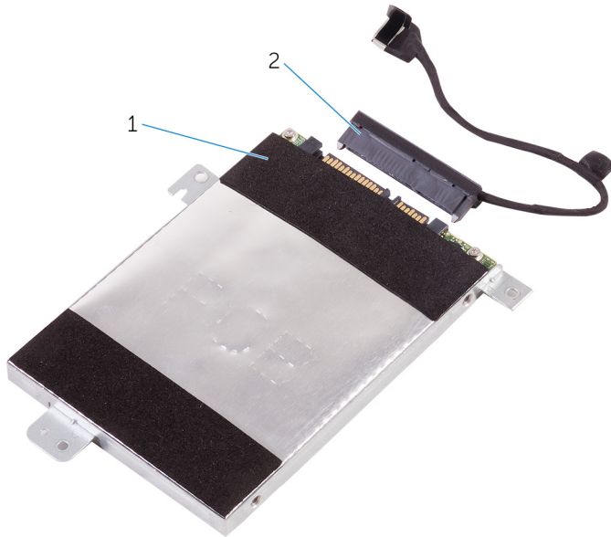
Figure 9. Disconnecting the interposer
