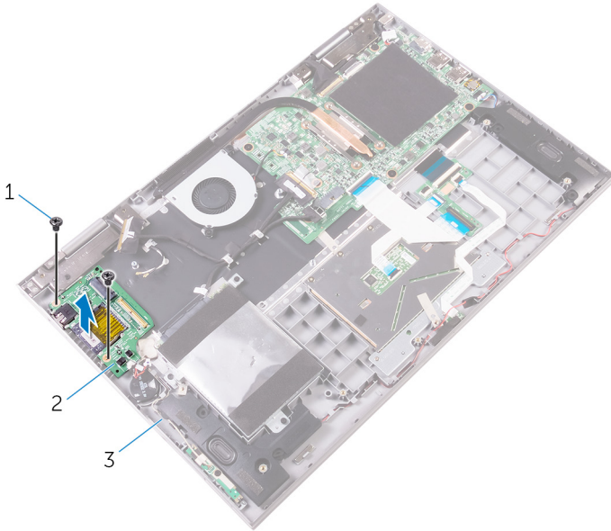
Figure 24. Removing the I/O board
