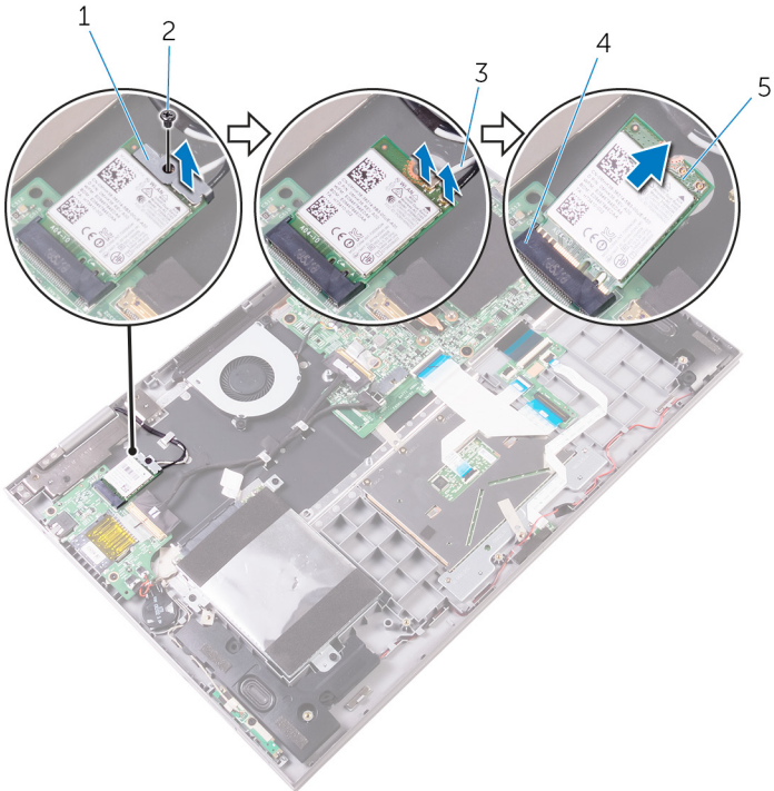
Figure 12. Removing the wireless card
