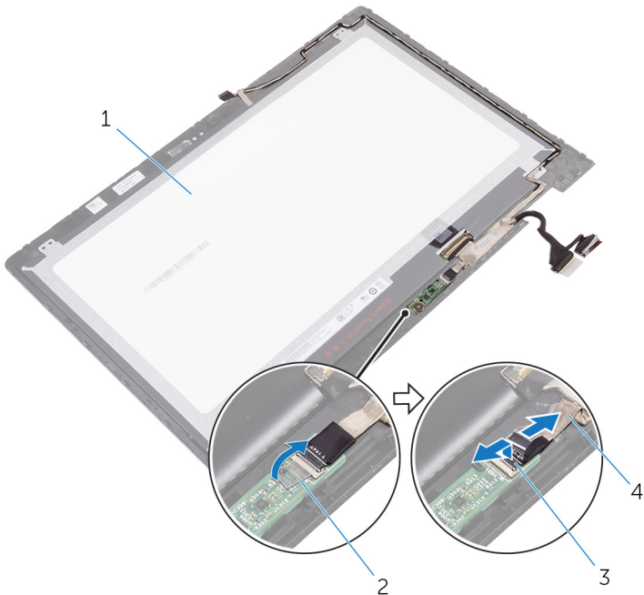
Figure 33. Removing the sensor-board cable
