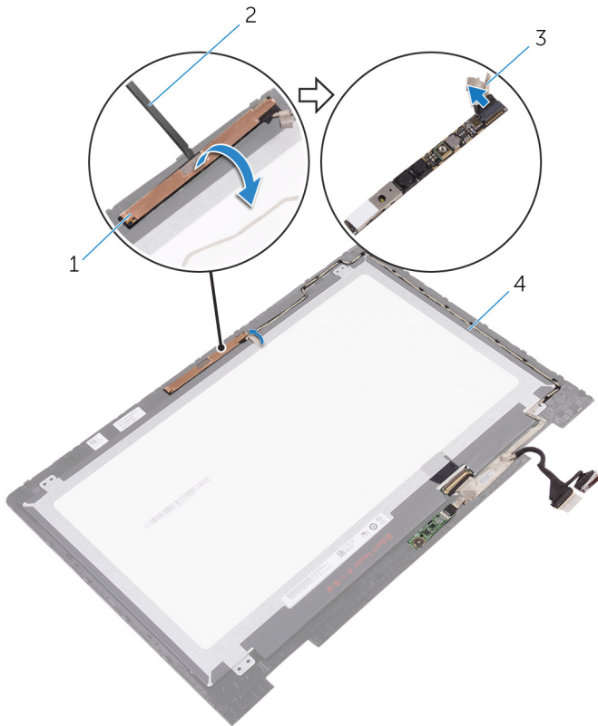
Figure 36. Removing the camera
