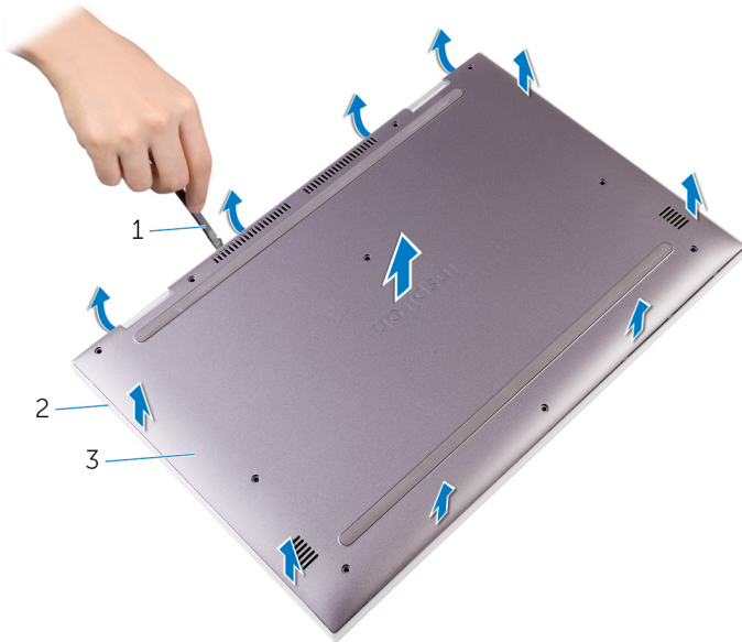
Figure 2. Removing the base cover
