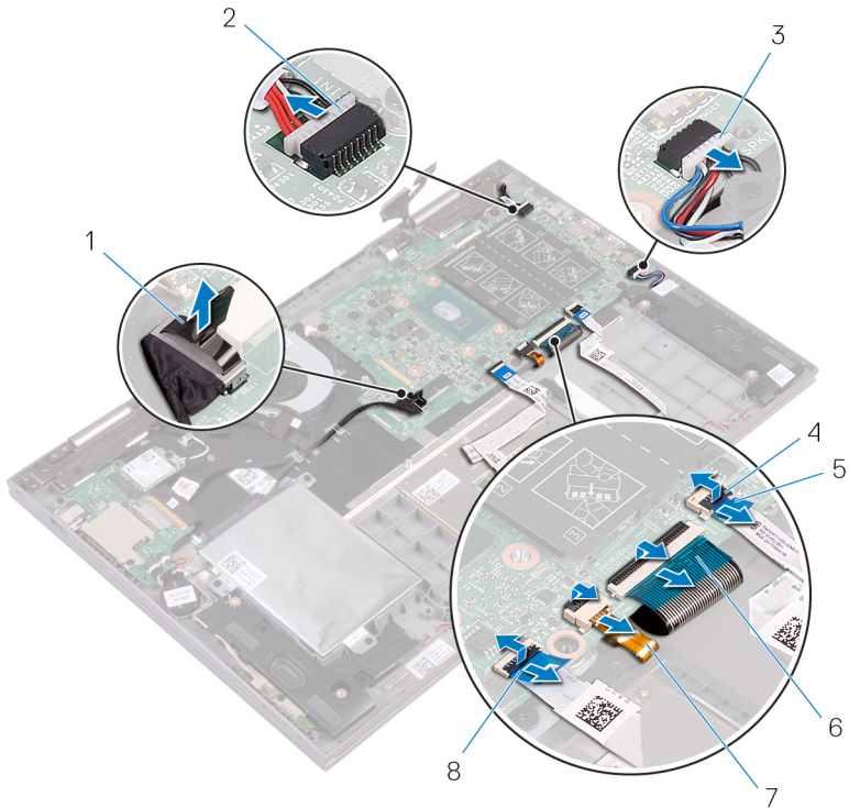
Figure 26. Removing the system board cables
