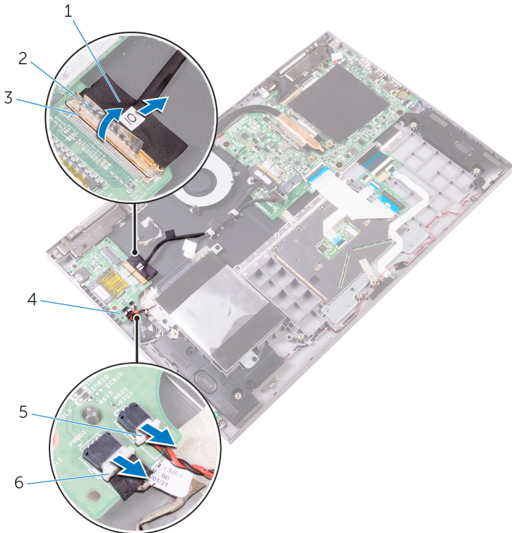
Figure 23. Removing the I/O board
