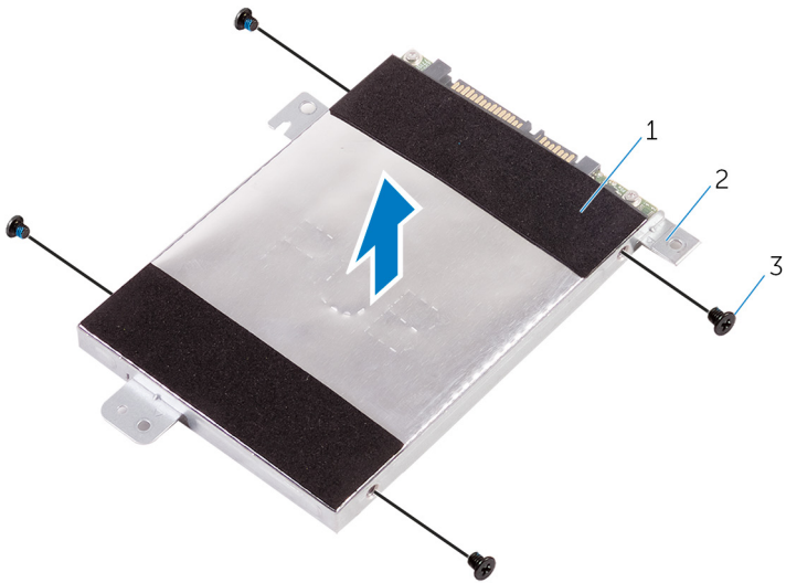
Figure 10. Removing the hard-drive bracket
