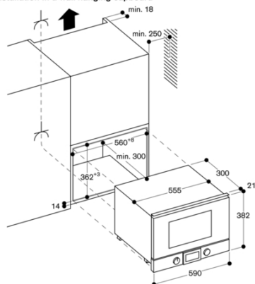
Installation in a wall-hanging cupboard
