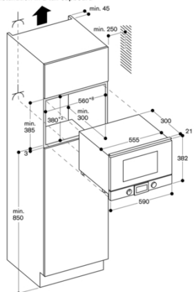
Installation in a tall cupboard
