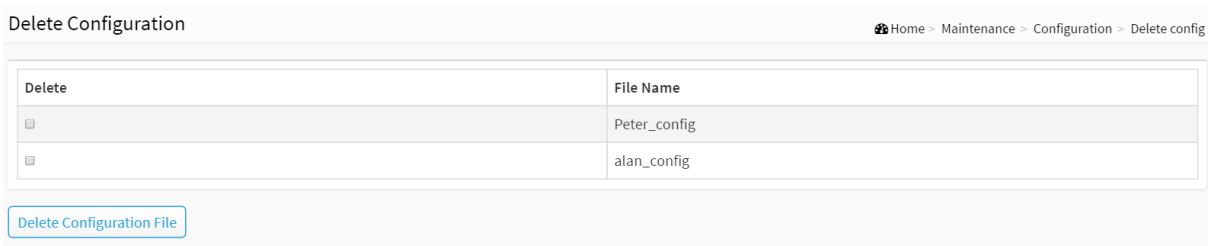
Figure 17-1.5: Delete Configuration
