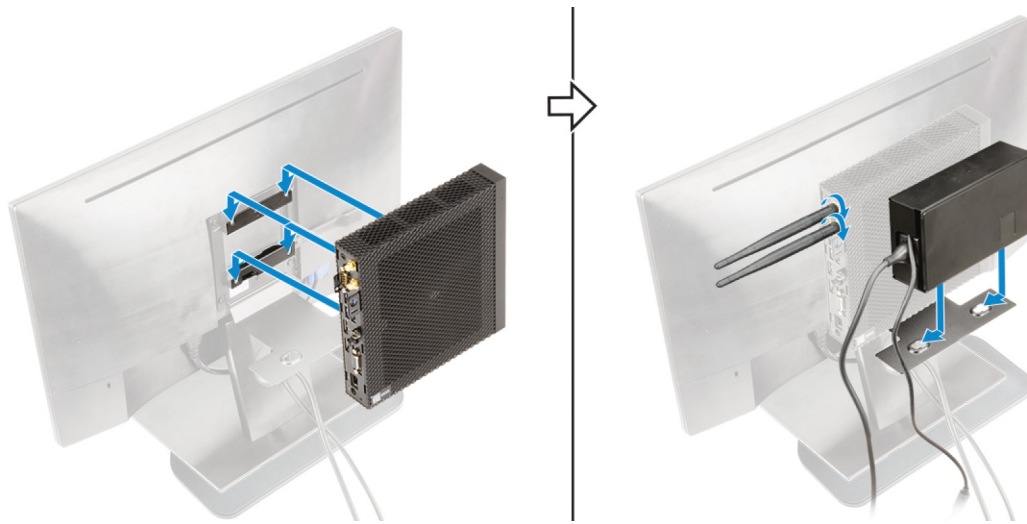
Figure 8. Attaching the thin client and adapter box
