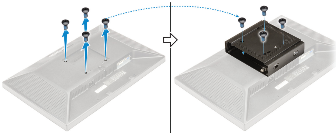
Figure 20. Attaching the dual VESA metal bracket to the display
