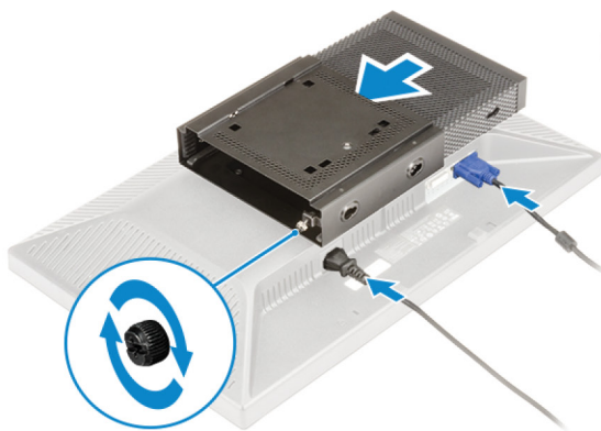
Figure 23. Mounting the thin client and adapter box
