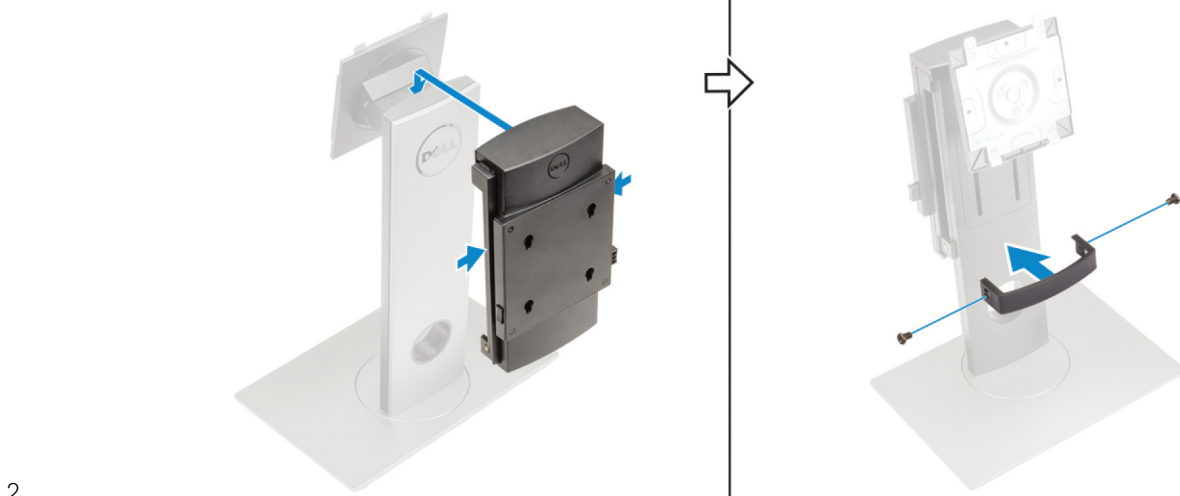
Figure 14. Engaging the P/U mount into the stand with the pocket clip
