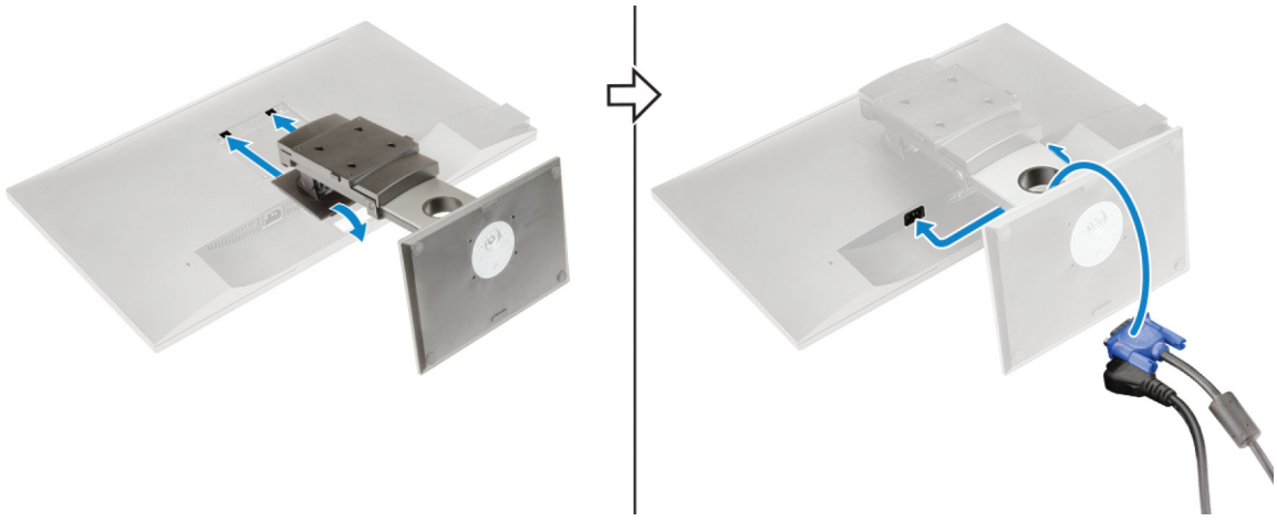
Figure 15. Assembling the stand with the P/U mount to the display
