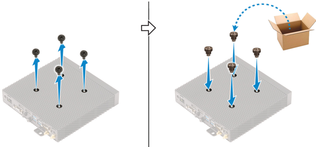
Figure 16. Tightening the shoulder screws
