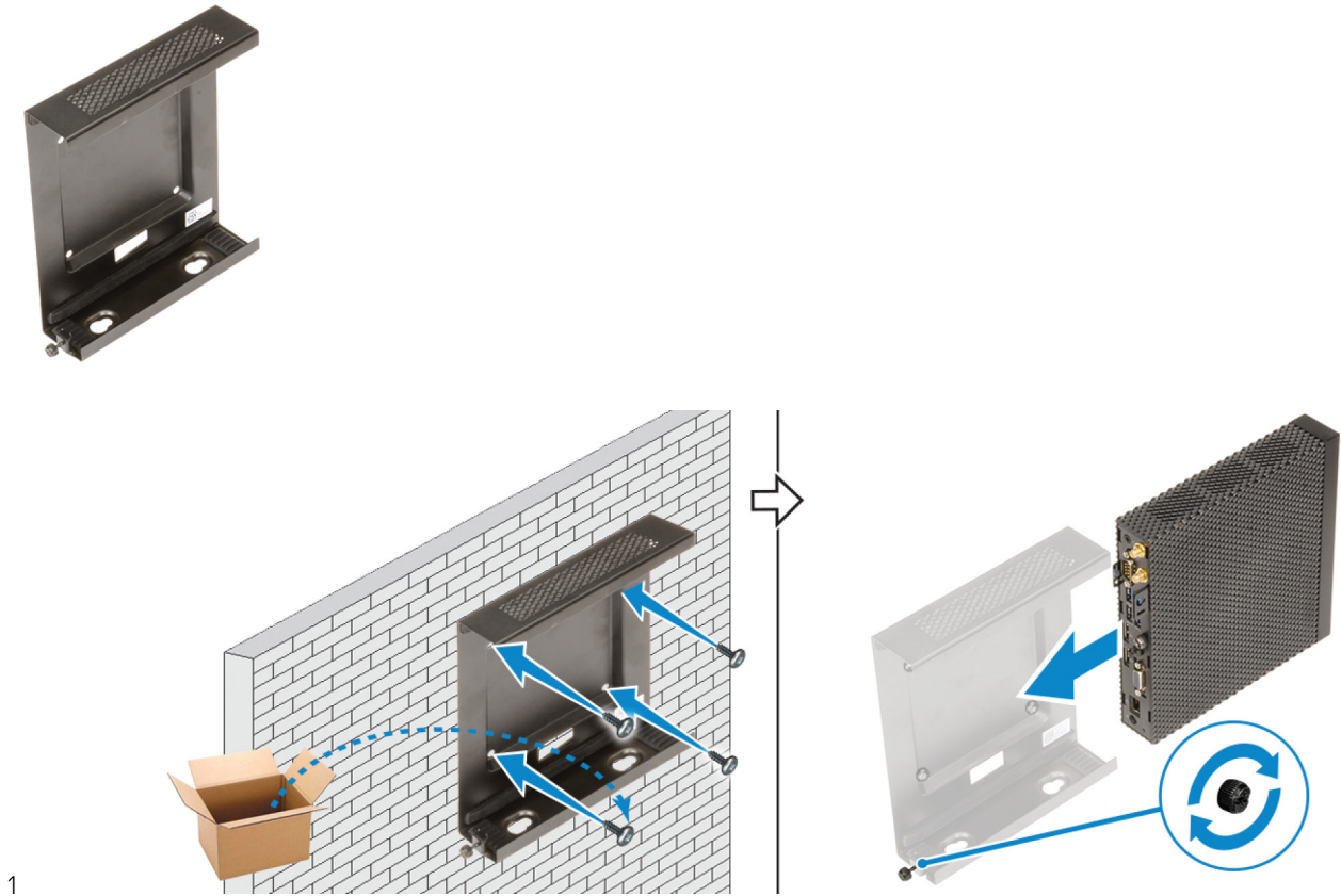
Figure 10. Insert the thin client into the metal bracket
