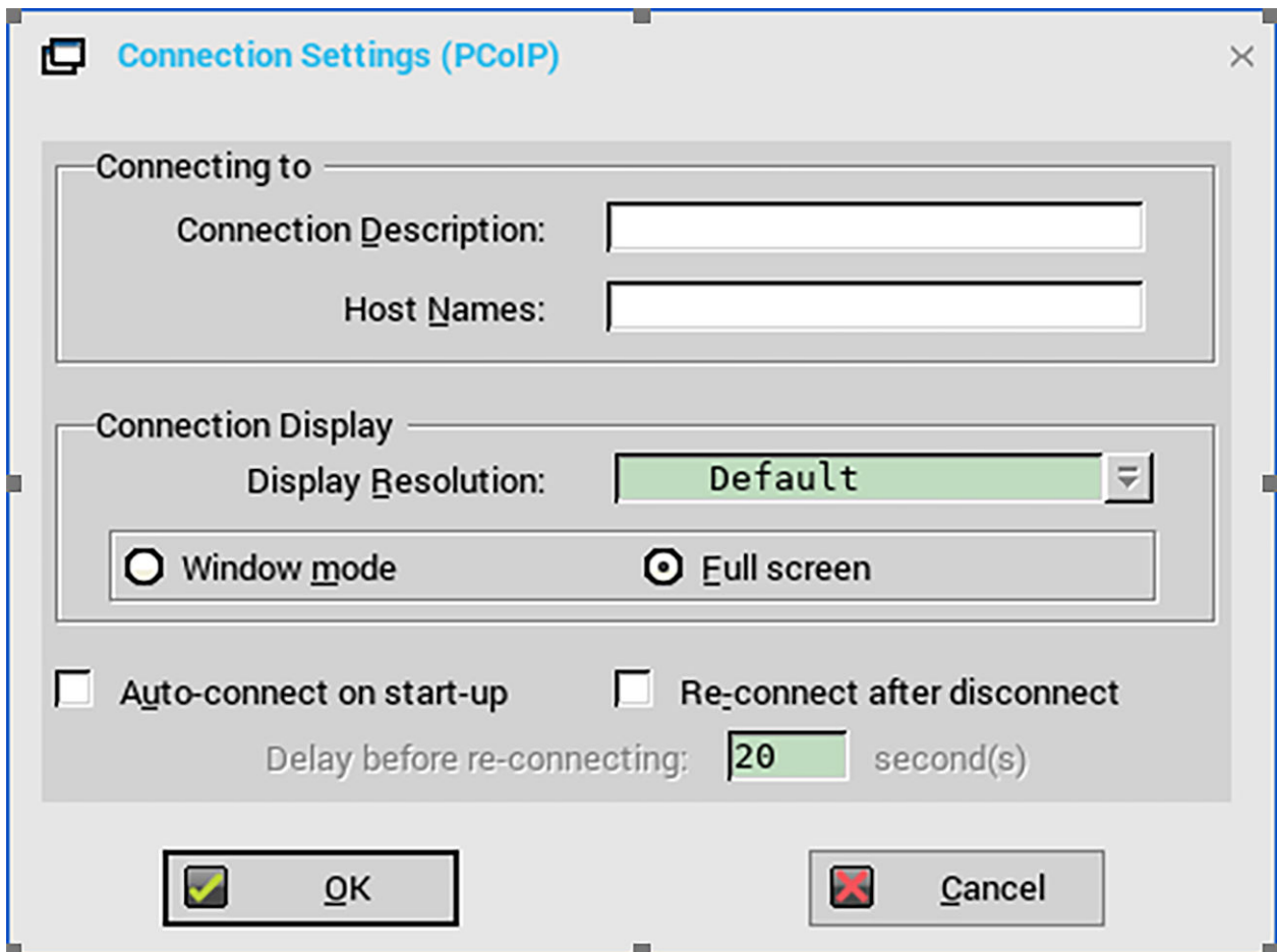
Figure 23. Connection Settings - PCoIP
