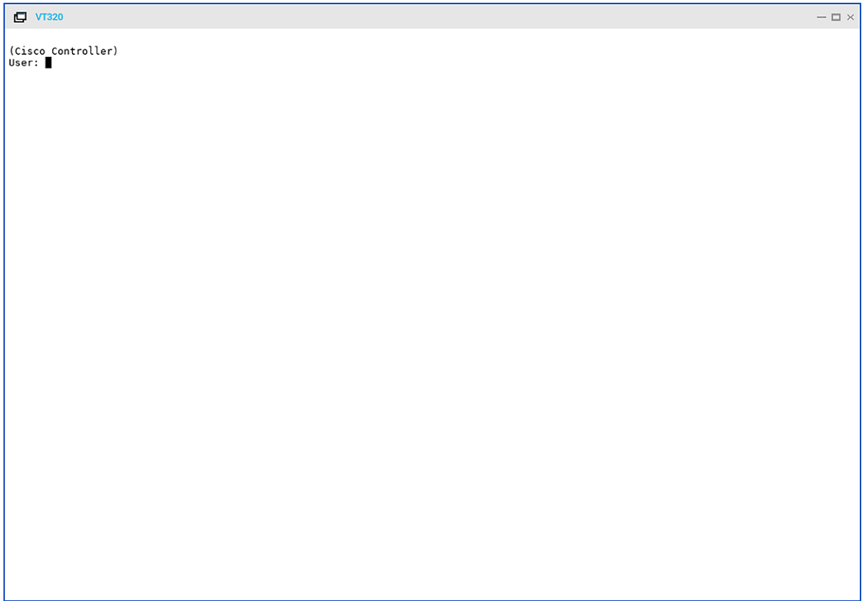
Figure 44. Telnet window
