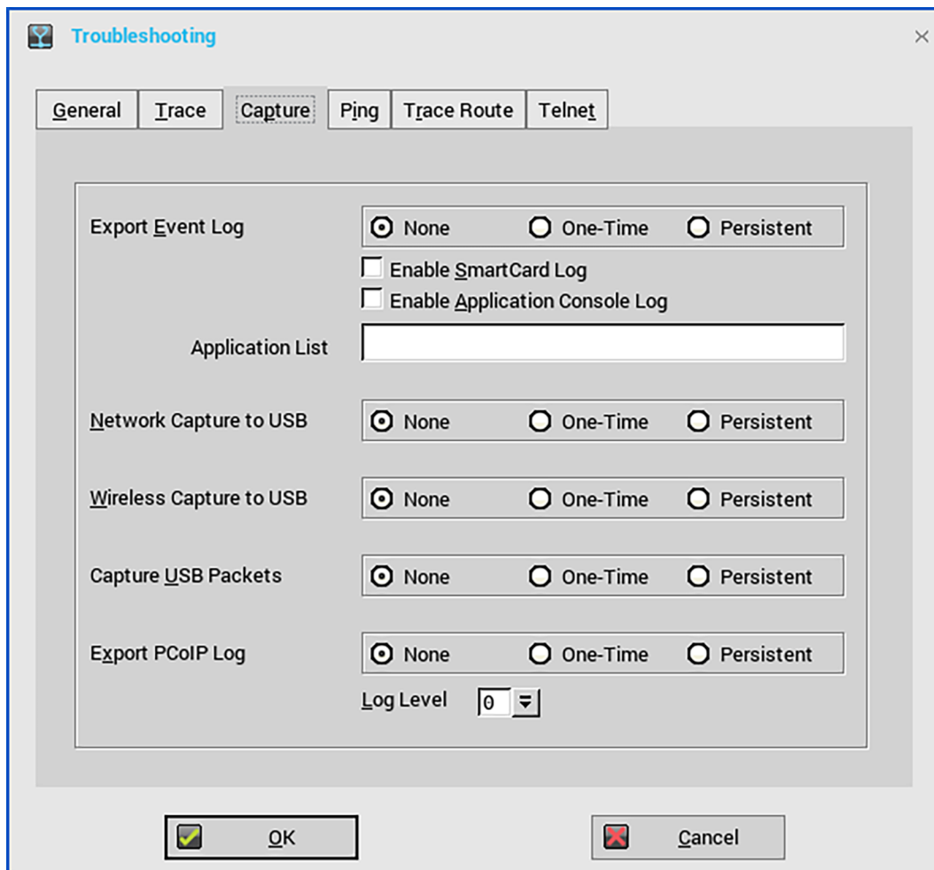
Figure 40. Capture
