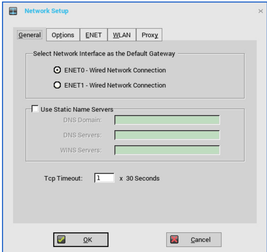
Figure 4. General settings with ENET0 and ENET1
