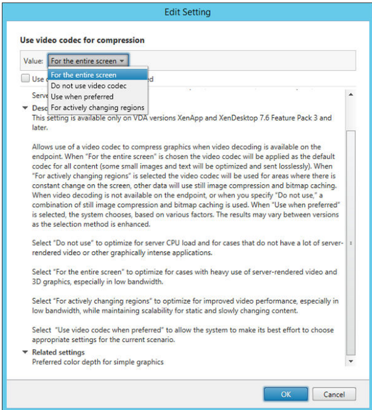
Figure 18. Use video codec for compression setting
