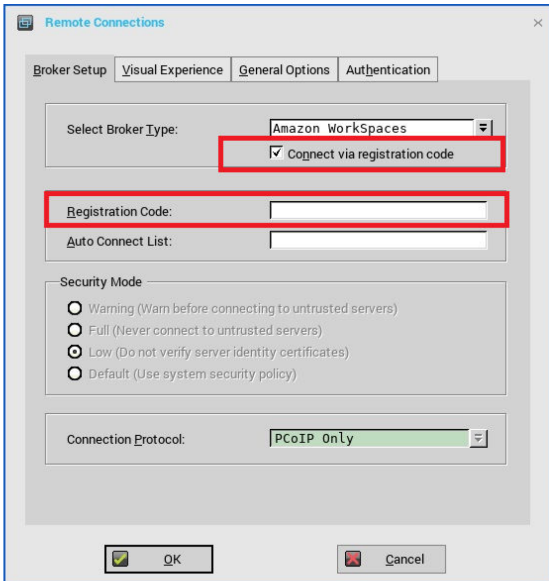
Figure 29. Amazon WorkSpaces with the Registration Code field
