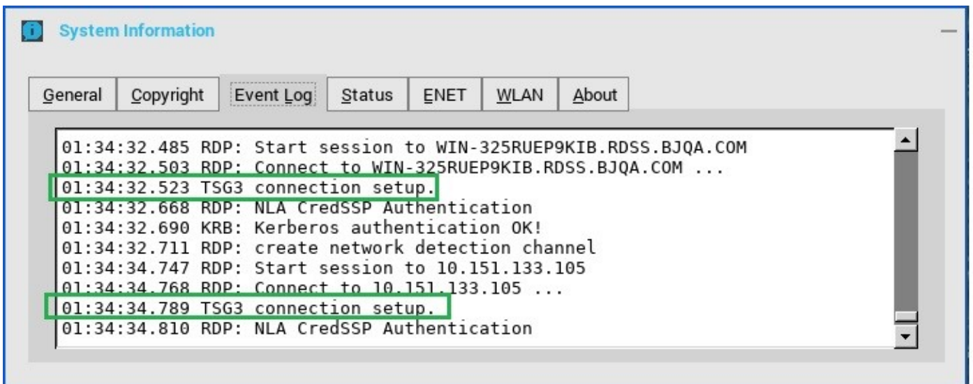
Figure 26. Event log tab
