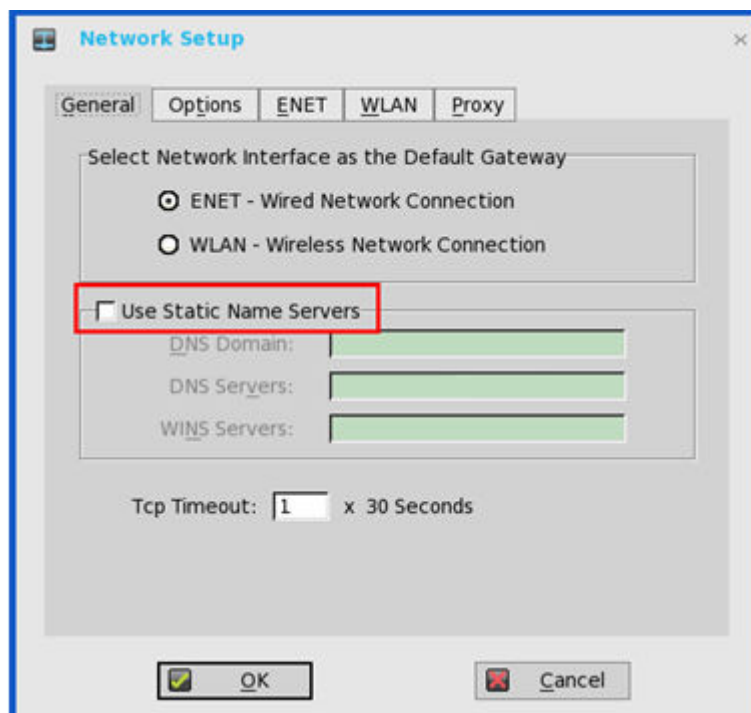
Figure 3. General settings with ENET and WLAN
