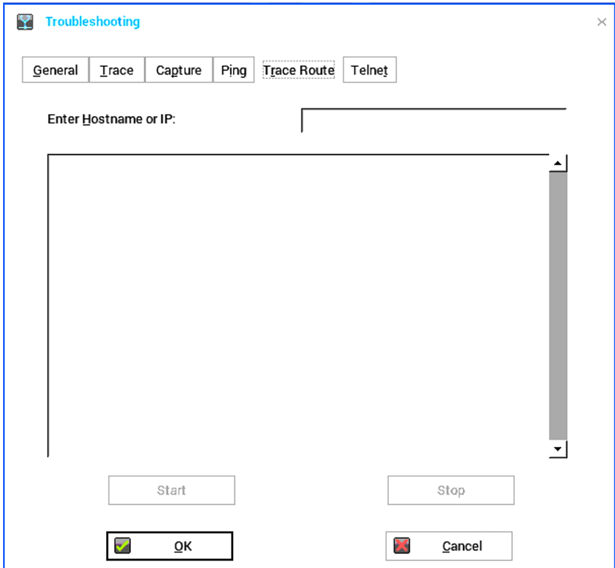
Figure 42. Trace route
