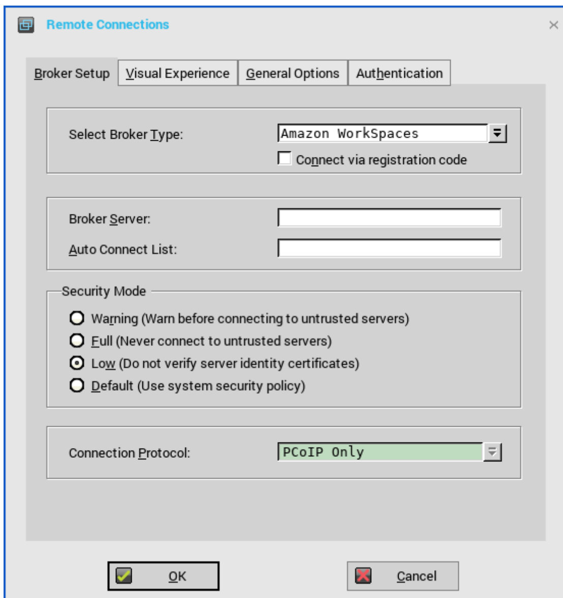
Figure 28. Amazon WorkSpaces
