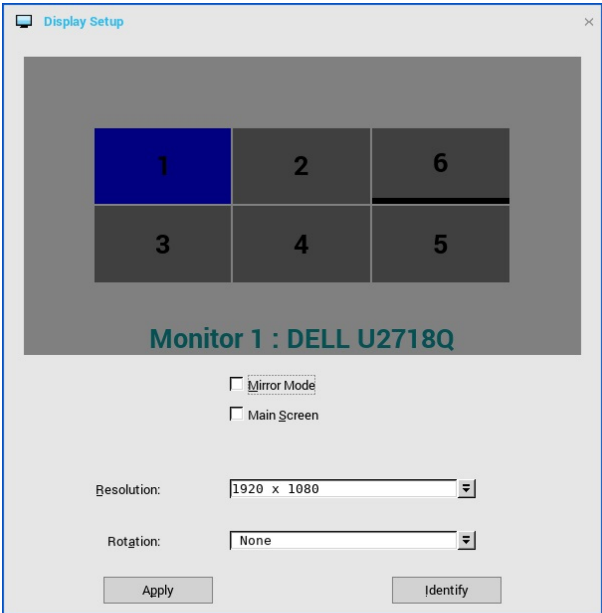
Figure 34. Display settings
