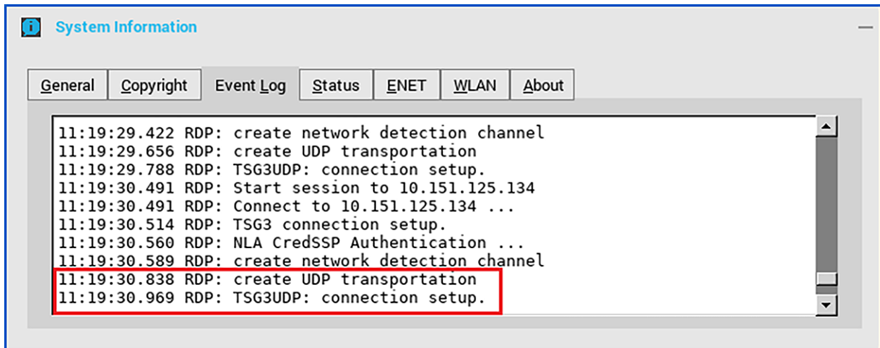
Figure 27. Event log
