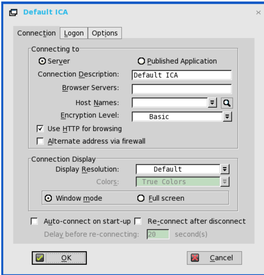
Figure 14. Default ICA
