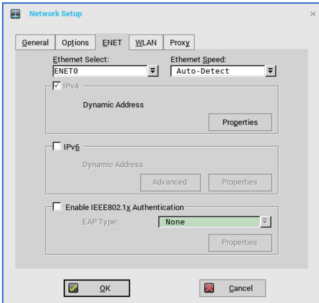
Figure 7. ENET tab
