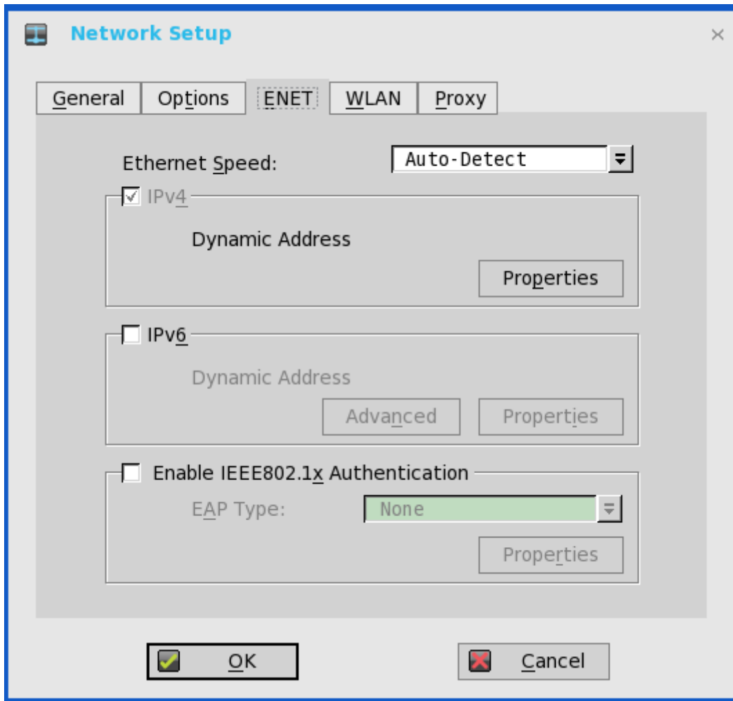
Figure 6. ENET tab
