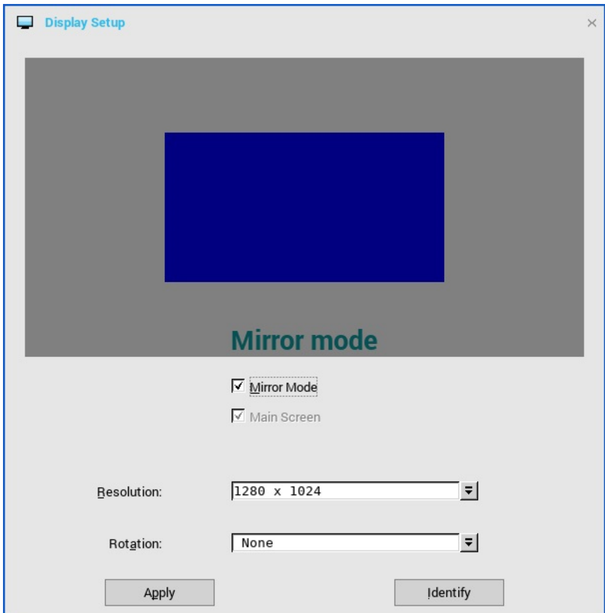
Figure 33. Display settings
