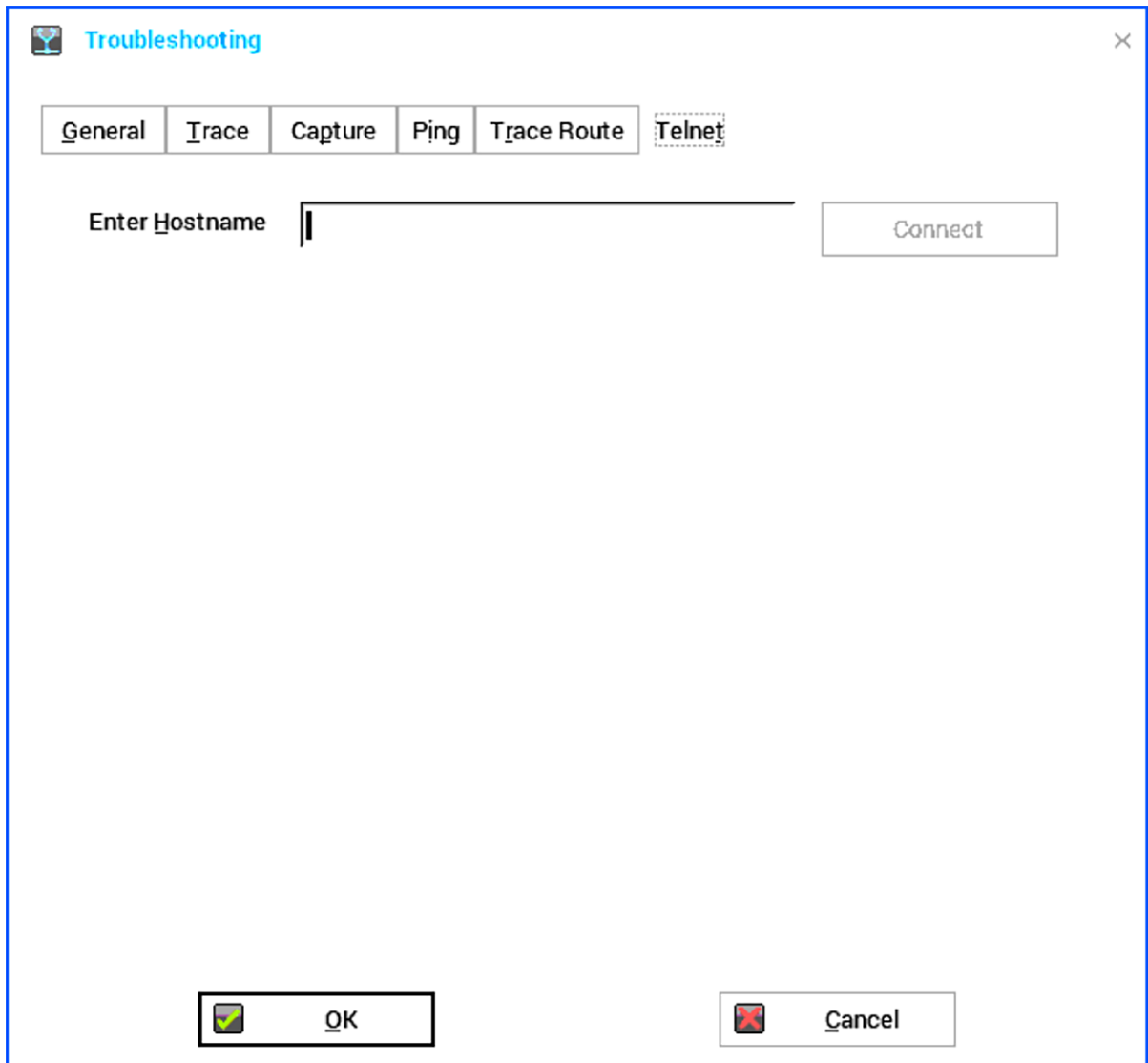
Figure 43. Telnet
