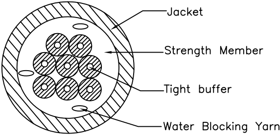
Cable Section (SCALE 5/1)
