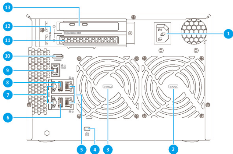
TVS-672XT
