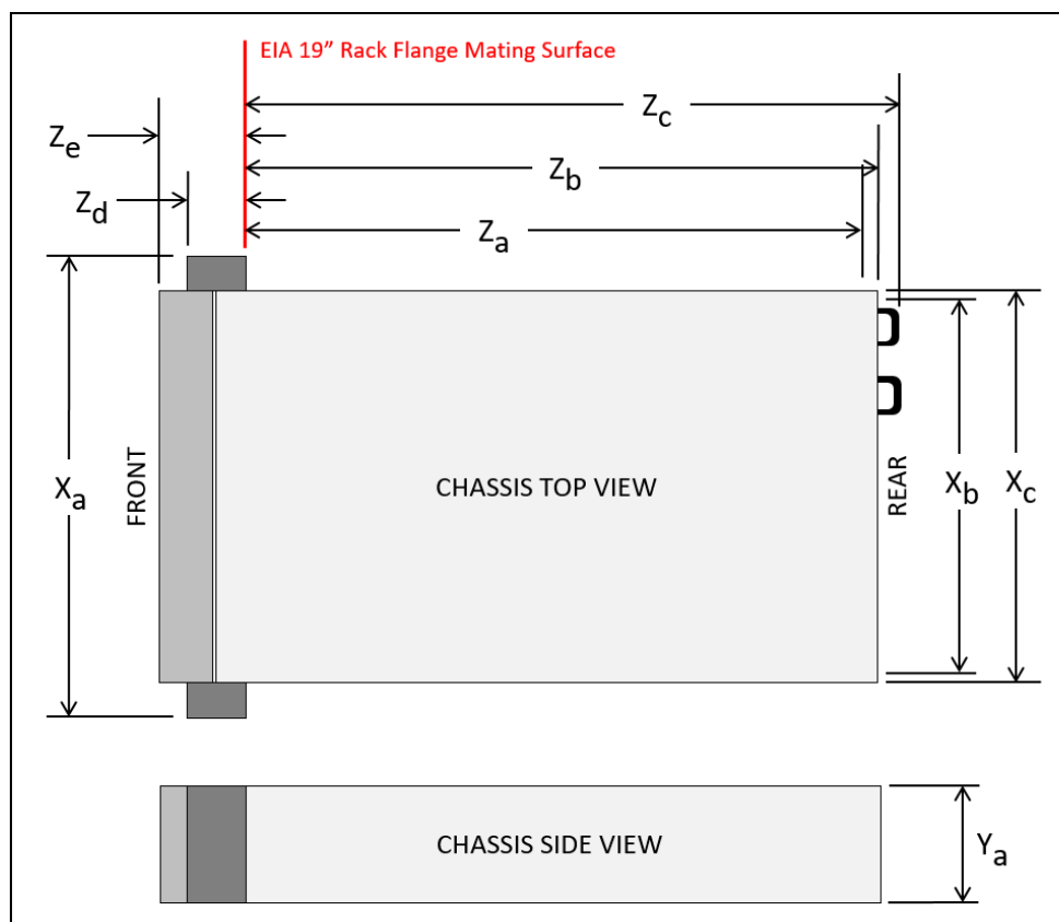
Figure 15. Server dimensions
