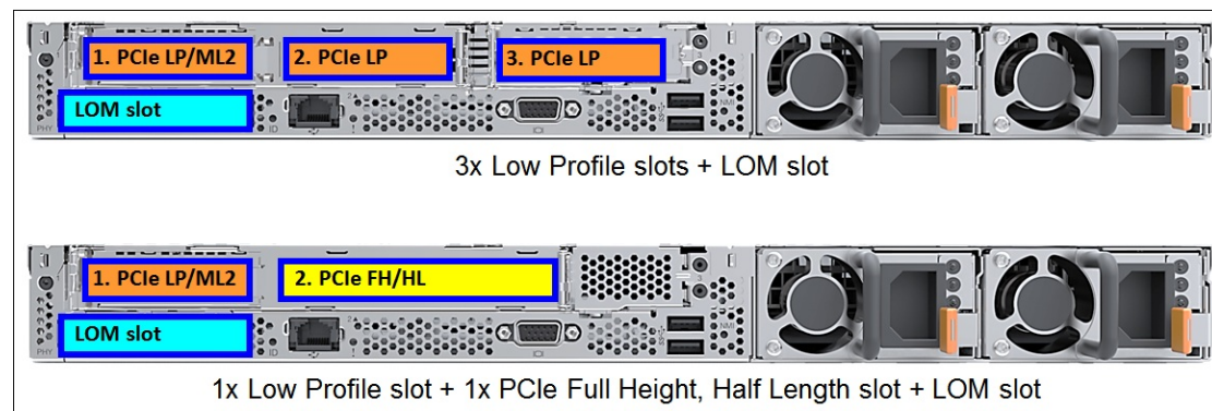
Figure 8. Slot locations
