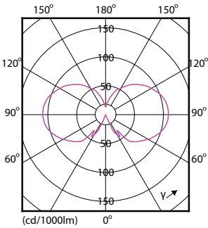
LEDbulb 100W E27 827 CL A67
