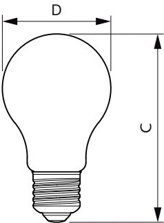
A70 230V 11-100W 1521lm 4000K E27 ND
