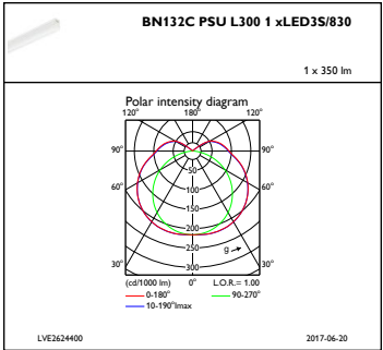
IFPC1_BN132CPSUL3001xLED3S830
