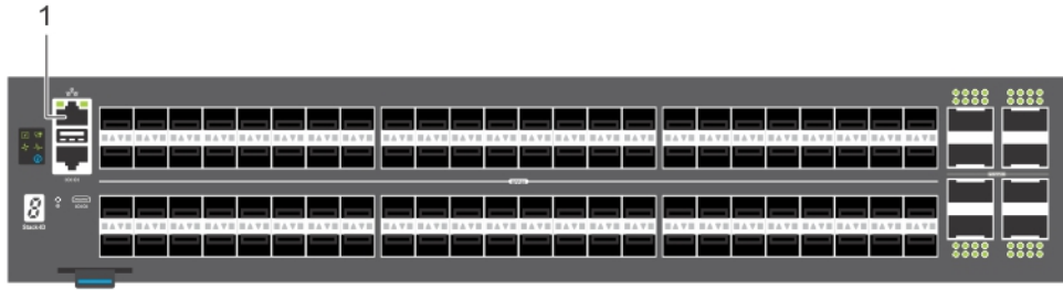
Figure 30. S5296F-ON switch management ports
