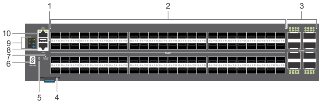
Figure 4. S5296F-ON switch I/O-side view
