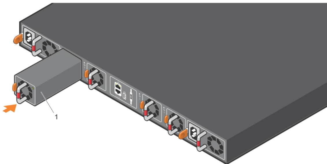
Figure 27. S5232F-ON or S5248F-ON switch fan module installation
