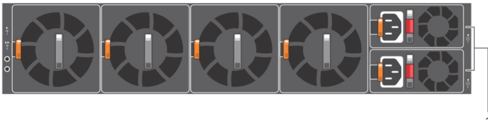
Figure 21. S5296F-ON PSUs
