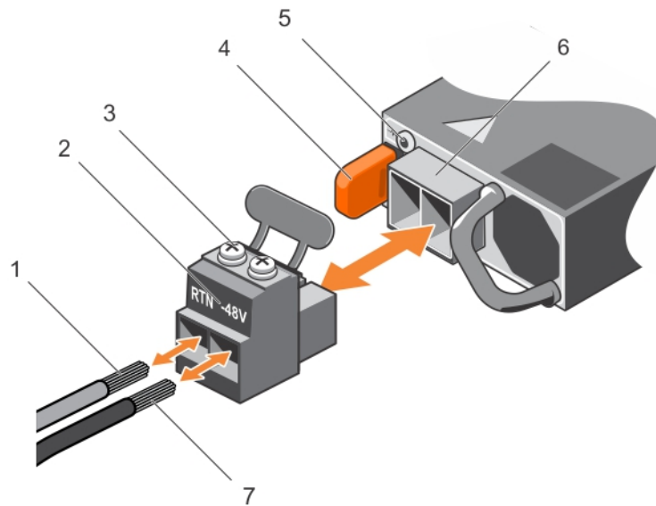
Figure 24. DC power connector and wiring block
