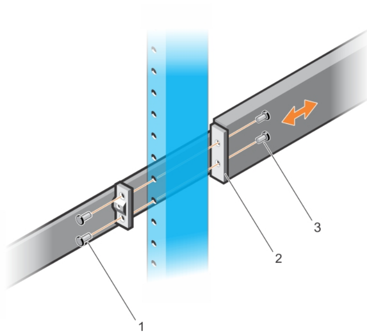
Figure 15. Two-post center-mount threaded round-hole installation
