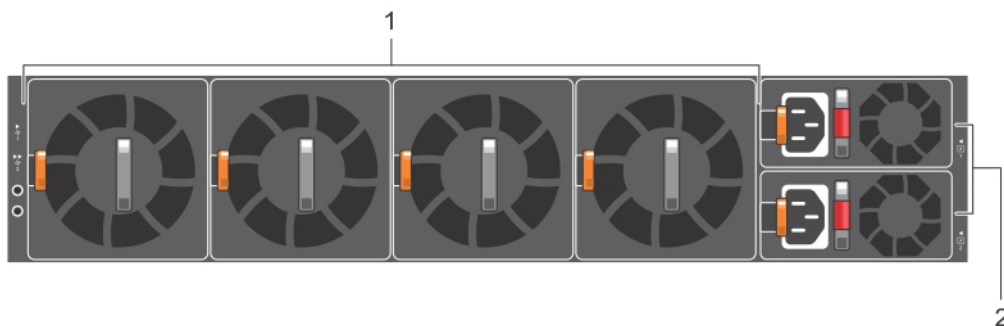
Figure 6. S5296F-ON switch PSU-side view
