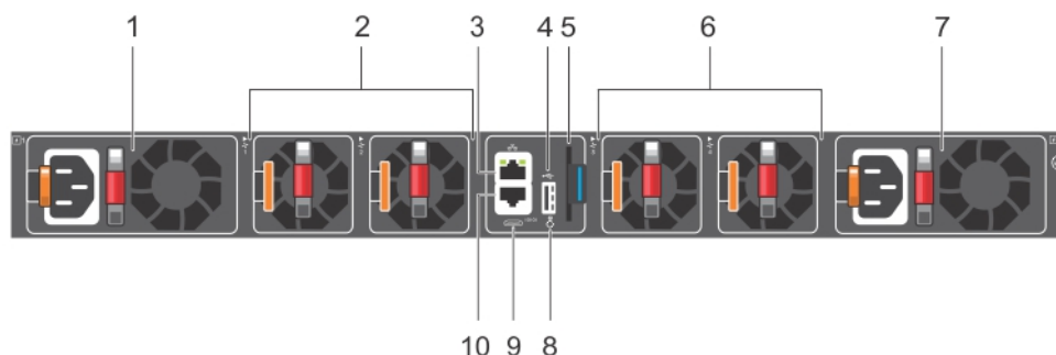
Figure 5. S5232F-ON or S5248F-ON switch PSU-side view
