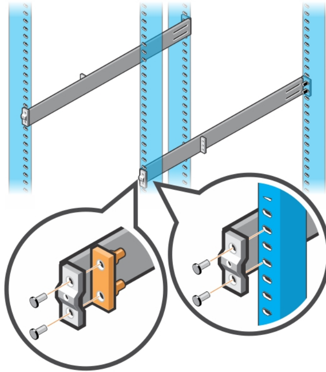
Figure 16. Four-post threaded round-hole installation
