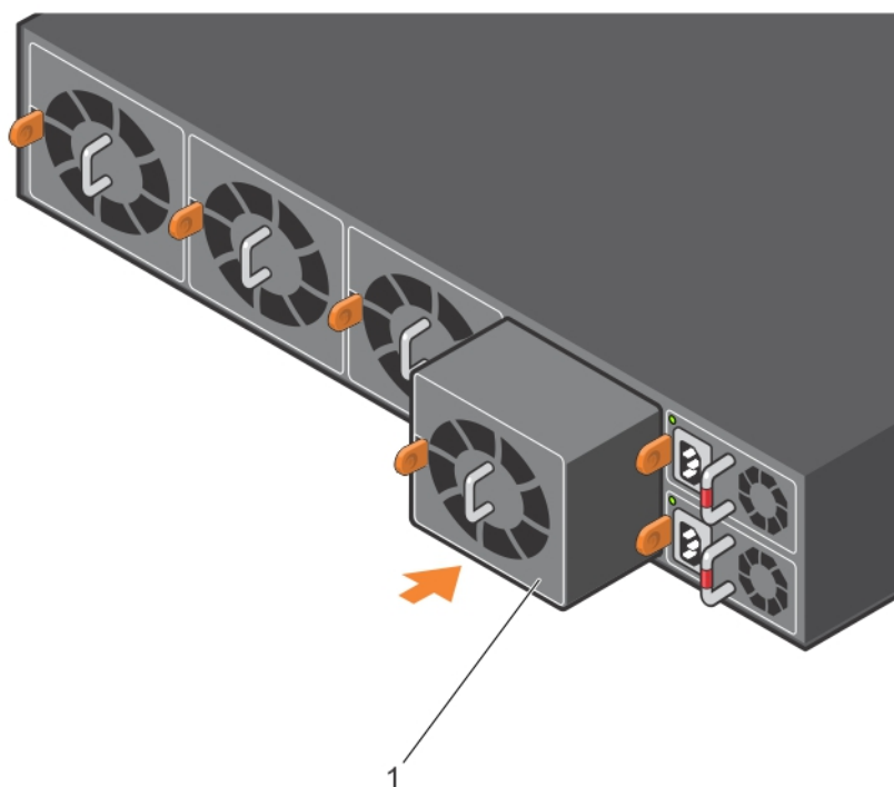
Figure 28. S5296F-ON switch fan module installation
