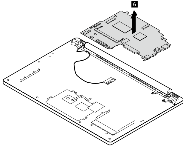
Figure 10. Removal steps of system board (continued)
