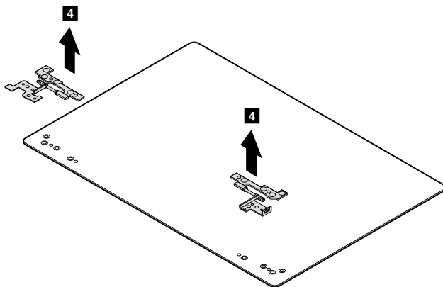
Figure 12. Removal steps of integrated camera, antenna assembly and LCD hinges (continued)
