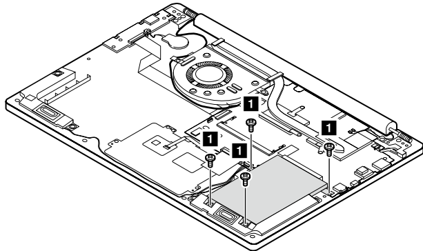
Figure 5. Removal steps of hard disk drive
