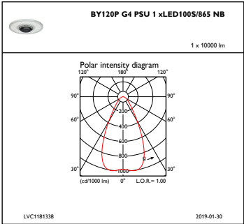
IFPC1_BY120PG4PSU1xLED100S865NB
