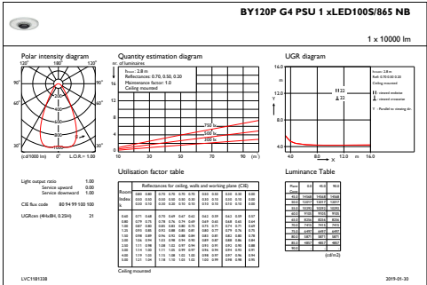
IFGU1_BY120PG4PSU1xLED100S865NB
