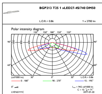
OFPC1_BGP213T251xLED27-4S740DM50
