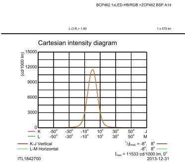
OFCC1_BCP462 1xLED-HBRGB +ZCP462 BSP A14.EPS
