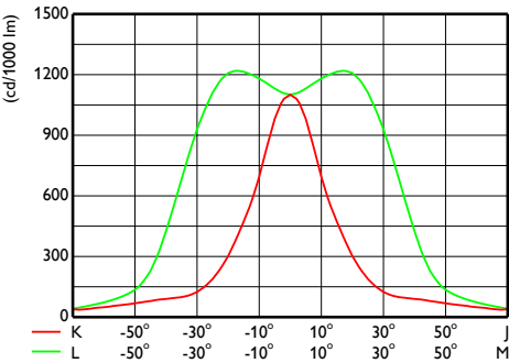
OFCS1_BVP650T251xLED340-4S740S
