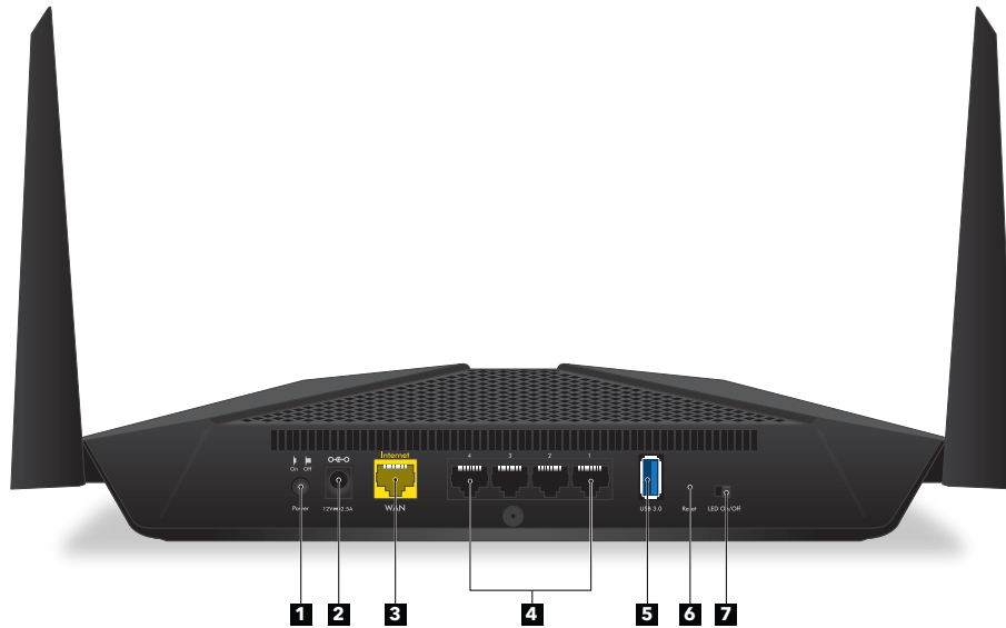
Figure 3. Rear panel
