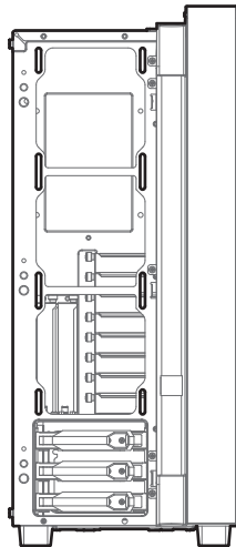
Front: Supports 120mm fan×3 or 120/240mm Radiator or 360mm Radiator(Remove HDD cage)
