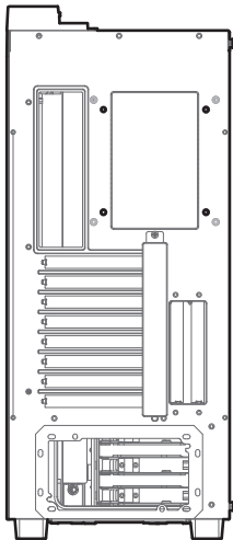
Rear: Supports 120mm fan×1 or 140mm fan×1 or 120/140mm Radiator
