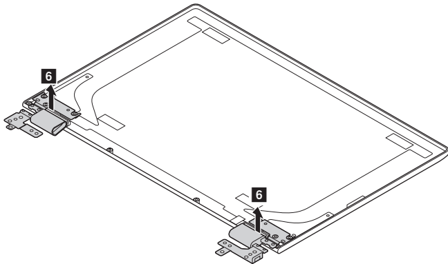
Figure 11. Removal steps of LCD unit (continued)
