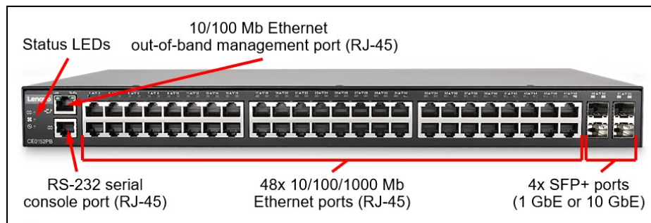
Figure 2. Front panel of the CE0152PB switch
