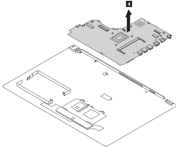
Figure 11. Removal steps of system board (continued)
