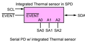
Serial PD w/ integrated Thermal sensor
