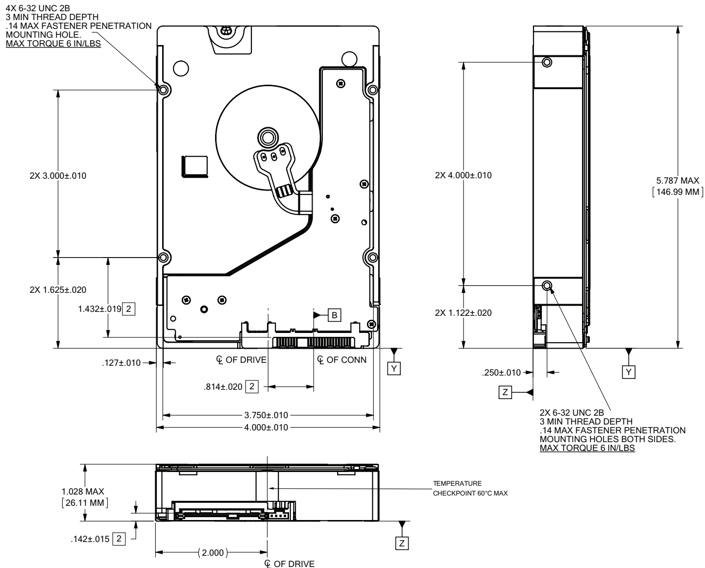
Figure 5. Mounting configuration dimensions (6TB models)
